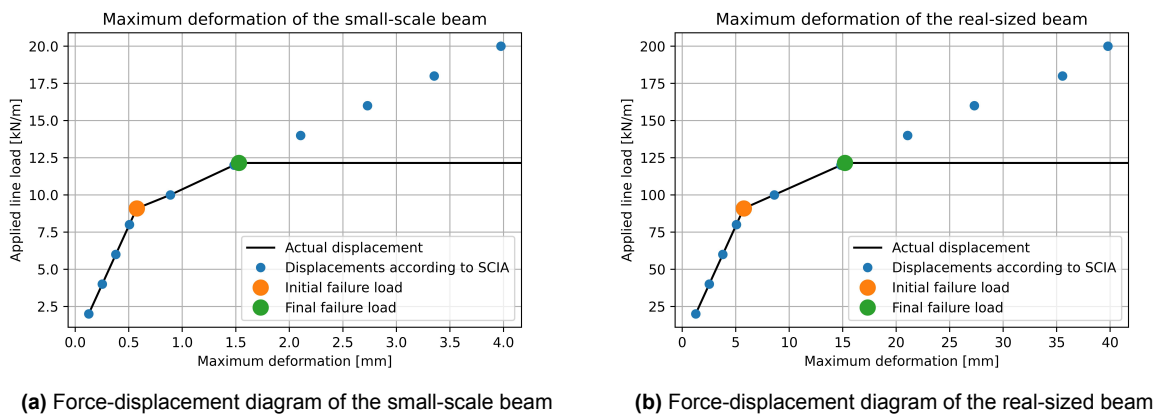
Figure 5.10: Force displacement diagram for the statically indeterminate beams. The structure fails when the final final failure load is reached
