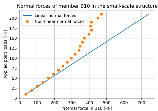
(a) Normal forces in member B10 of the small-scale structure.
