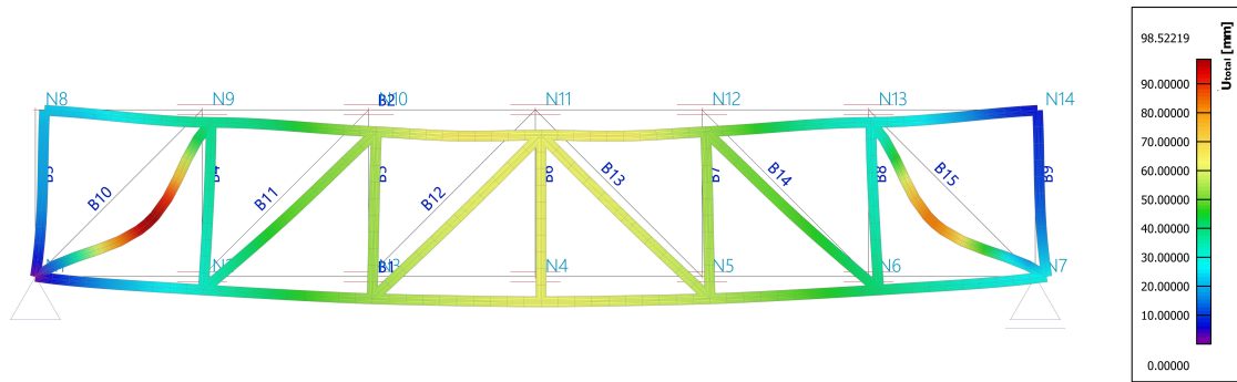
Figure 4.10: Non-linear displacement of the real-sized truss when subjected to a load of 800 kN .
