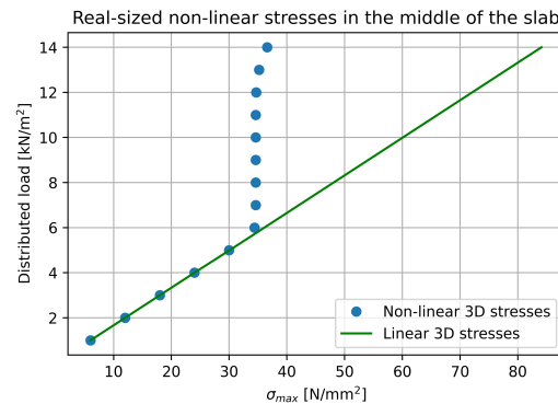
(b) Distributed load vs non-linear 3D stresses in the real-sized structure.
