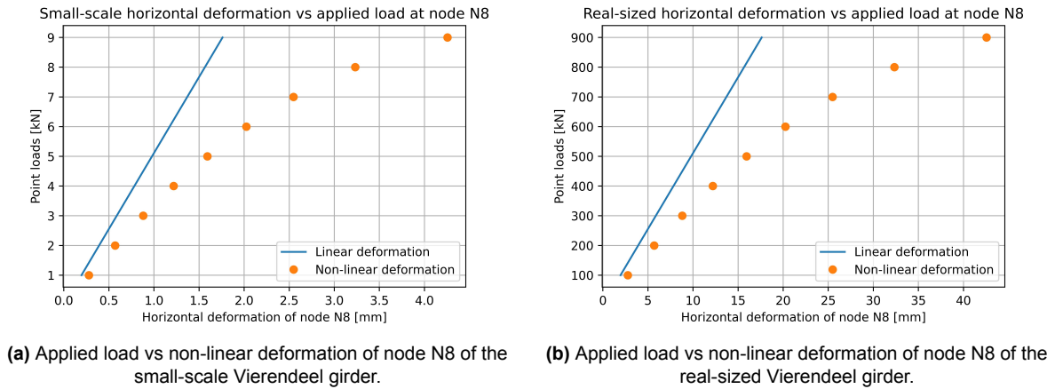
Figure 6.8: Non-linear displacement of node N8 of both the small-scale and real-sized Vierendeel girders. The applied point loads range from 1 kN to 9 kN and 100 kN to 900 kN .
