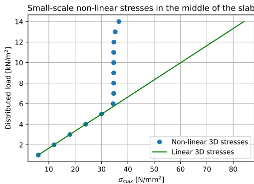
(a) Distributed load vs non-linear 3D stresses in the small-scale structure.
