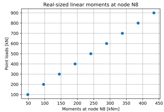
(b) Applied load vs linear moment of node N8 of the real-sized Vierendeel girder.
