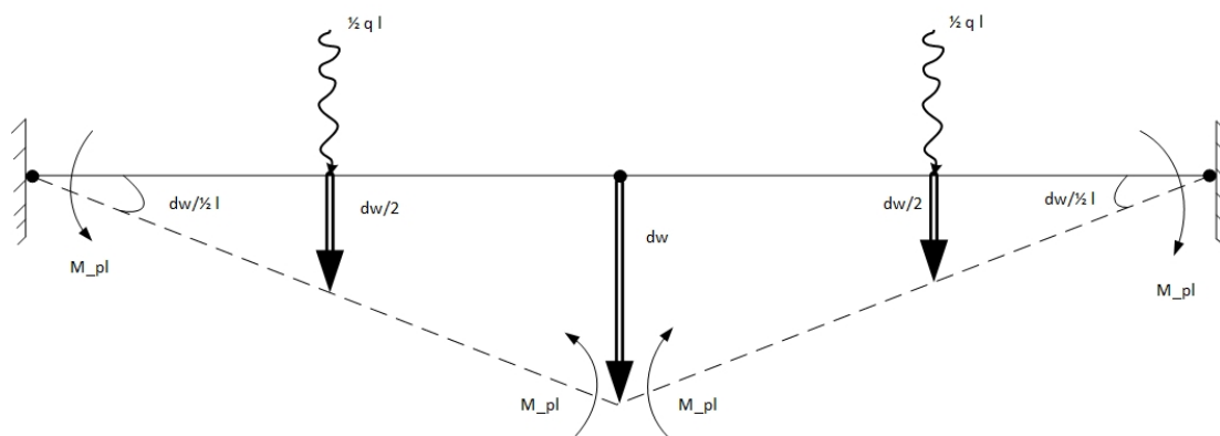
Figure C.2: Virtual work model for the statically indeterminate beam.
