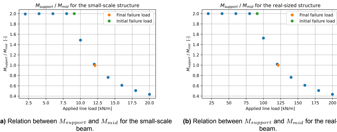
Figure 5.9: Relation between M_{support} and M_{mid} for both structures when subjected to the physical non-linear calculation. The initial factor is 2, but this changes as the applied load increases.
