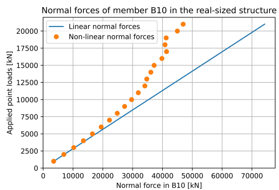
(b) Normal forces in member B10 of the real-sized structure.
