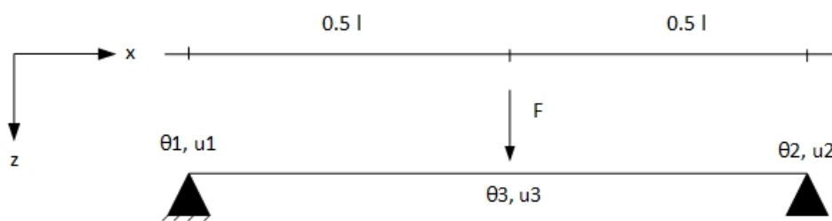
Figure 2.1: A simply supported beam subjected to a force at midspan. An example of finite element analysis is shown using this structure.
