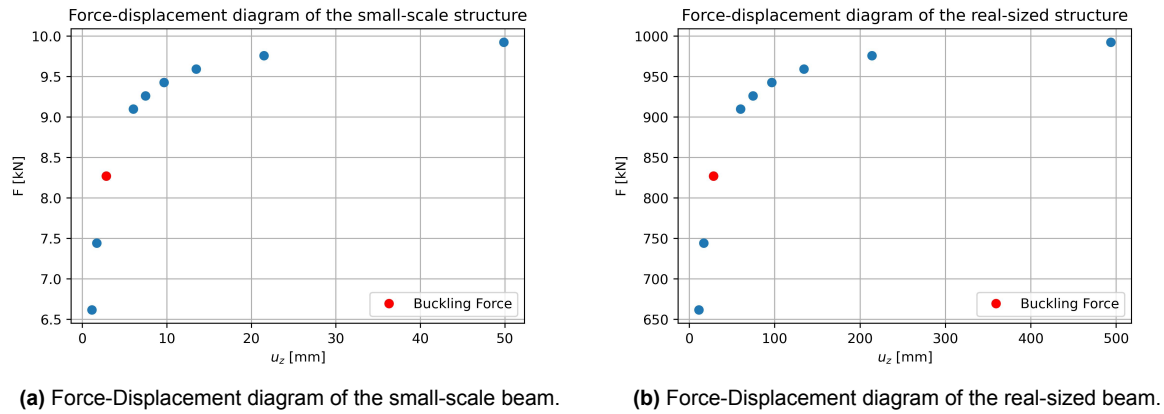
Figure 5.2: Force-displacement diagram for both the small-scale beam 5.2a and the real-sized beam 5.2b. The red dot shows the buckling force and the corresponding displacement. All data was retrieved from a non-linear SCIA Engineer calculation.
