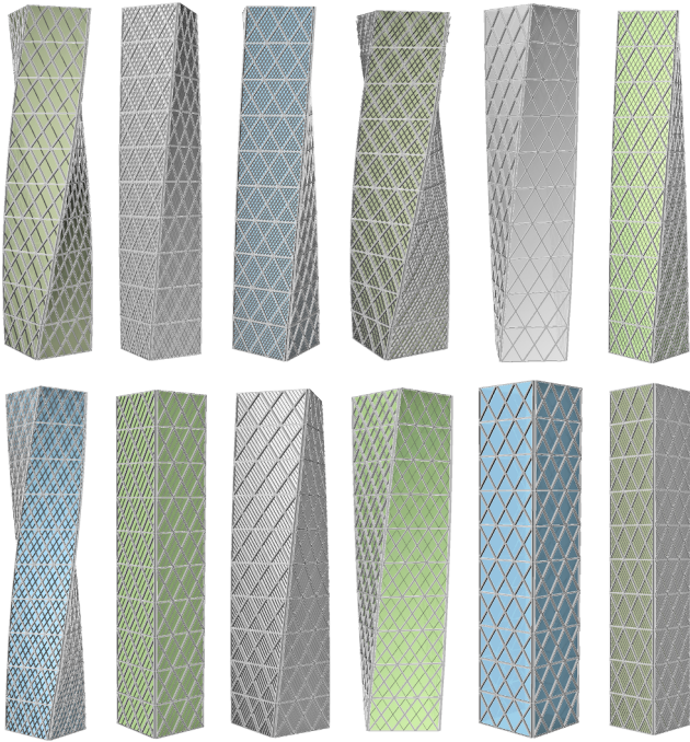
Fig. 10. Typical diagrid high-rise examples.
