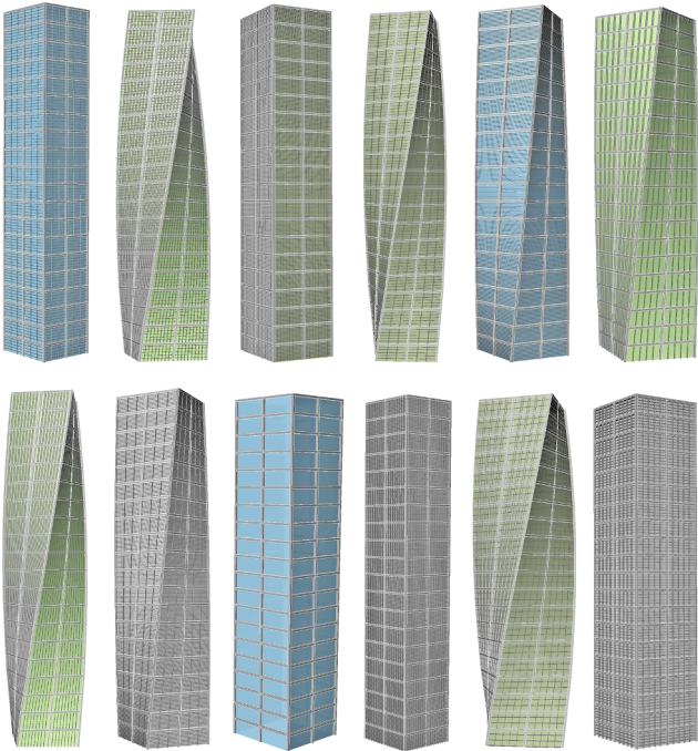
Fig. 9. Typical quad-grid high-rise examples.
