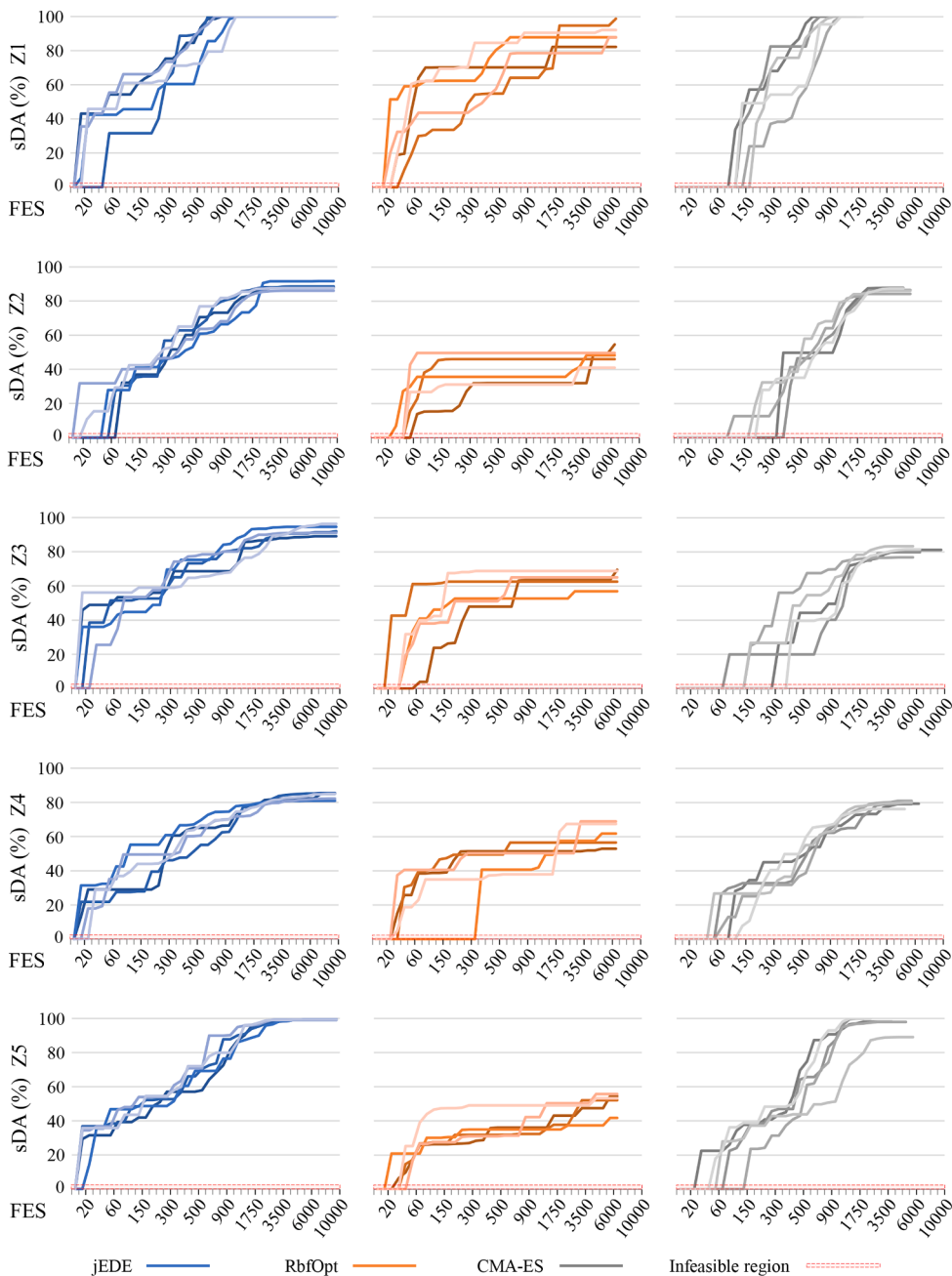
Appendix B1. Quad-grid convergence graphs for all replications from Z1 to Z5
