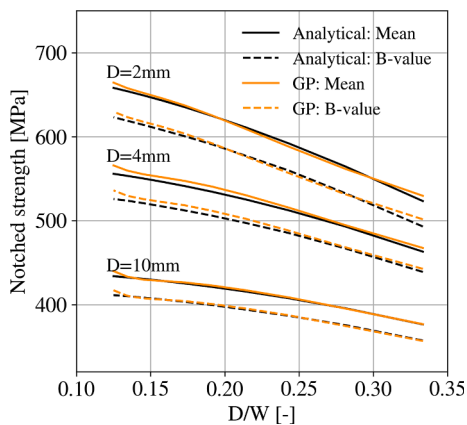
Fig. 17. Design chart for diameter-to-width ratio, 1/8 < D/W < 1/3 and hole diameters D = 2, 4, 10 mm for an IM7/852 [45/-45/20/-20] DD laminate obtained using the analytical framework and the Gaussian Processes model.
