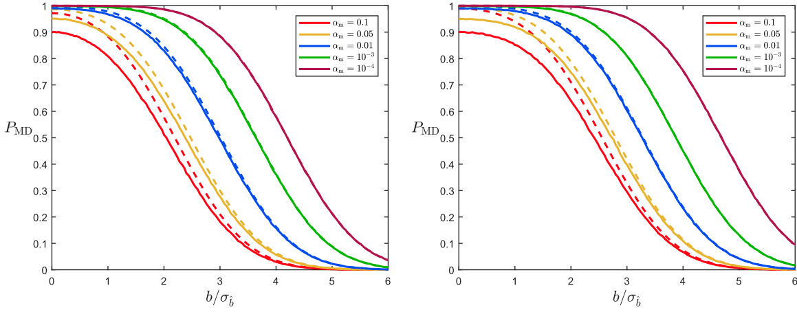
2 P_{MD_m} (full line) as a function of the normalised bias-size b/\sigma_{\hat{b}} , for different values of \alpha_m , in comparison with the upper bound P_{MD_1} (dashed lines). For the model A = [1, \dots, 1]^T \in \mathbb{R}^m and D(y) = I_m with on the left the case m=4 ( \sigma_{\hat{b}} = 1.155 m) and on the right the case m=10 ( \sigma_{\hat{b}} = 1.054 m)
