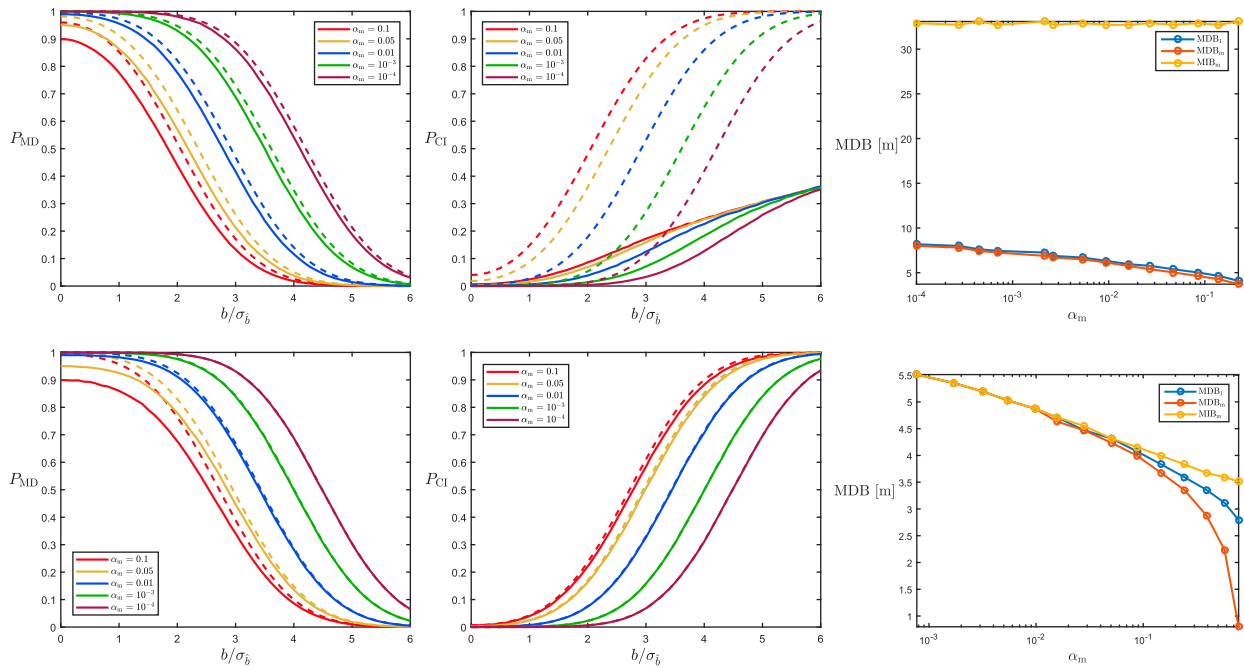
9 GNSS single point positioning. On the left, P_{MDm} (full) and P_{MD1} (dashed), and in the middle, P_{CI_m} (full) and P_{CI1} (dashed), as functions of the normalised bias b/\sigma_b , for different values of \alpha_m . At the right, MDBs and MIB as functions of \alpha_m for \gamma = 0.8 . Top row, weak GPS-only case of Fig. 8 at left, with outlier in PRN 5 ( \sigma_b = 1.69 m); bottom row, strong GPS+Galileo case of Fig. 8 at right, with outlier in PRN 12 ( \sigma_b = 1.14 m)
