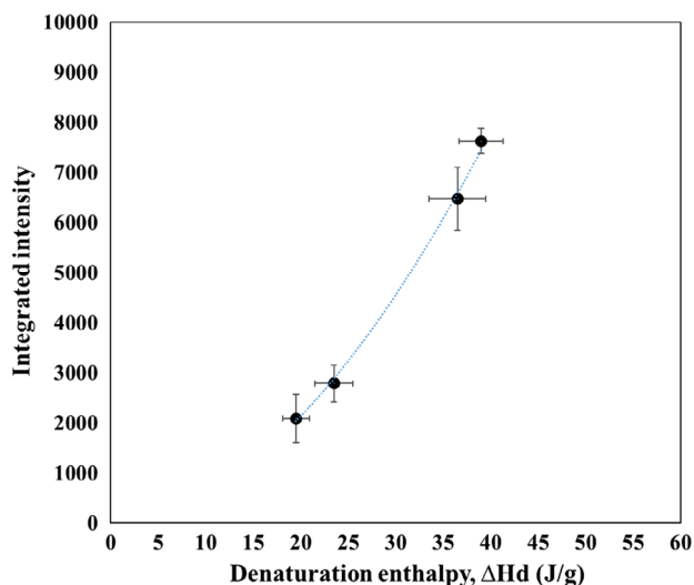
Figure 6. Correlation between integrated intensity of XRD peak at 2\theta \approx 8^\circ and enthalpy of denaturation of triple-helix coil obtained from DSC.
