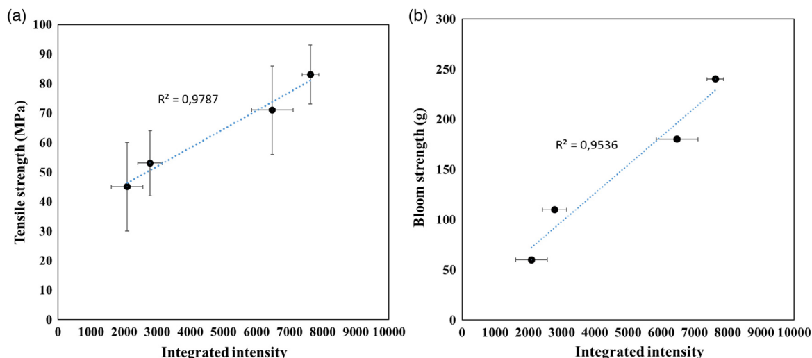
Figure 7. a) Tensile strength plotted versus integrated intensity of the XRD patterns at 2\theta \approx 8^\circ with a linear least squares regression; b) Bloom strength plotted versus integrated intensity with a linear least squares regression.
