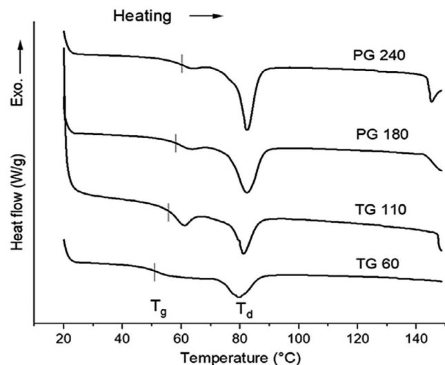
Figure 1. First heating thermograms of gelatin films obtained by DSC.
