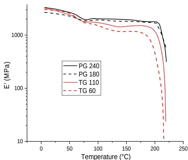
Figure 4. Storage modulus–temperature curves of different gelatin films obtained from DMA.
