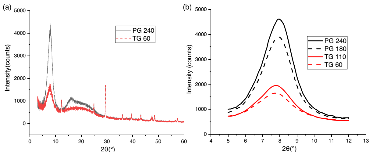
Figure 2. a) Comparative XRD patterns of PG 240 and TG 60 over a wide range of 2\theta ( 3^{\circ} – 60^{\circ} ); b) comparative XRD patterns of gelatins at 2\theta \approx 8^{\circ} .
