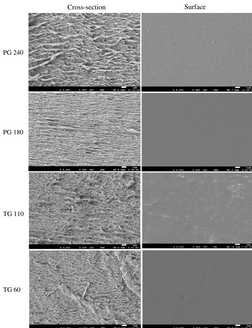
Figure 5. SEM micrographs of cut cross sections and surfaces of different gelatin films.
