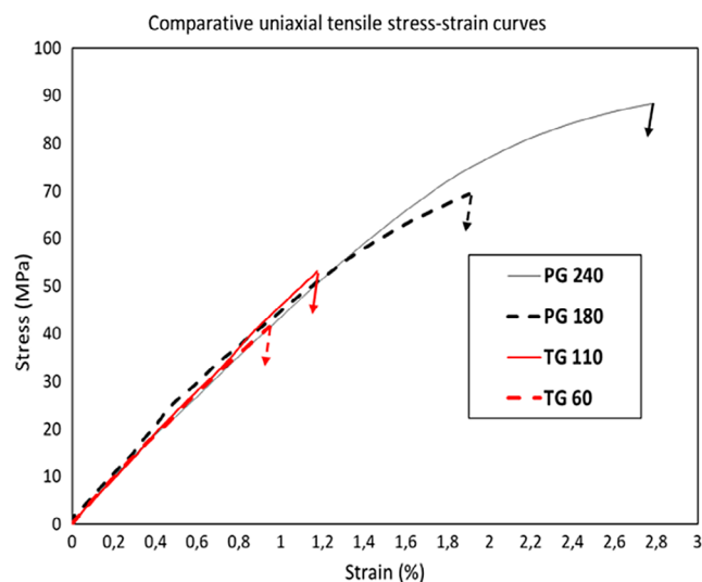
Figure 3. Uniaxial tensile stress–strain curves of gelatin films with different Bloom values, at standard environmental conditions.
