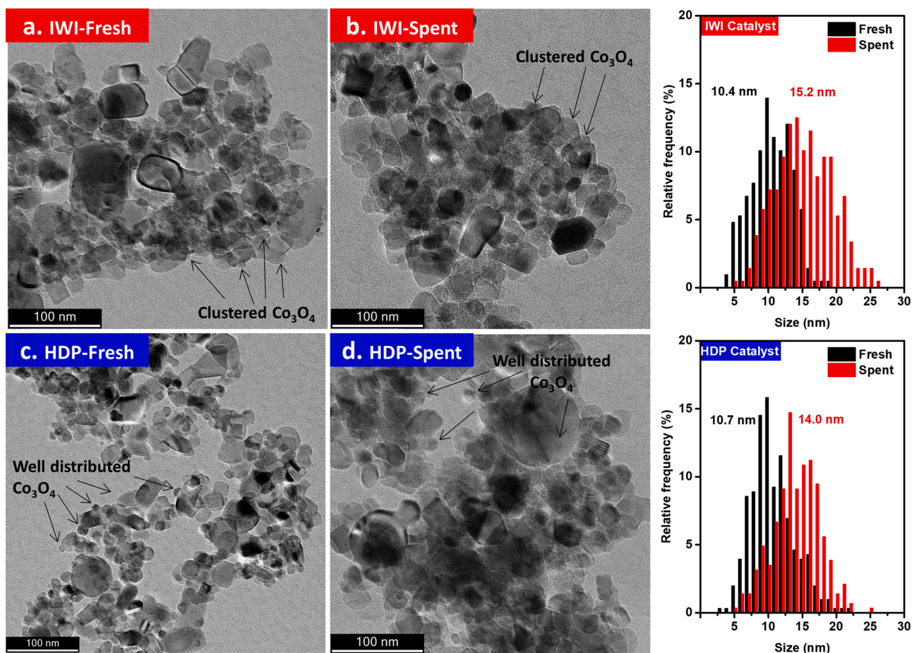
Fig. 1. TEM micrographs and histograms for cobalt particle size analysis of IWI and HDP catalysts.
