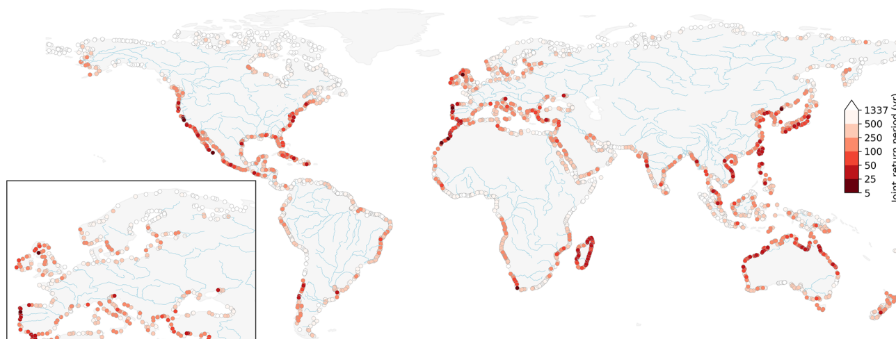
Figure 6. Probability of a co-occurring annual maxima in a given year P_F presented as the return period in years exceeding the marginal 5-year return periods of discharge and of storm surge. Major rivers are shown in light blue.
