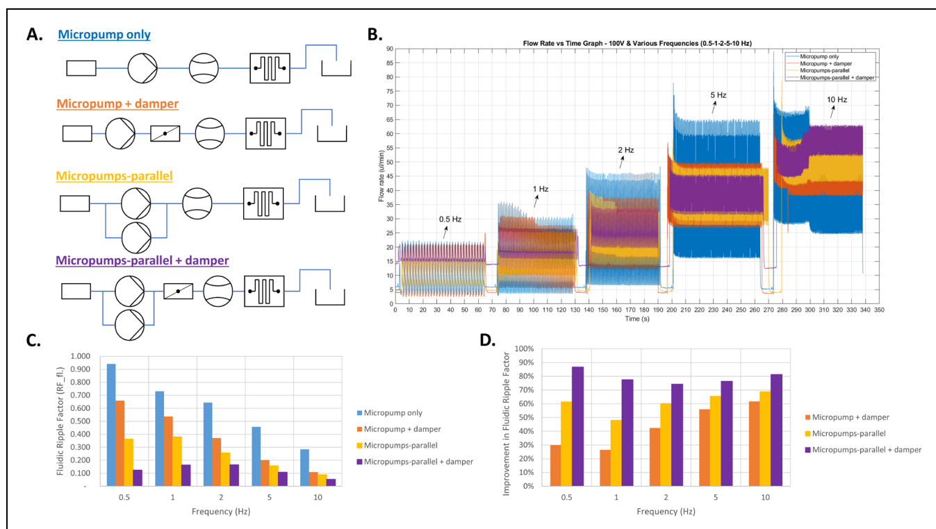
Figure 1: Comparison of tested configurations for minimizing flow ripples in piezoelectric micropumps. A. Schematics used for calculating RF_{FL} values. B. Flow ripple formation at various frequencies. C. Calculated fluidic ripple factors for each configuration. D. Ripple factor improvement ratios of the configurations.
