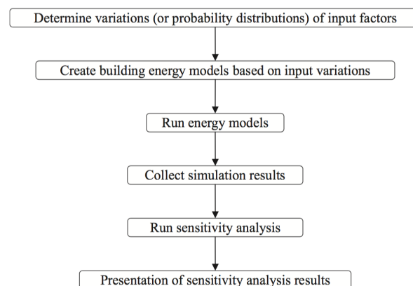
Figure 2.10: Typical workflow of sensitivity analysis in building performance analysis. Retrieved from Wei [3]
