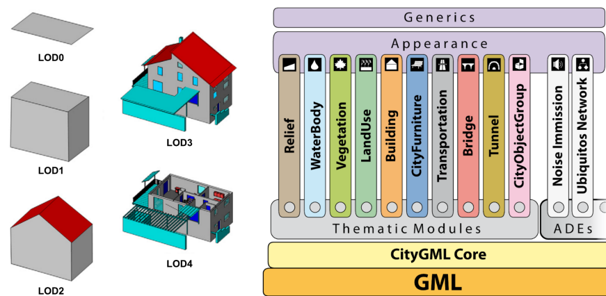
Figure 2.9: Left: Five level of detail representations in CityGML. Right: General CityGML architecture, thematic modules and application domain extensions (ADEs). Retrieved from [58, 61]
