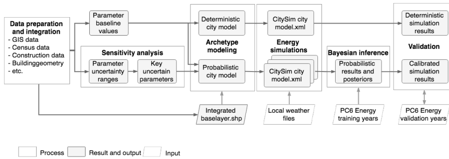
Figure 1.1: The generalized workflow followed by this research. Only key processes and results are shown. Complete breakdown of this workflow is discussed in Chapter 3
