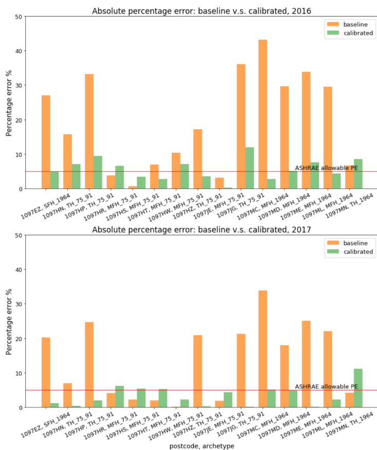
Figure 6.4: Baseline and calibrated simulation results of the partial postcodes presented in absolute percentage error. The red horizontal line indicates the ASHRAE allowable maximum percentage error (5%) of annual calibrated model.
