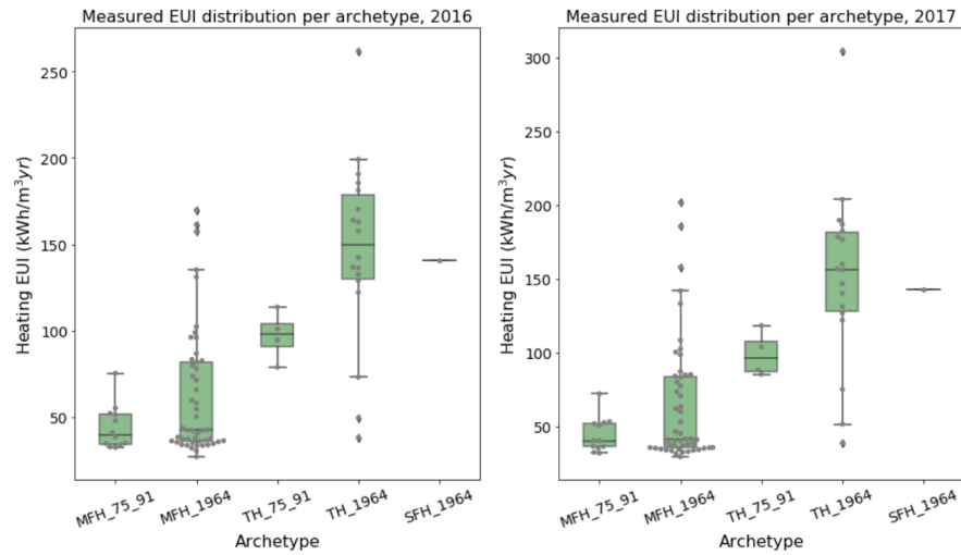
Figure 6.1: Measured postcode level EUI distribution per archetype included in the test site. 84 and 85 samples available in 2016, 2017 respectively.
