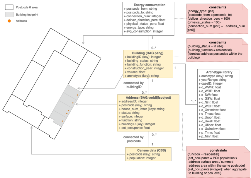
Figure 4.7: UML diagram presents the key attributes, feature constraints, and relationships of these heterogeneous datasets. The spatial resolution of each data is illustrated on the left. The integrated baselayer is integrated from the UML classes colored in yellow, and the data filtering rules are colored in red.
