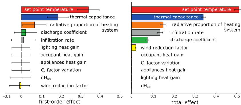
Figure 2.12: Example result of the first order and total effect of the variables conducted by Sobol method. Retrieved from Menberg et al. [66]
