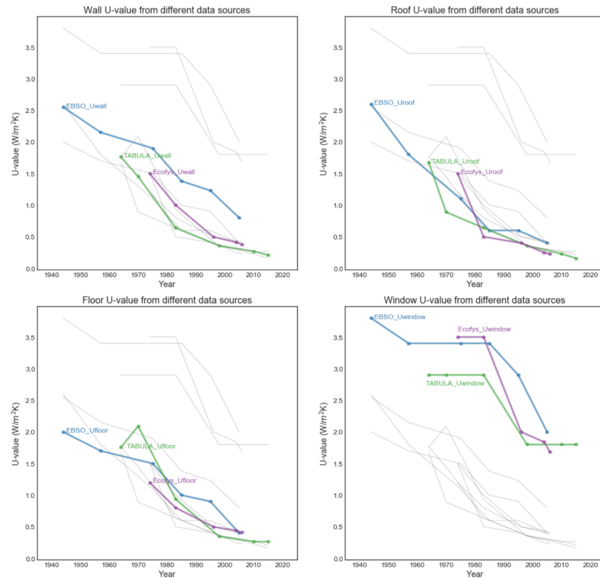
Figure 4.4: Comparison of multiple U-values of the construction materials collected from different sources
