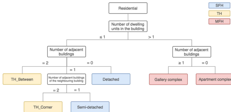
Figure 4.9: Classification rules based on topology relation and the number of address per building is implemented for the dwelling type classification.
