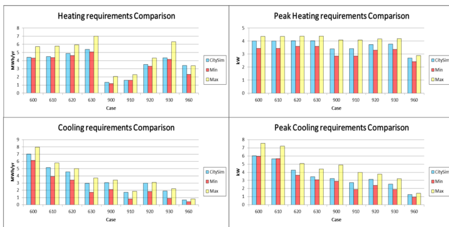
Figure 2.8: Comparative testing results of CitySim compared with reference kernels based on BESTEST for the annual heating, cooling loads, and peak heating and cooling requirements. Retrieved from Walter and Kämpf [53]
