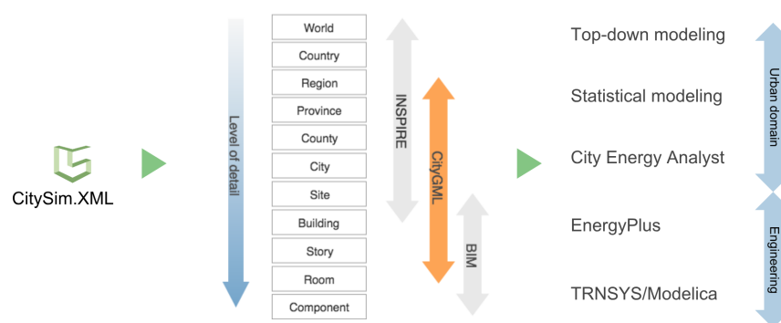
Figure 7.4: From stand-alone data model to standardized semantic data model can potentially increase data interoperability and facilitate data exchange to make multi-scale and multi-domain simulations and applications easier. Adapted from [59]
