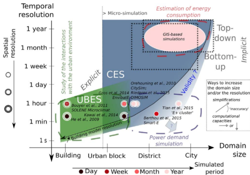
Figure 2.6: Multi-scale and multi-domain nature of energy simulation. Retrieved from Frayssinet et al. [27]
