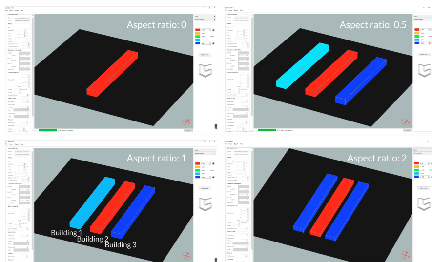
Figure 5.1: Annual heating demand results with four different aspect ratio set-ups. Heating demand from high to low is colored in red to blue.
