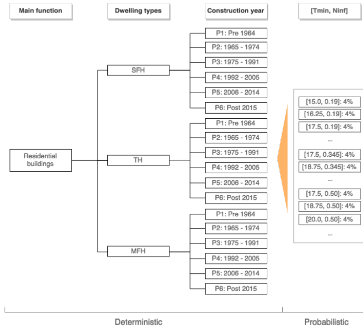
Figure 5.7: T_{min} and N_{inf} are two key uncertain parameters according to the sensitivity analysis. This information enables the modeler to expand each of the existing deterministic archetype with a probabilistic definition.
