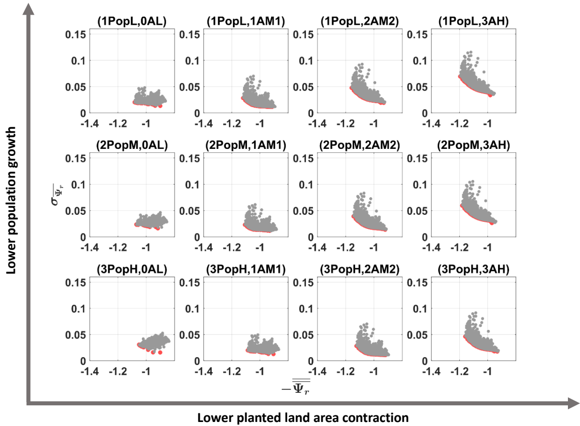
Figure 7a Food secure pareto frontiers under least optimistic climate scenario (RCP8.5, P10%). The x-axis shows the objective of minimizing the negative of average food self-sufficiency
