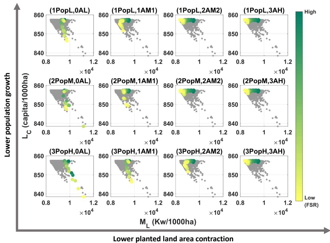
Figure 10a Trade-off between crop labor force, L_C , and land-preparing machinery power, M_L , used under least optimistic climate scenario (RCP8.5, P10%).
