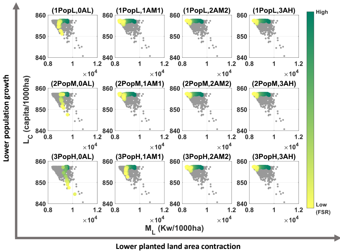
Figure 10b Trade-off between crop labor force L_C and land-preparing machinery power M_L under most optimistic climate scenario (RCP2.6, P95%)
