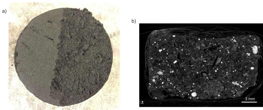
Fig. 8. Fabric of reconstituted peat sample (a) cross section image; (b) micro-CT scan. [Colour online.]
