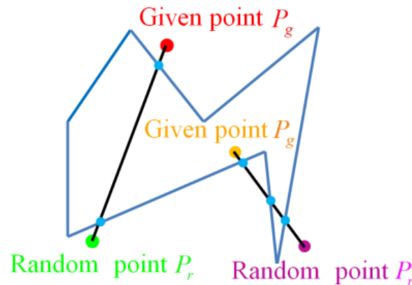
Figure 4.10: The method to judge whether a given point is inside or outside a polygon. If a given point is outside a polygon, the line between the given point and the random point has even number of intersects with the polygon. If a given point is inside a polygon, the line between the given point and the random point has odd number of intersects with the polygon.
