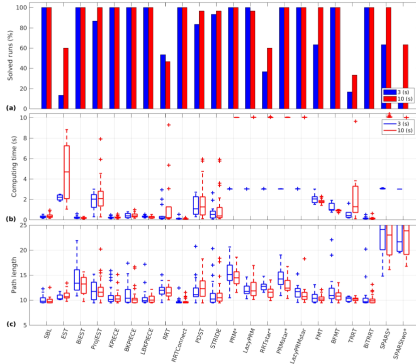
Figure 6.14: Comparison results of 23 motion planners in MoveIt! for benchmark 1.
