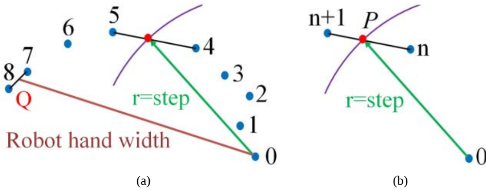
Figure 5.12: The step point searching.
