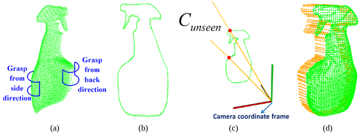
Figure 6.9: Illustration of the solution to deal with the unseen part of the target object to eliminate the grasp uncertainty.
