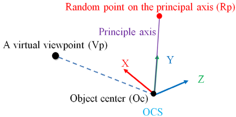
Figure 3.20: Schematic illustration of constructing a virtual object coordinate system (VOCS).
