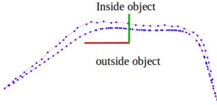
Figure 5.7: Concave hull of the projected point cloud of the concavity.
