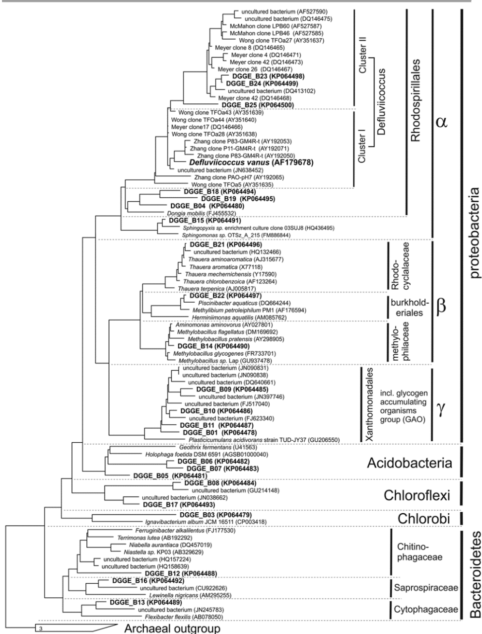
Fig. 5 - The phylogenetic tree was calculated using maximum-likelihood algorithm implemented in ARB (RAxML module). Full sequences from the SSU115-NR99 database were used for calculation together with an SSUref: bacteria filter (resulting in 1125 base pairs). DGGE bands and clones with a variable length (311-962 base pairs) were added later using parsimony algorithm. Bootstrap (250rxn) was performed but not shown. Sequences shown were deposited into Genbank under accession number KP064478 - KP064500.
