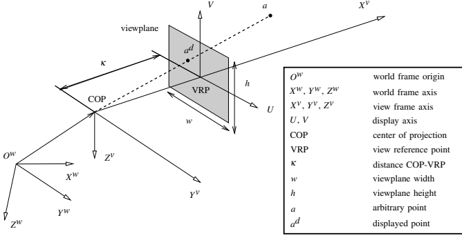
Fig. 3. The perspective projection method and its principal terminology.
