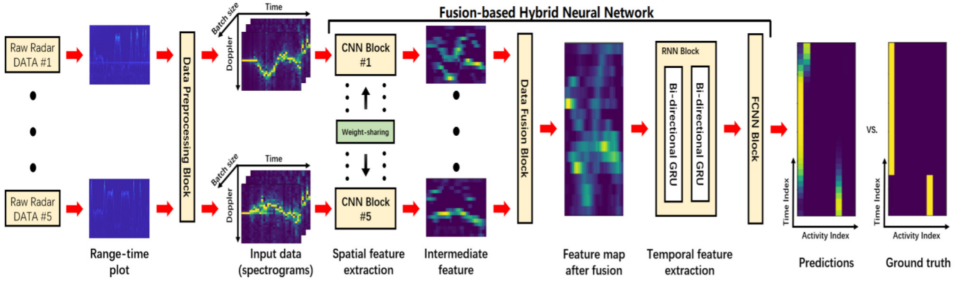
Fig. 3. Architecture overview of the proposed HAR system. On the leftmost are the raw radar inputs from five UWB radar sensors. The inputs to the CNN block are the spectrograms. The outputs of the HAR system are predictions, which provide information about the performed activities.
