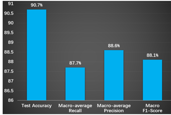
Fig. 10. Performance of the proposed classifier evaluated using accuracy and three additional metrics. All results are measured using the testing data with the L1PO method.
