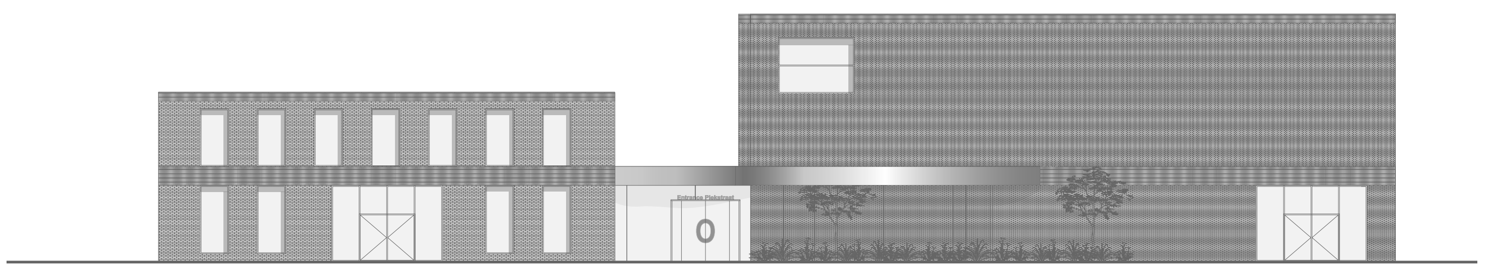
East elevation 1:200
