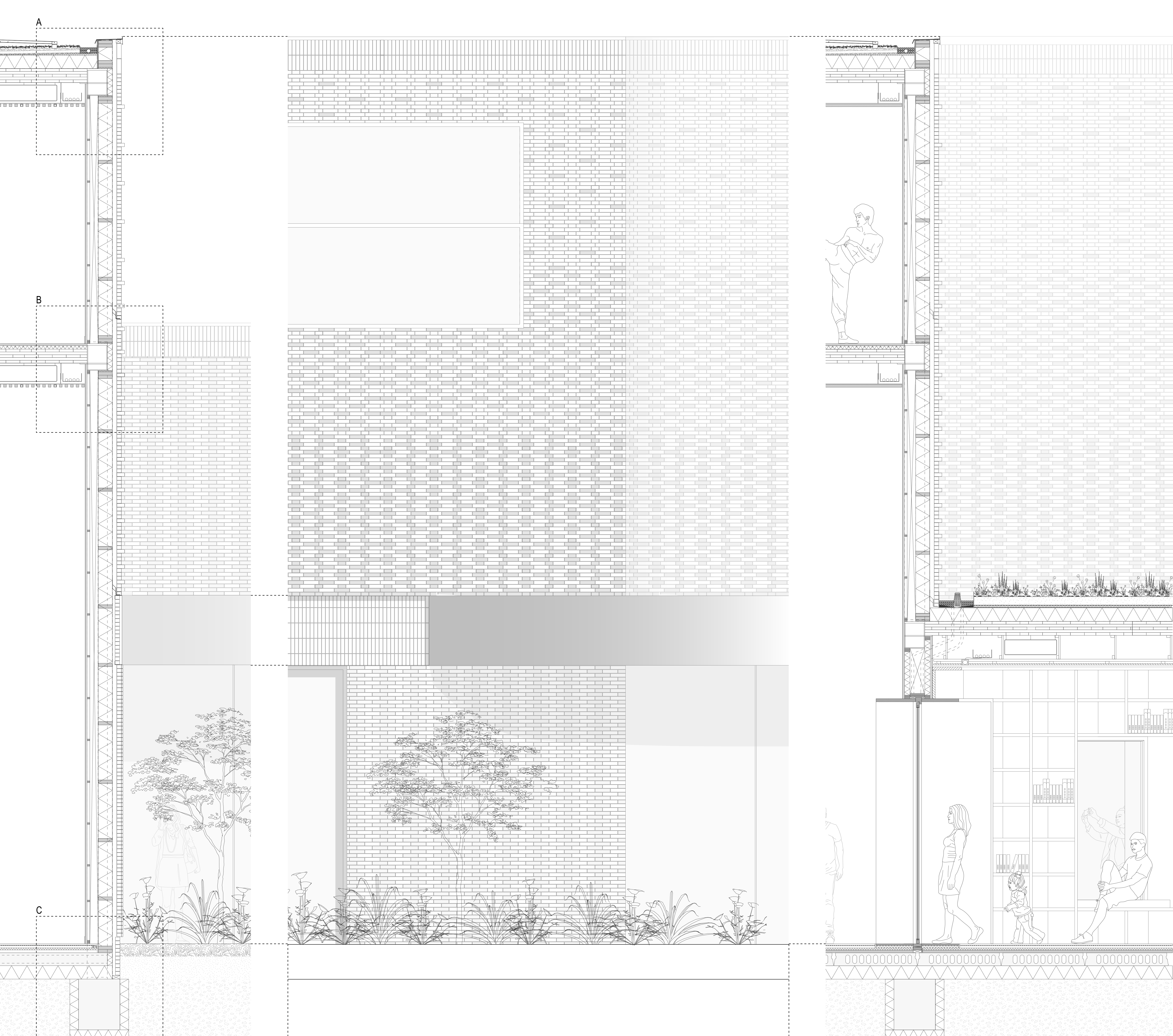
2 Brick facade fragment 1.20
