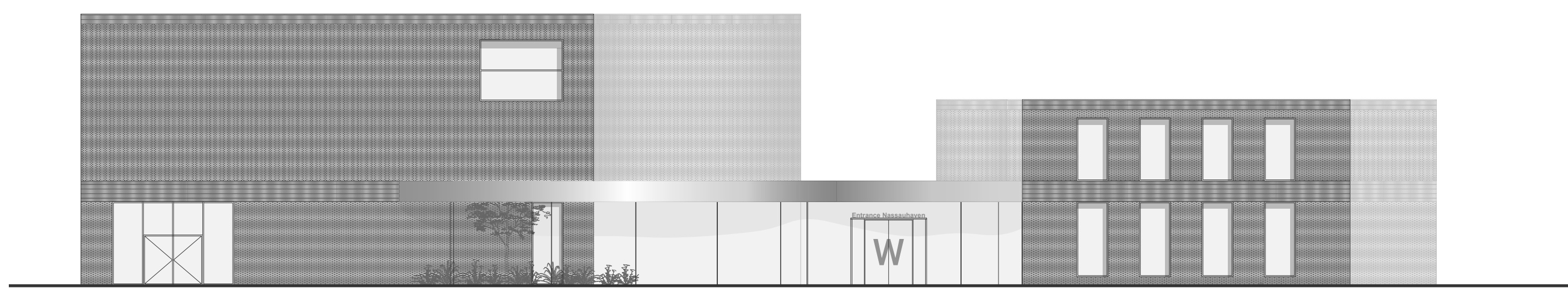
West elevation 1:200
