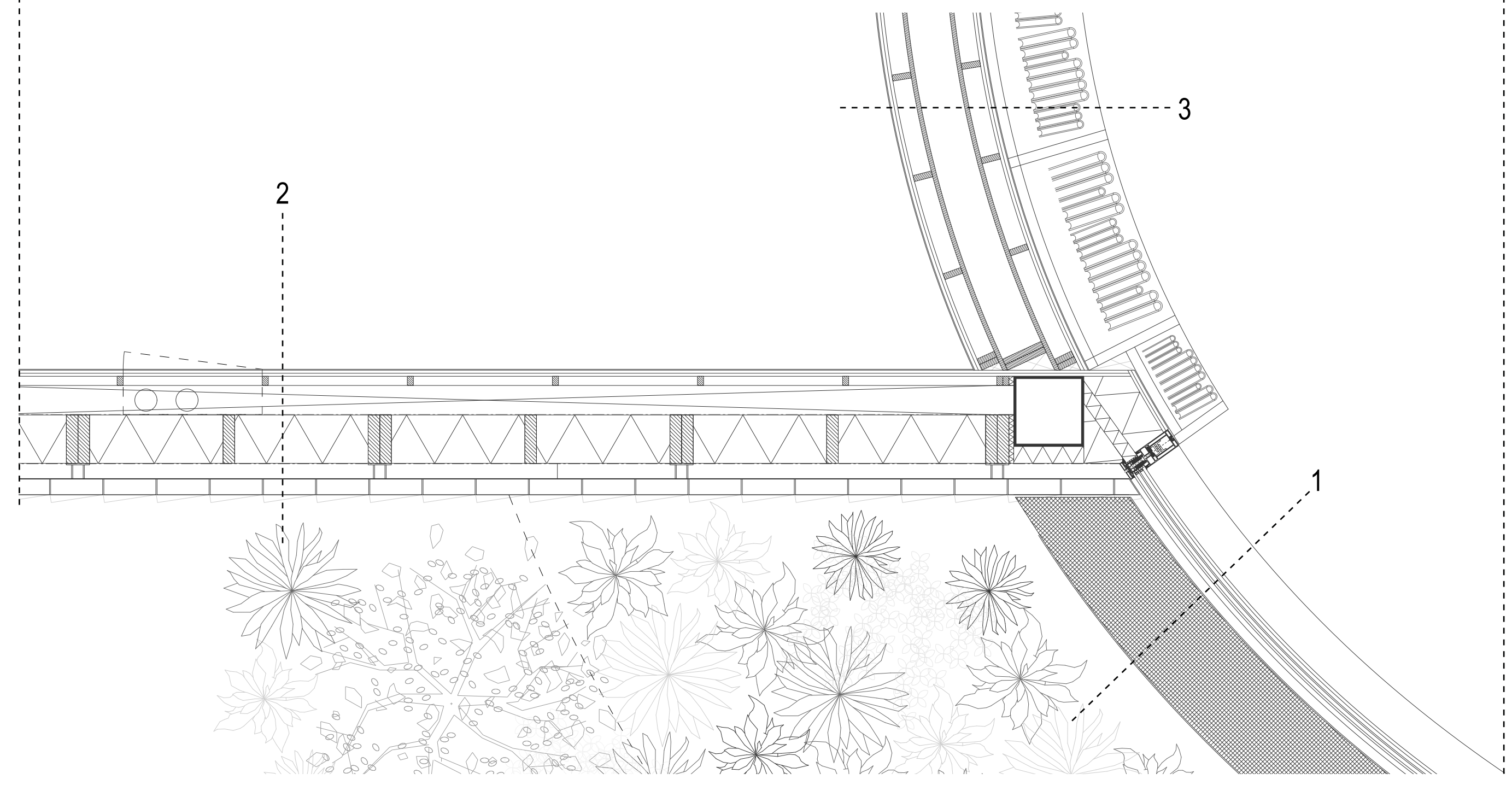
Horizontal facade fragment 1.20
