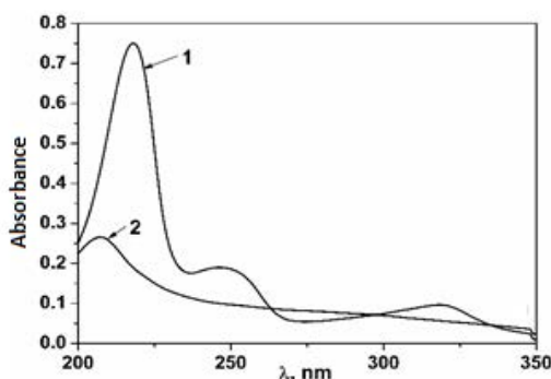
Figure 4: UV-VIS spectrum profile of PCP: 1-initial and 2-after 90 minutes of photoelectrodegradation.
