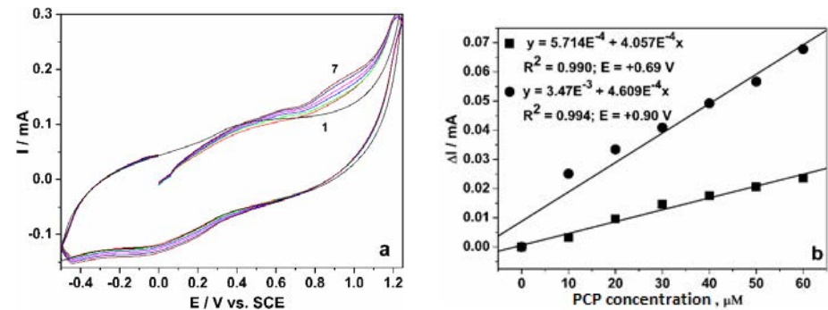
Figure 2: (a) Cyclic voltammetry recorded at TiZCNT electrode under UV irradiation in 0.1 MNa 2 SO 4 and various PCP concentrations: 1-0 μM; 2-10 μM; 3-20 μM; 4-30 μM; 5-40 μM; 6-50 μM; 7-60 μM; potential range: -0.5 V → +1.25 V vs. SCE; scan rate: 0.05 V·s -1 ; (b) Linear dependence of anodic peak current versus PCP concentrations (E = +0.69 V și E = +0.90 V vs. SCE).
