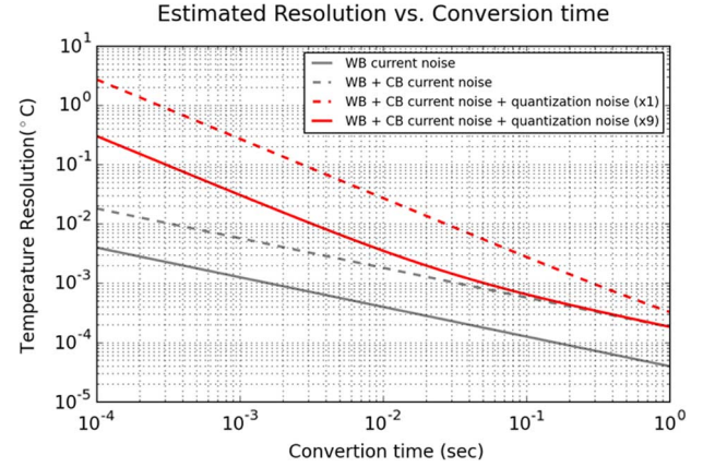
Fig. 5. Estimated temperature resolution of the WB-based temperature sensor with FLL-based readout method.
