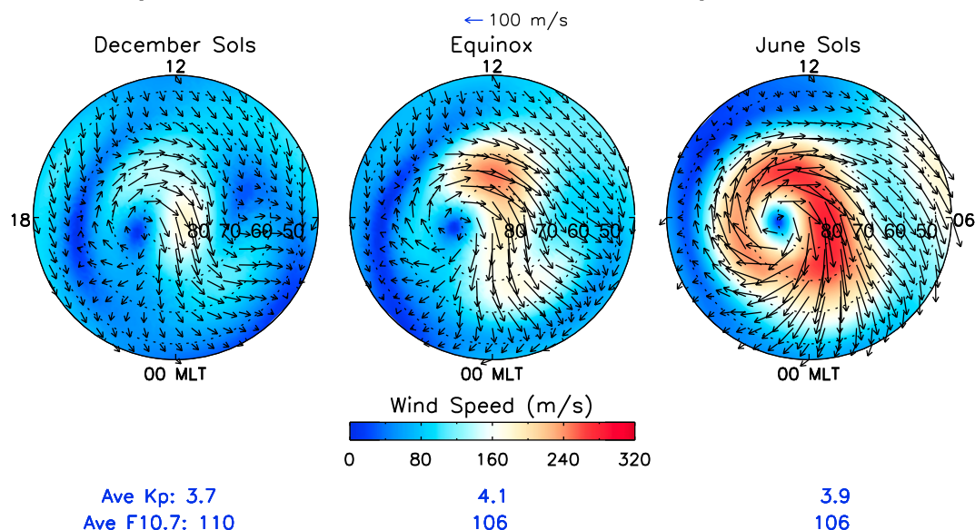
Figure 3. Polar plots of active-time northern high-latitude F region assimilated neutral vector winds as a function of magnetic latitude and magnetic local time (looking down on the geomagnetic North Pole). The background color represents the wind speed. Average K_p and F_{10.7} of the data for each season are listed at bottom of each panel. The outer boundary of each panel is located at 45^\circ\text{N} MLAT.
