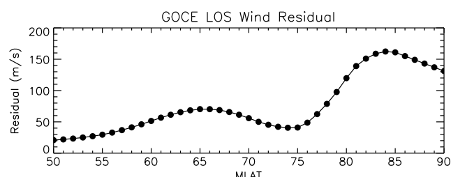
Figure 2. Systematic difference between quiet time GOCE cross-track winds and quiet time model climatology without GOCE as a function of magnetic latitude, averaged over all magnetic local times. This quantification of the bias was applied to GOCE data as a correction profile to correct the apparent bias in the GOCE winds.
