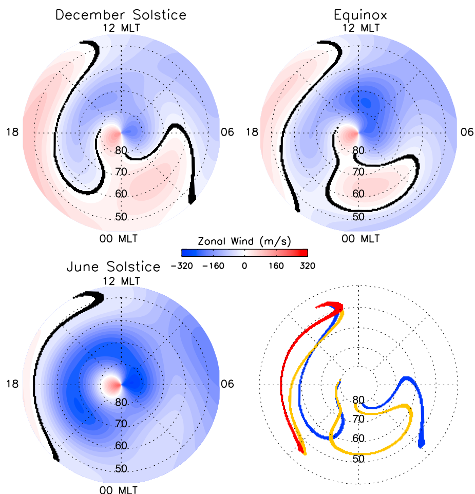
Figure 4. Polar plots of active-time assimilated zonal winds as a function of season, magnetic latitude, and magnetic local time (looking down on the geomagnetic North Pole). The black curves in the first three panels represent the boundary between westward (zonal wind negative) and eastward (zonal wind positive) zonal wind flows (wind reversal boundary). For a direct comparison, overplotted wind flow reversal boundaries for December solstice (blue), equinox (yellow), and June solstice (red) are shown in the last panel.
