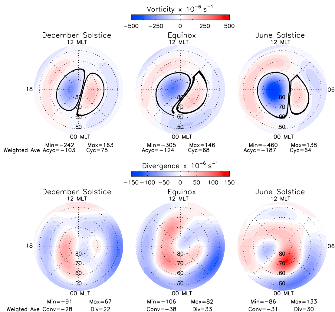
Figure 7. (top row) Vorticity and (bottom row) divergence of the empirically assimilated active-time northern high-latitude F region thermospheric vector wind fields as a function of magnetic latitude and magnetic local solar time for December solstice, equinox, and June solstice. For vorticity case, maximum anticyclonic and cyclonic vorticity ( \times 10^{-6} \text{ s}^{-1} ) for each season are listed at the bottom of each seasonal panel. The black curves mark the boundary of cyclonic and anticyclonic vortices. The cosine-latitude weighted average vorticity given at the bottom of each panel is calculated for the region inside the black boundaries, which mark the reversal of the sign of the vorticity. For the divergence case, peaks (minimum and maximum) and weighted averages are calculated over the entire shown area.
