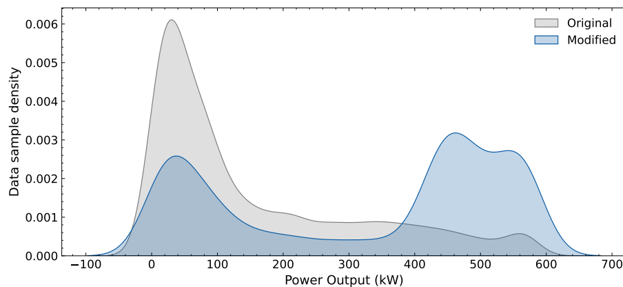
Figure 4: Data density of the original and modified (after SMOGN application) healthy data set
