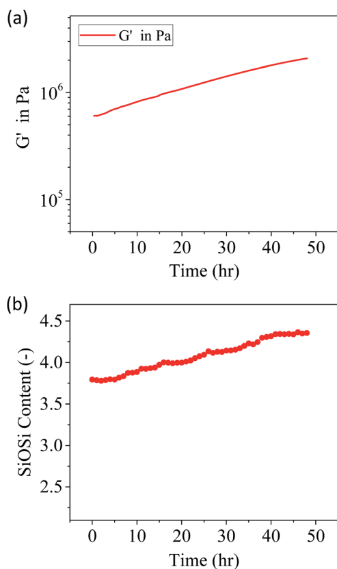
Fig. 5 Evolution of G' (a) and content of Si–O–Si links (b) in a 2 h-cured hybrid sol–gel polymer during a rheological time-sweep scan performed at 70 °C.
