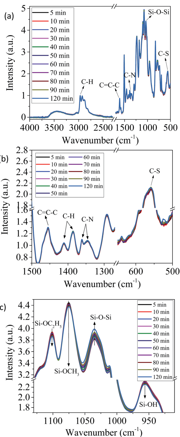
Fig. 3 FTIR spectra of the hybrid sol-gel polymer cured for 2 h and further cured at 100 °C during a time-sweep rheological scan: spectral range of 4000–500 cm -1 (a), 1500–500 cm -1 (b) and 1150–900 cm -1 (c).
