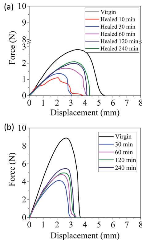
Fig. 9 Force-displacement plots of the virgin and healed DENT specimens for the 2 h-cured (a) and the 48 h-cured (b) hybrid sol-gel polymer.
