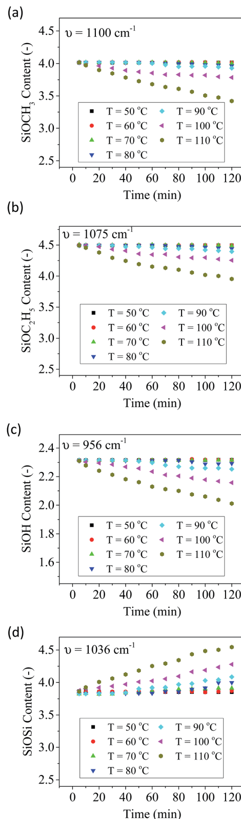
Fig. 4 Evolution of \text{SiOCH}_3 (a), \text{SiOC}_2\text{H}_5 (b), \text{SiOH} groups (c) and Si–O–Si bonds (d) of the hybrid sol–gel polymer cured for 2 h and further cured at different temperatures in a rheological time-sweep scan.
