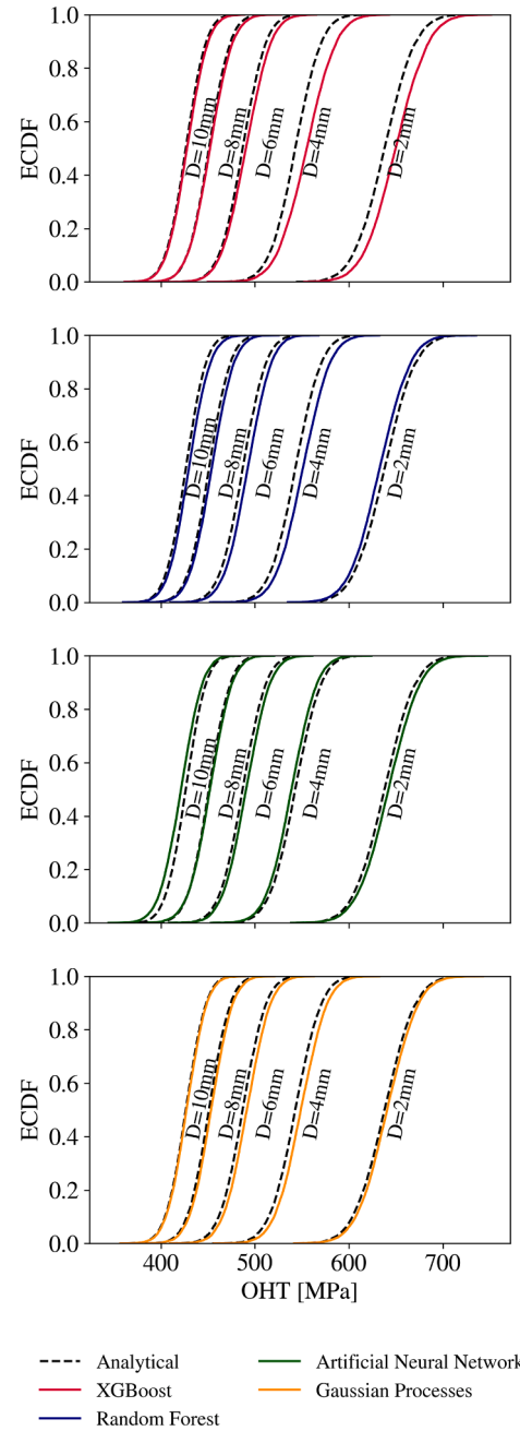
Fig. 15. Double-Double: ECDF obtained using the analytical model and the trained machine learning models (IM7/8552 DD [45/−45/20/−20] laminate, D = 2 –10 mm and W = 12 –60 mm).
