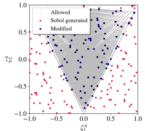
Fig. 5. Sobol sampling modification for Legacy Quad laminates.
