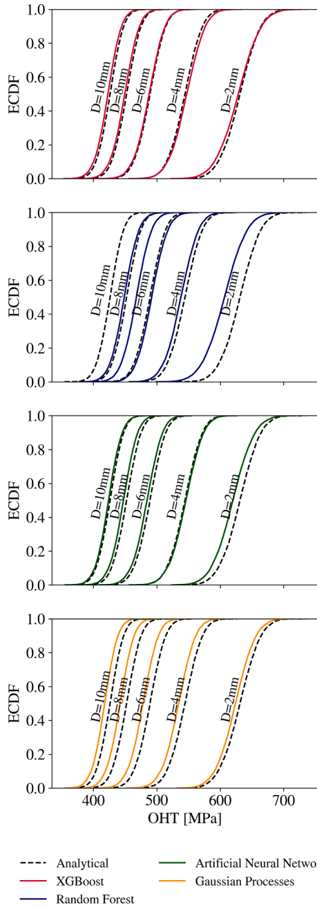
Fig. 14. Legacy Quad: ECDF obtained using the analytical model and the trained machine learning models (IM7/8552 [90/0/−45/45] 3s , D = 2 –10 mm and W = 12 –60 mm).
