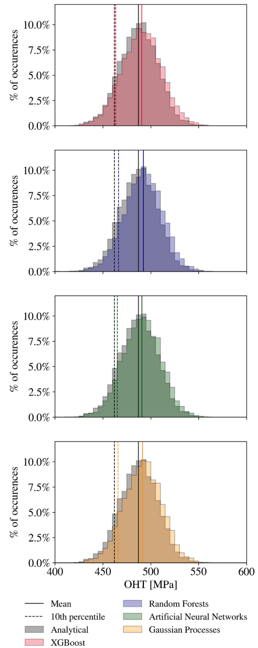
Fig. 13. Double-Double: distribution of the notched strengths, B-basis (dashed lines) and mean value (full lines) provided by the analytical model and the trained machine learning models (IM7/8552 DD [45/−45/20/−20] laminate, D = 6 mm and W = 36 mm).
