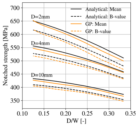
Fig. 16. Design chart for diameter-to-width ratio, 1/8 < D/W < 1/3 and hole diameters D = 2, 4, 10 mm for an IM7/8552 [90/0/-45/45] 3s Legacy Quad laminate obtained using the analytical framework and the Gaussian Processes model.
