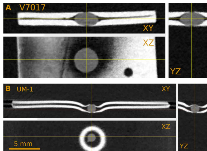
Fig. 4. Orthogonal cross sections of computed tomography of the Van Leeuwenhoek microscopes from Leiden and Utrecht, as shown in Fig. 1. (A) The cross sections of the lentil-shaped lens of the medium-powered microscope (V7017). (B) The circular cross section of the high-powered microscope (UM-1). The XZ projection shows that this ball-shaped lens has a tiny glass stem connected to it.
