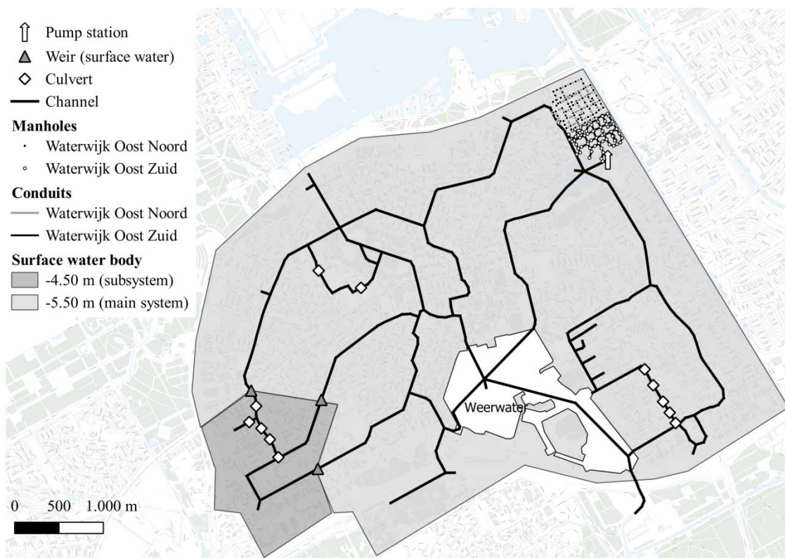
Figure 7 | The urban water system of Almere.
