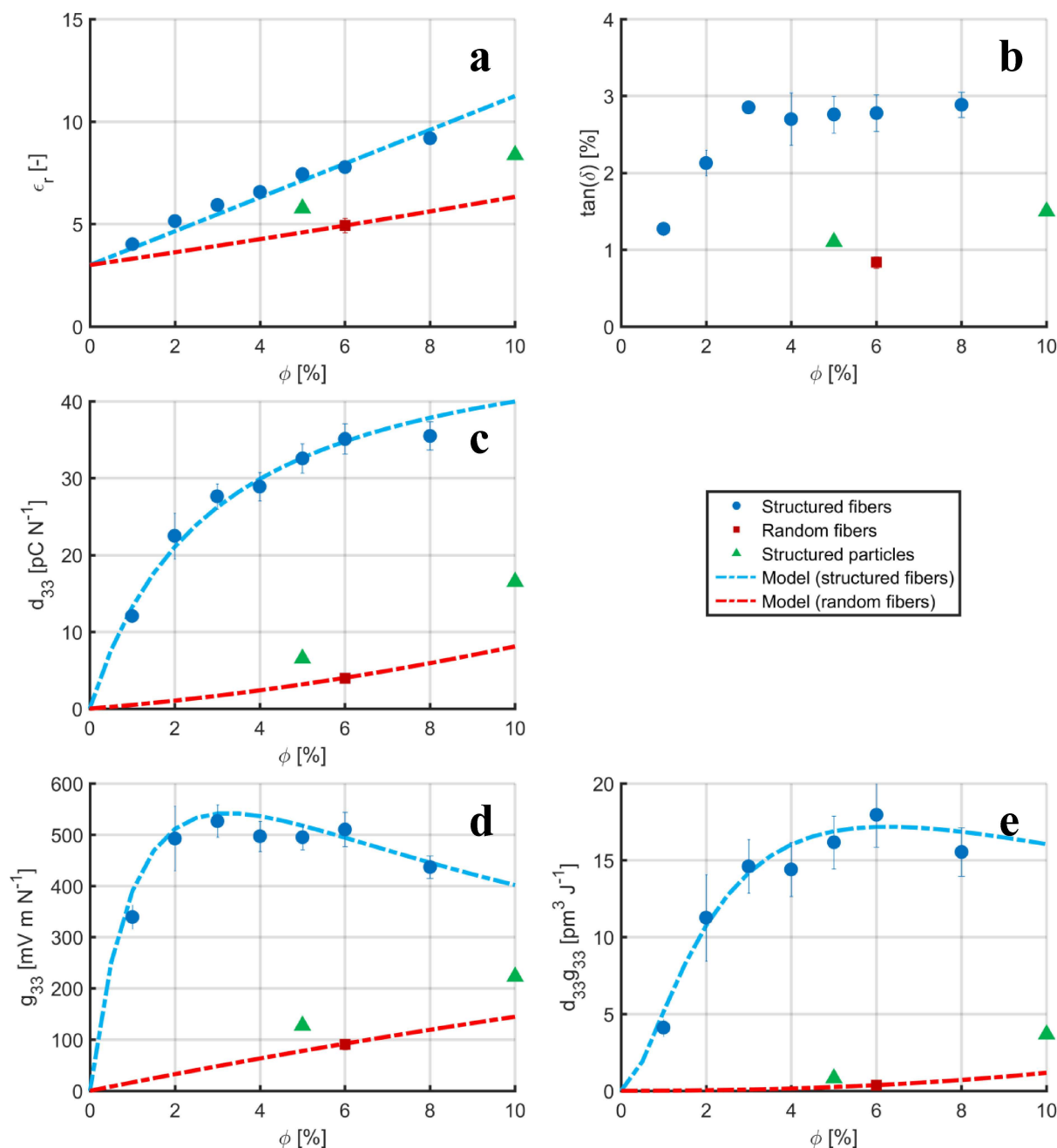
Figure 4. Piezoelectric- and dielectric constants of random 0–3 and structured quasi 1–3 KNLN/PDMS fiber composites as a function of KNLN volume fraction, \phi . Blue circles refer to structured composites and red squares refer to random composites. a) The relative dielectric constant, \epsilon_r , b) the dielectric loss, \tan(\delta) , c) the piezoelectric charge coefficient, d_{33} , d) the piezoelectric voltage coefficient, g_{33} , e) the stress energy density, d_{33}g_{33} . For comparison, reported data of quasi 1–3 particle KNLN/PDMS composites are included as the green triangles. [25] The dash-dotted lines are a guide for the eye, calculated with the same models as used in Figure 1.
