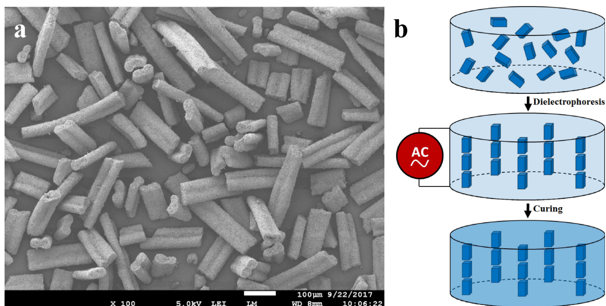
Figure 2. (a) SEM micrograph of the sintered KNLN fibers. (b) Schematic representation of the alignment of the piezoelectric fibers using dielectrophoresis.
