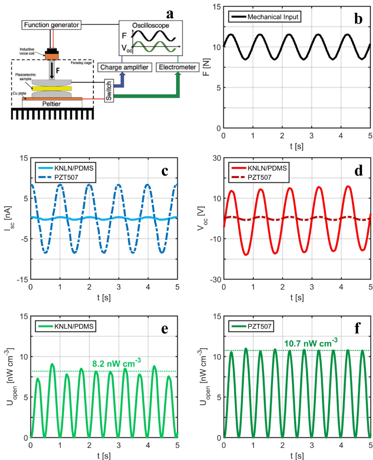
Figure 5. Electrical response to a mechanical input of KNLN/PDMS and PZT507, both having a thickness of 1 mm and an area of 50 mm 2 , measured using a specifically designed piezometer system. a) Schematic representation of the piezometer system, [10] b) the mechanical input, F , c) the short circuit current, I_{sc} , d) the open circuit voltage, V_{oc} , and the stored electrical energy, U_{open} , of e) KNLN/PDMS and f) PZT507, respectively.
