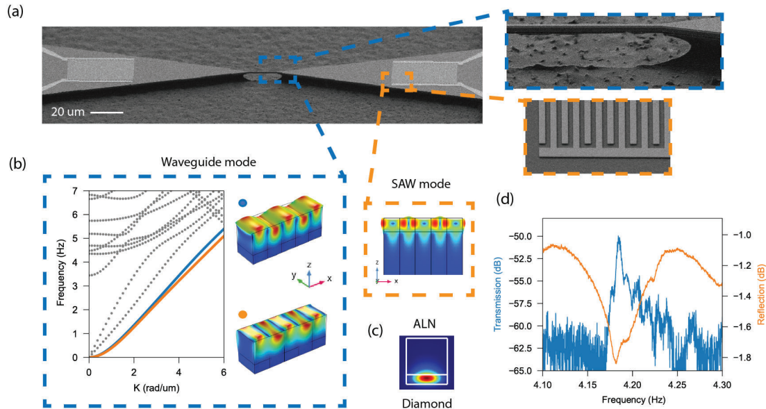
Fig. 1. a) Scanning electron microscope images of the fabricated waveguide, tapered regions, and associated IDTs. The electrode thickness is 100 nm and the period is 2 \mu\text{m} . The waveguide is 785 nm wide and has a 700-nm-thick layer of ALN on top of 200 nm of diamond. Devices with lengths ranging from 5 to 20 \mu\text{m} all showed at least -70 dB of transmission. The insets show the detail of the IDT and the taper connected to the suspended waveguide. b) Mechanical simulation results of the device. The color shows total displacement. c) Optical simulation of the waveguide. The color corresponds to normalized electric field intensity, and the field is confined mostly in diamond. d) Measured transmission and reflection of the device.
