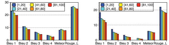
Figure 2: Results of question generation with different source sentence lengths..
