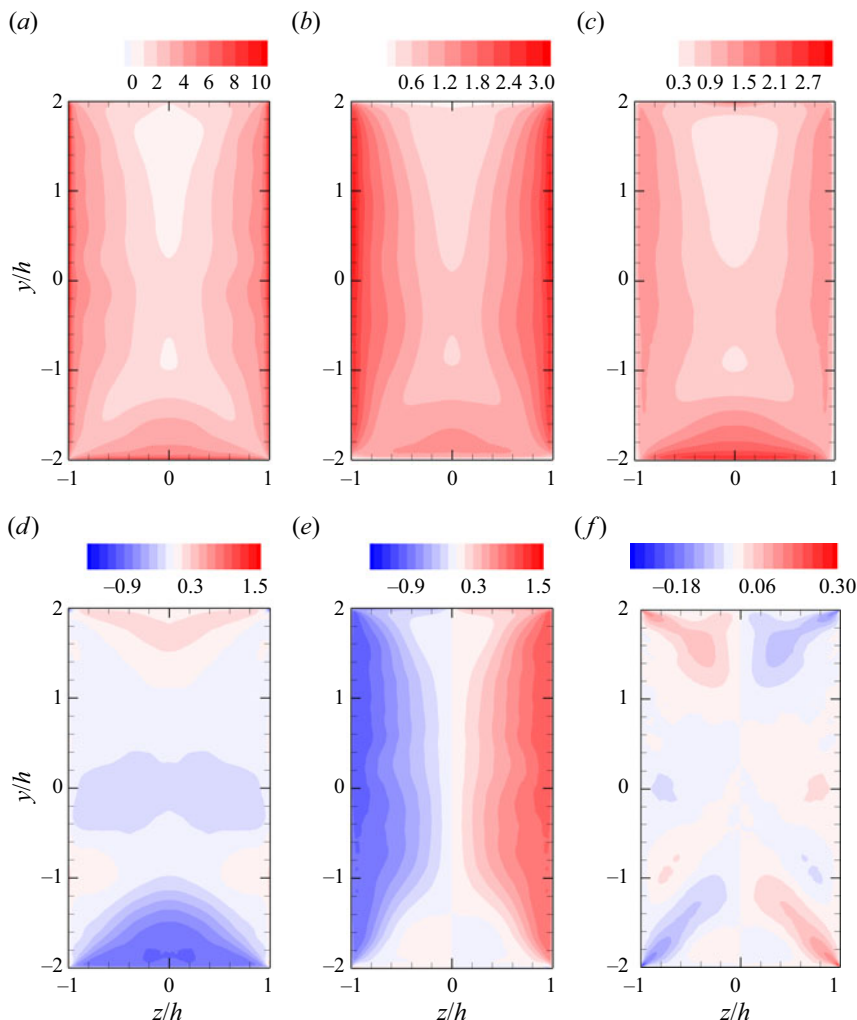
Figure 17. Components of the Reynolds stress tensor in the cross-stream plane for case AR05-H: (a) \tau_{11}^+ , (b) \tau_{22}^+ , (c) \tau_{33}^+ , (d) \tau_{12}^+ , (e) \tau_{13}^+ , (f) \tau_{23}^+ .
