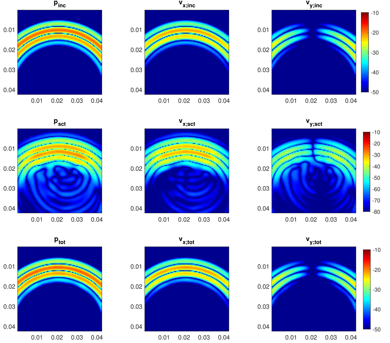
FIG. 4. Snapshots of incident (top row), scattered (middle row) and total fields (bottom row) at t = 28 \mu\text{s} . Left column shows the pressure field; the middle and right columns the particle velocity fields. All fields are normalized with respect to the maximum absolute value and shown on a dB scale.
