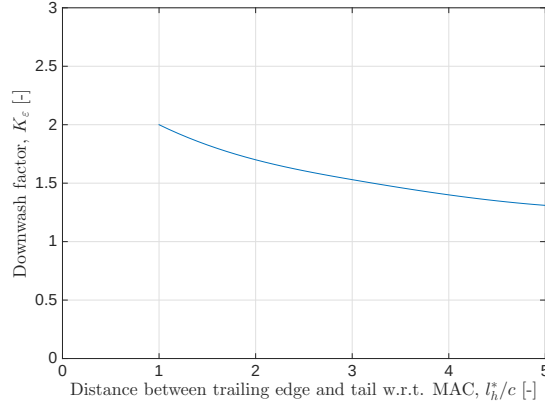
Figure 5. Downwash factor K_\varepsilon versus distance behind the wing trailing edge. 4
