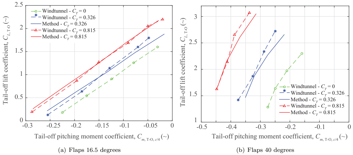
Figure 11. Tail-off pitching moment curves - Fokker 50I
