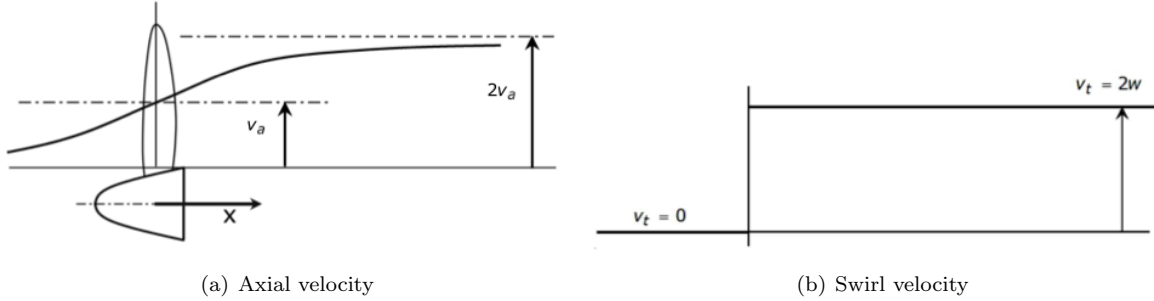
Figure 2. Velocity variations induced by the propeller. 2
