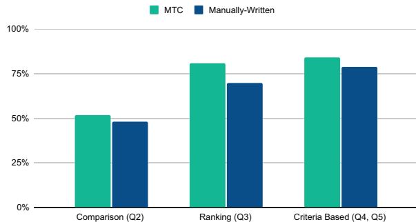
Fig. 7. Understandability of MicroTestCarver versus manually written tests
