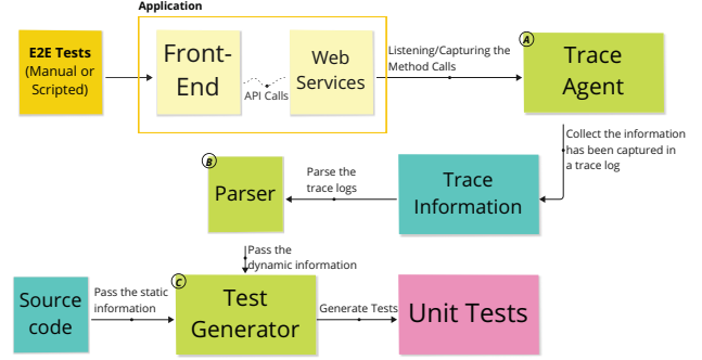
Fig. 1. Overview of the carving framework
