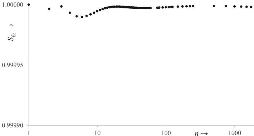
Fig. 7. The similarity of w_{i,n,mod} and w_{i,n,ref.} , i.e. between the WLR weight algorithm and theory.
