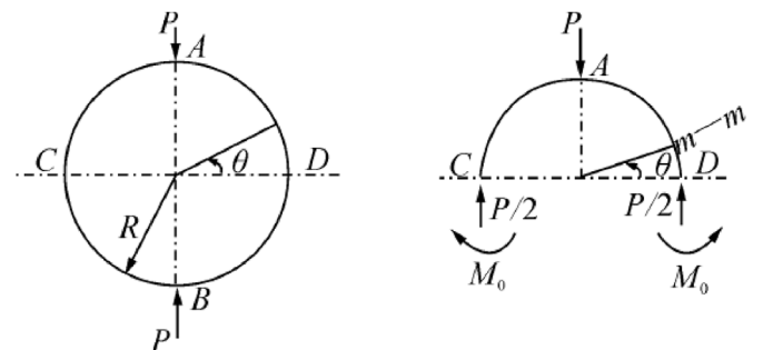
Fig. 2. Schematic diagram of a ring compressed in the radial direction (Tang et al., 2016).
