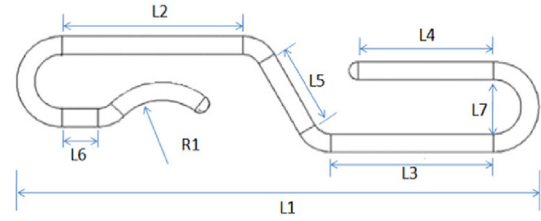
Fig. 5. Schematic diagram of the carcass profile (Tang et al., 2016).
