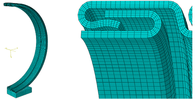
Fig. 6. Radial compressed carcass model, (a) whole view and (b) detailed view.
