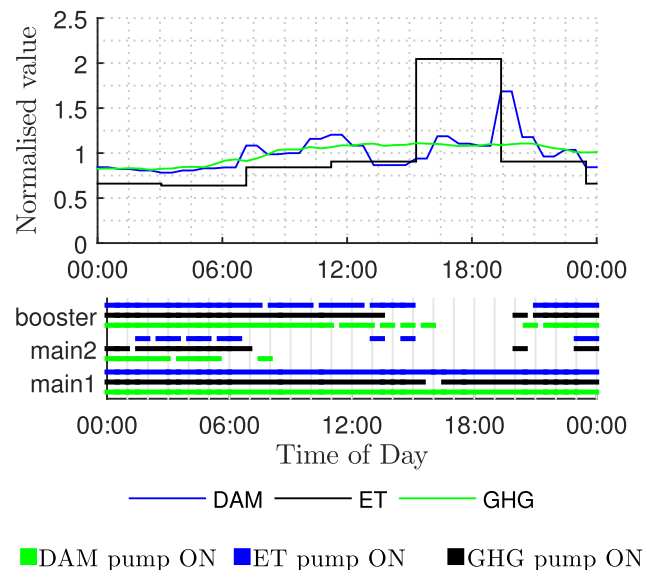
Fig. 4. Calculated pump schedules that take into consideration the various electricity tariffs, green house gas emissions and the day-ahead market prices. The inputs are normalised to have a mean of 1.
