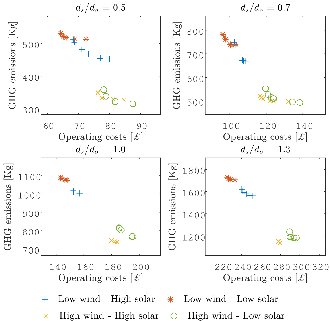
Fig. 6. Pareto fronts ( Green* scenario) that quantify the trade-offs in reducing both the operating (electricity) costs and GHG emissions based on the pump utilisation rate and energy supply scenarios.
