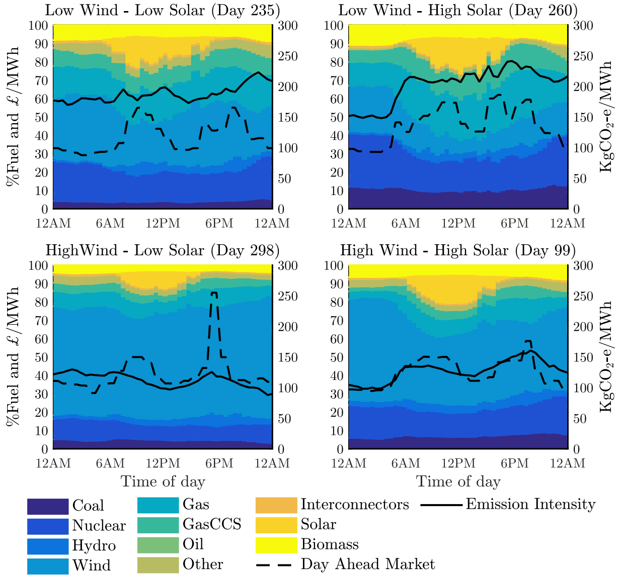
Fig. 2. Fuel mix share and electricity prices for the selected days of the 2035 Green (UK) scenario. The left y-axis shows fuel mix share and spot market prices, the right y-axis represents the emission intensity.
