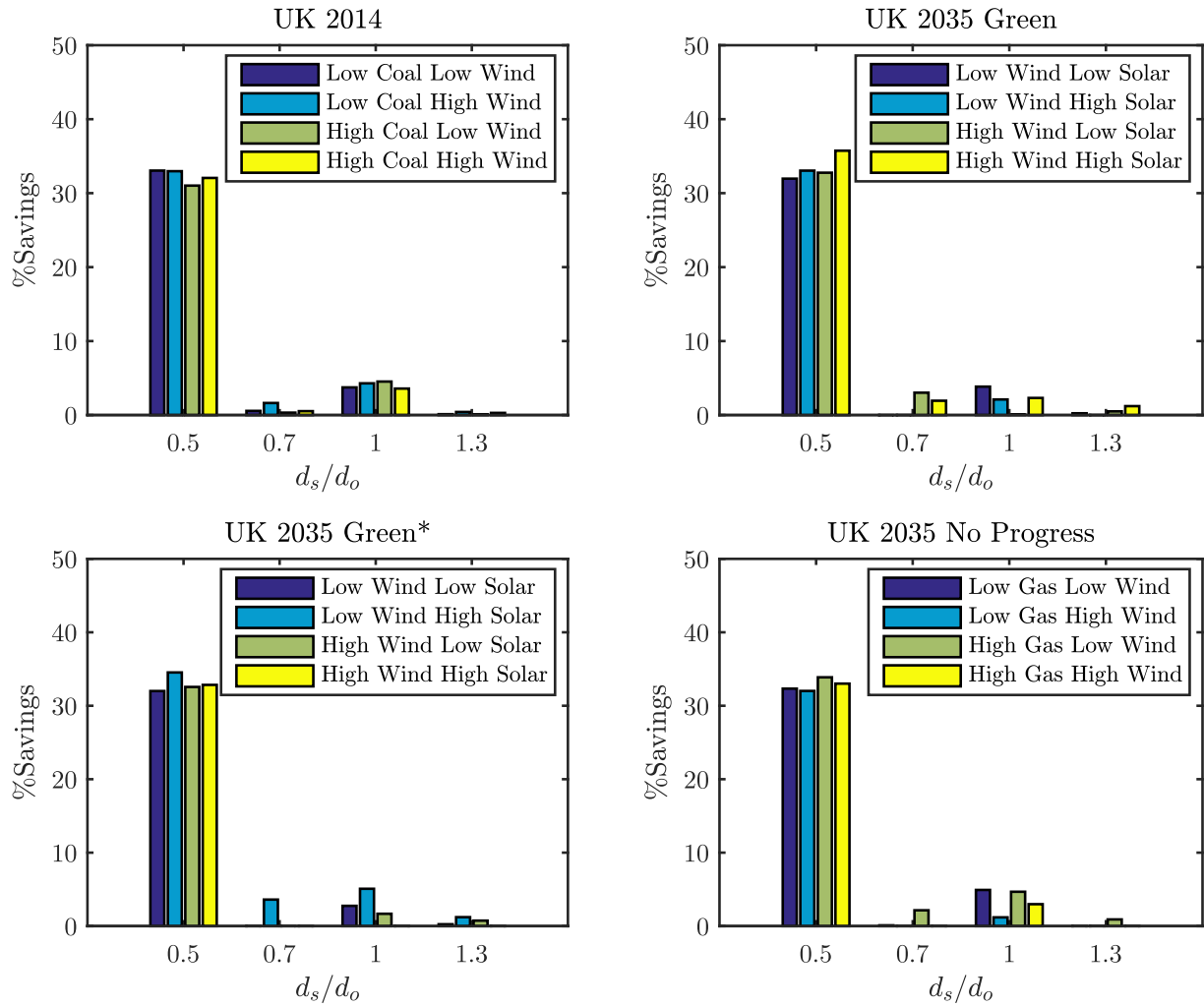
Fig. 5. Pump utilisation rate versus the reduction (savings) in GHG emissions when changing electricity tariffs from TOU to DAM for all energy supply scenarios and operating days.
