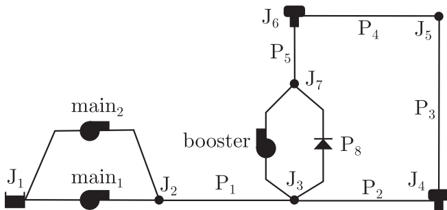
Fig. 3. Benchmark case study adopted from [33].
