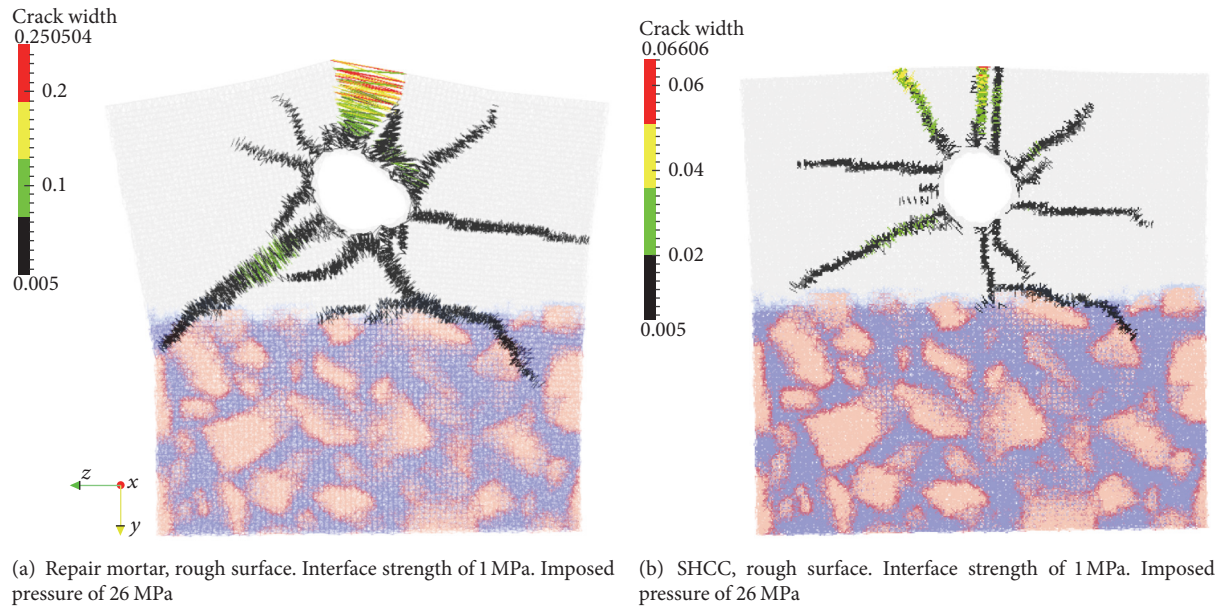
FIGURE 17: Numerically obtained crack pattern and maximum crack widths due to the pressure imposed by expanding bar in repair systems and influence of different types of repair materials; top: repair material; bottom: substrate (deformation scaled 20x; note that for different samples maximum crack widths are different).
