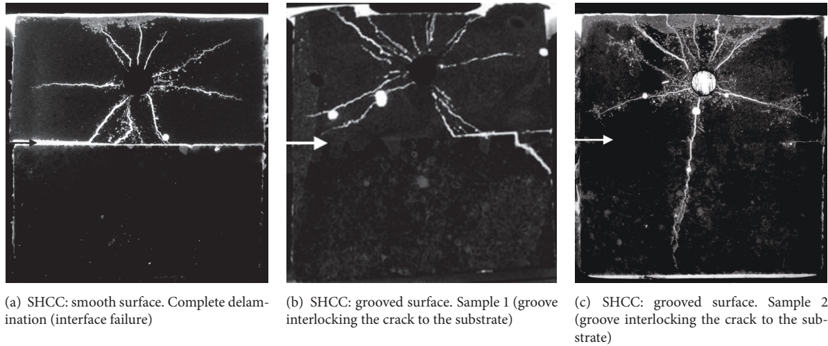
FIGURE 15: Experimentally obtained damage patterns when SHCC is used as a repair material (top: repair material; bottom: mortar substrate; interface is indicated with the arrow); samples are epoxy impregnated and imaged under UV light.
