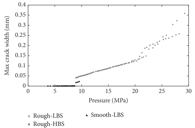
FIGURE 13: Influence of interface strength and substrate surface roughness on imposed internal pressure and corresponding maximum crack widths prior to repair system failure. Plain mortar is used as a repair material (LBS corresponds to interface strength 1 MPa and HBS to interface strength 3 MPa).
