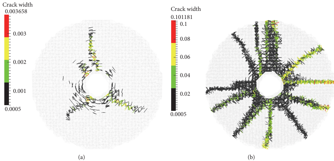
FIGURE 11: Lattice simulation of corrosion induced cracking of experiments reported in [13] (a) in mortar (imposed internal pressure of 17.32 MPa) and in (b) SHCC (imposed internal pressure of 103.58 MPa).
