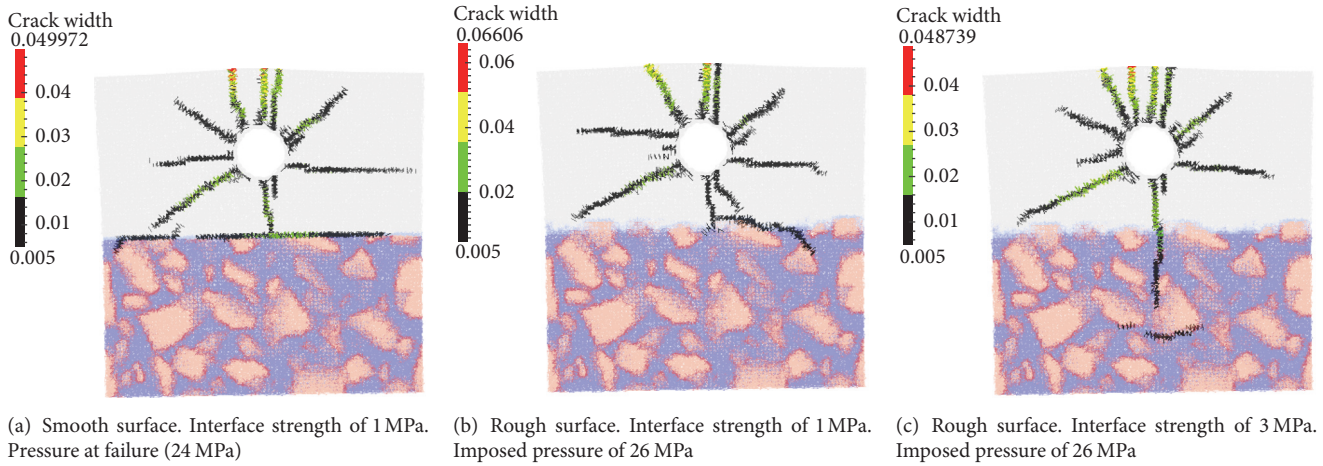
FIGURE 14: Numerically obtained crack pattern and maximum crack widths due to the pressure imposed by expanding bar in repair systems. SHCC is used as a repair material, influence of the substrate surface roughness, and the interface strength (deformation scaled 20x; note that for different samples maximum crack widths are different).
