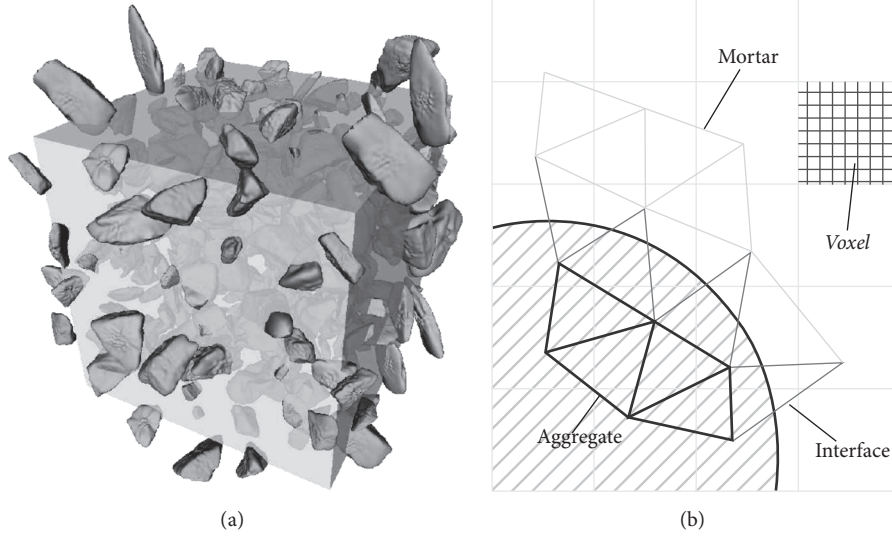
FIGURE 6: (a) Aggregates in the concrete substrate generated by Anm model [22]; (b) two-dimensional overlay procedure for generation of the lattice model in interface zone between aggregate and substrate mortar (ITZ) [23].
