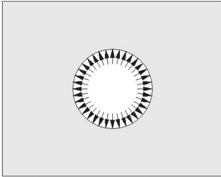
FIGURE 9: Pressure distributions caused by uniform corrosion, as applied in simulations [12].
