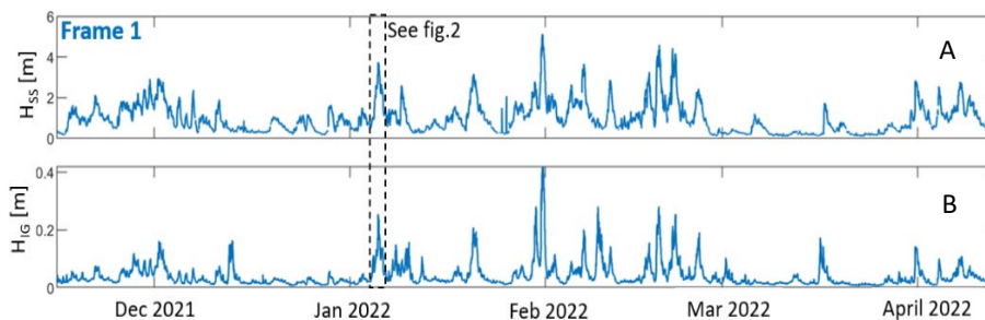
Fig. 1: Sea-swell (SS, f > 0.05\text{Hz} ) and infragravity (IG, 0.005 < f < 0.05\text{ Hz} ) significant wave heights at the most offshore frame ( \bar{d} = 14.5\text{m} ) during the 5-month campaign.
