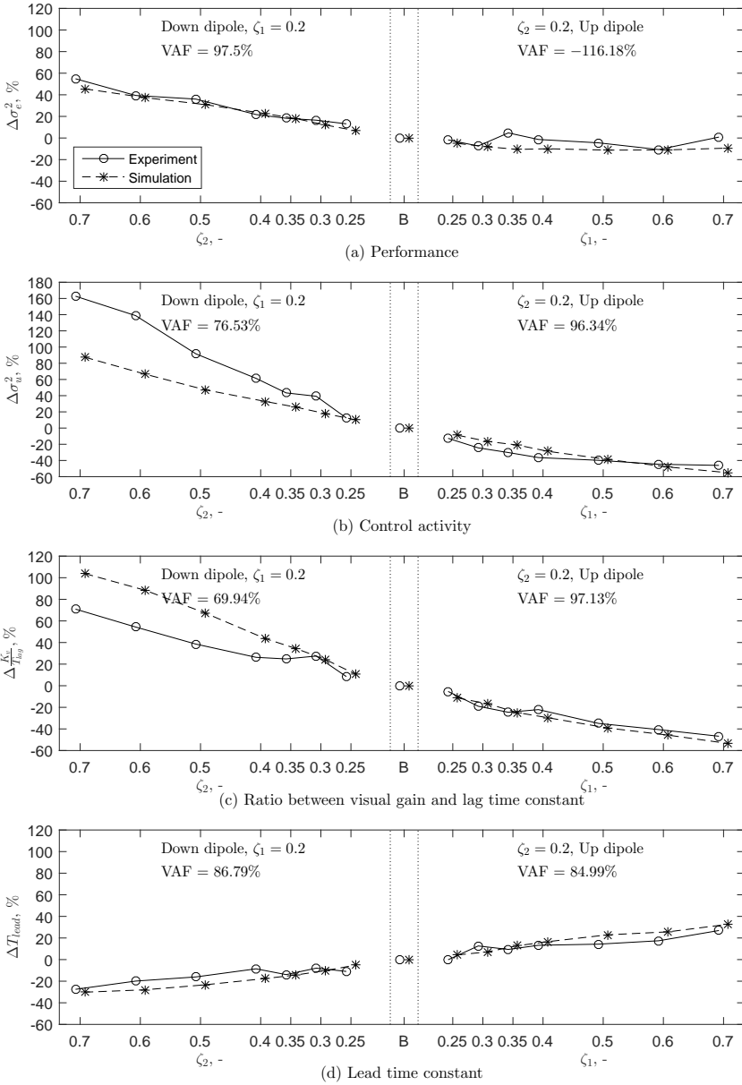
Figure 6.11: Comparison of the relative changes of the medians with respect to the baseline between the experiment and simulation results. The VAF values are shown to indicate the fittings of the simulation data to the experiment results for the up and down dipoles, respectively.
