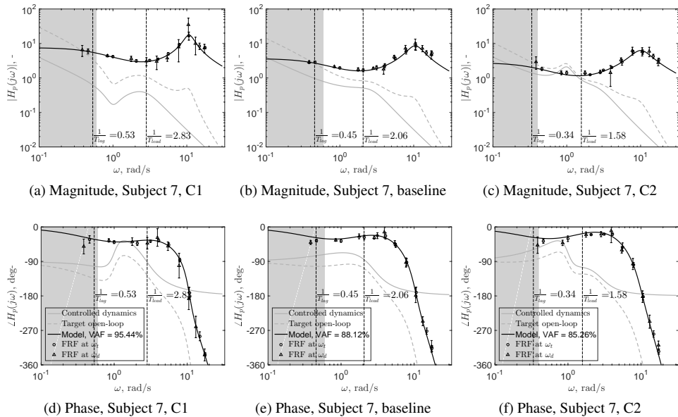
Figure 4.13: Subject 7 compensatory model fits and frequency response functions for conditions of C1, baseline and C2. The shaded area in each figure indicates the frequency range within which the controlled dynamics are single integrator like.
