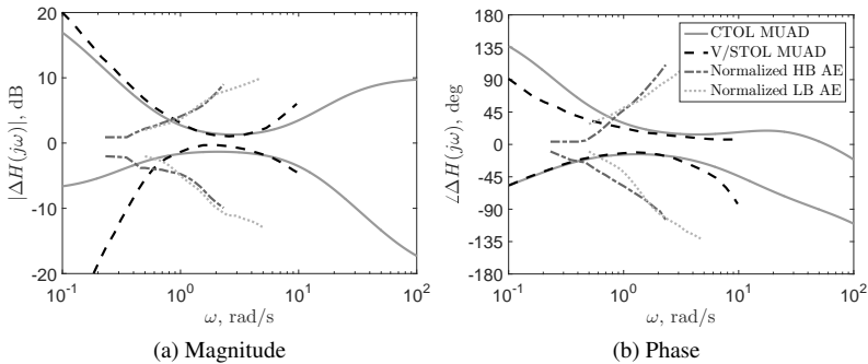
Figure 1.3: Comparisons among CTOL Maximum Unnoticeable Added Dynamics (MUAD) envelopes [67], V/STOL MUAD [72], normalized high-bandwidth (HB) Allowable Error (AE) envelopes and normalized low-bandwidth (LB) AE [74].
