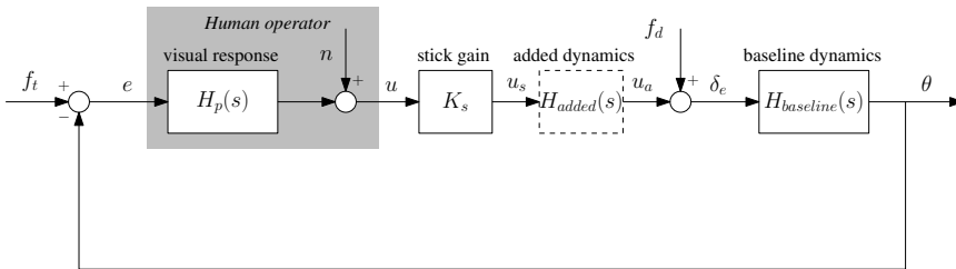
Figure 4.1: A schematic representation of the aircraft pitch attitude tracking task.
