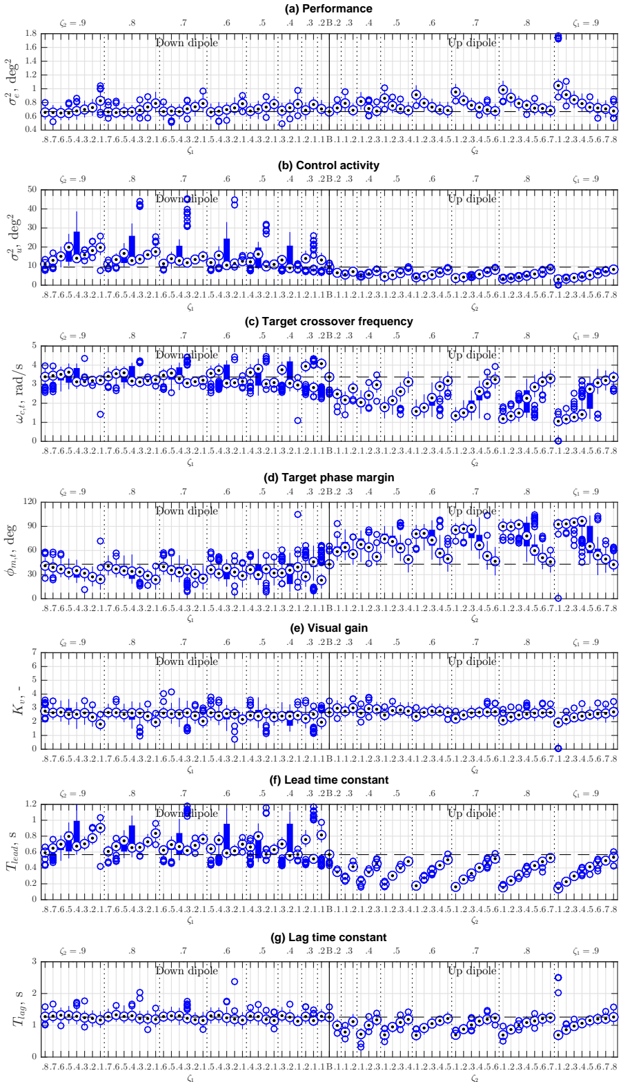
Figure C.3: All simulation results at \omega_{dp} = 6 \text{ rad/s} .
