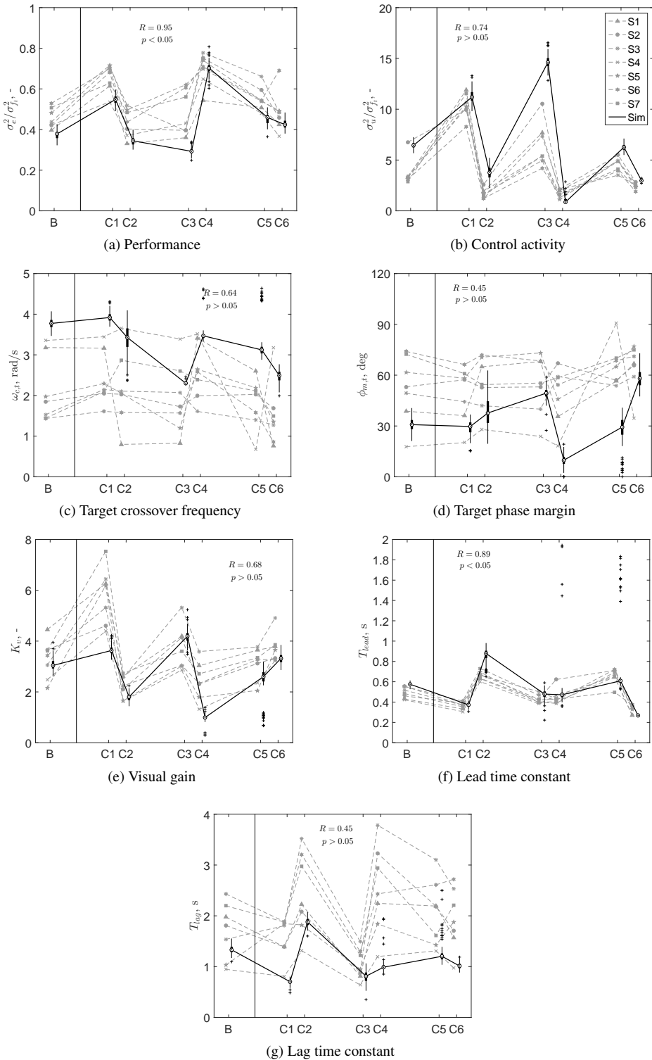
Figure A.2: Comparison between experiment and simulation results (in simulation \sigma_n^2 / \sigma_u^2 = 0.15 ).
