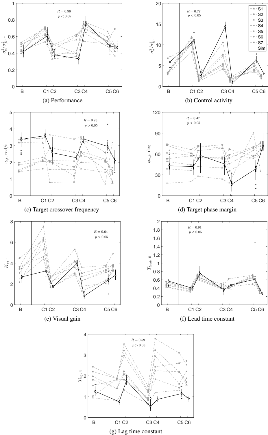
Figure A.4: Comparison between experiment and simulation results (in simulation \sigma_n^2 / \sigma_u^2 = 0.25 ).
