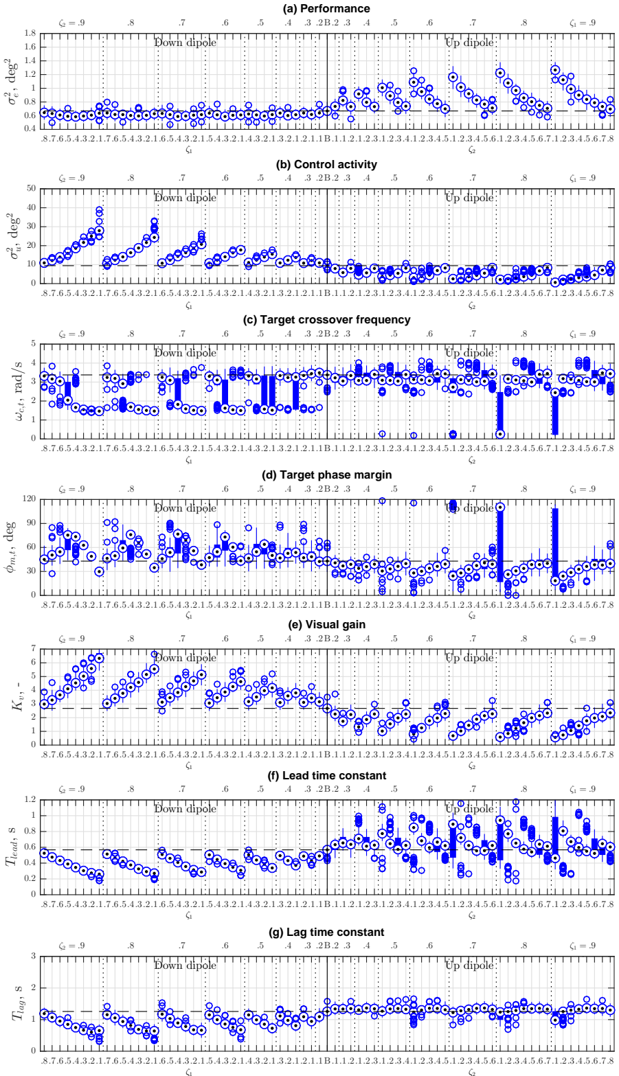
Figure 5.9: All simulation results at \omega_{dp} = 2 rad/s.
