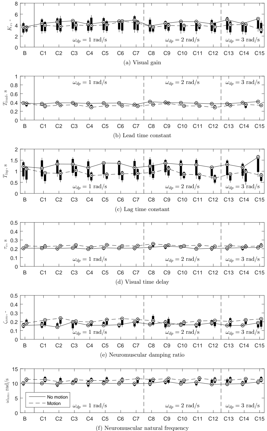
Figure D.6: Comparison of the human operator model parameters between no-motion and motion cases.
