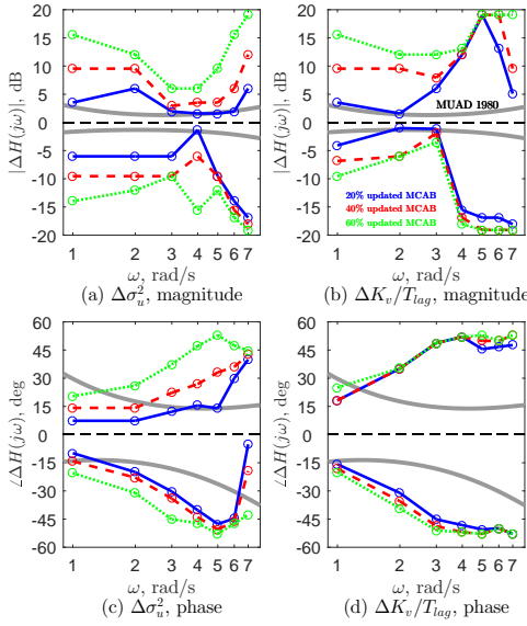
Figure 6.14: The updated MCAB for \Delta\sigma_u^2 and \Delta K_v/T_{lag} .
