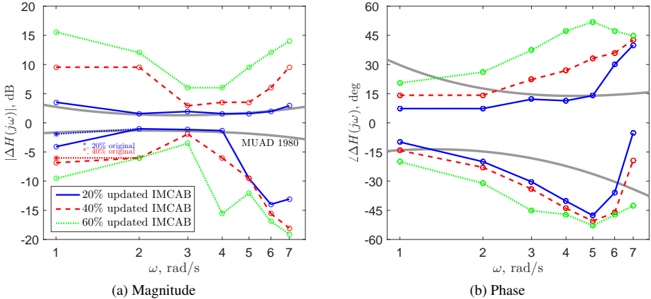
Figure 6.13: The updated simulation-based IMCAB based on the intersection part of all sub-figures of Figure 6.12 for magnitude and phase, respectively. Figure 6.13a also shows the changes compared with the original simulation-based IMCAB developed in Chapter 5.
