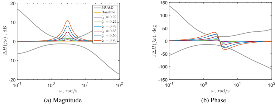
Figure 3.3: MUAD and all added dynamics.
