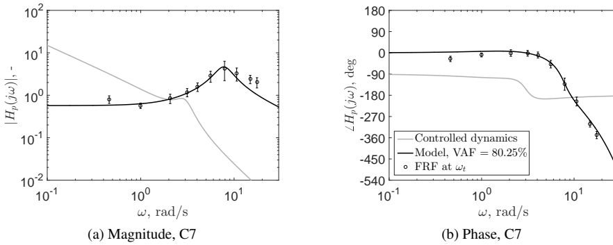
Figure 3.7: Example of human operator model fitting results for C7 (Subject 7).
