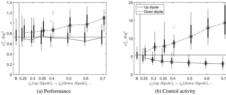
Figure 6.5: Variance of the error signal e and control signal u for each condition of fifteen subjects. The asterisk mark the conditions significantly different from the baseline (B) based on a Wilcoxon signed-rank test ( p < 0.0036 ).
