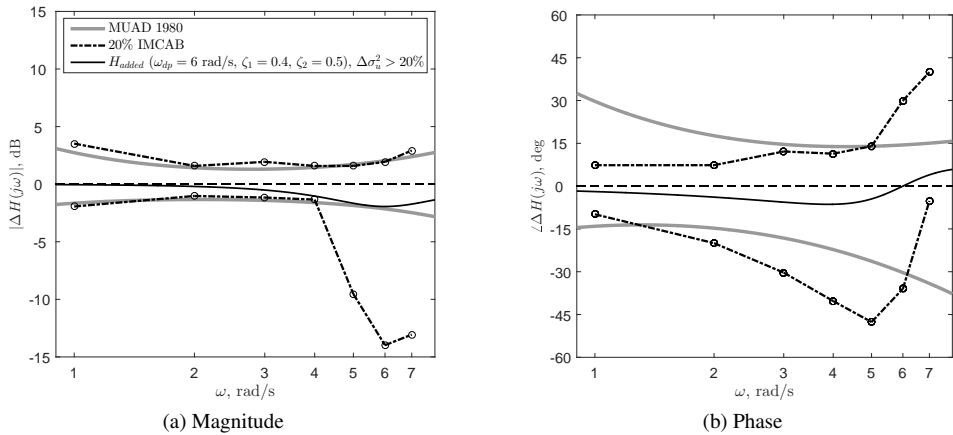
Figure 5.15: Integrated Manual Control Adaptation Boundaries (IMCAB) of 20% with the added dipole dynamics ( \omega_{dp} = 6 rad/s, \zeta_1 = 0.4 , \zeta_2 = 0.5 ) of which \Delta\sigma_u^2 > 20\% .
