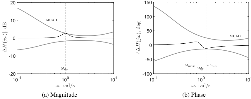
Figure 5.5: An example of an added dipole within the MUAD magnitude envelope and an added dipole within the MUAD phase envelope.
