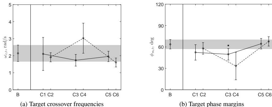
Figure 4.11: Target crossover frequencies and phase margins for each condition, averaged over seven subjects. The grey area marks the range of the baseline condition, and the asterisk marks the condition significantly different from the baseline condition.
