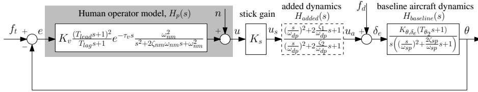
Figure 6.1: A schematic representation of the aircraft pitch attitude tracking task.
