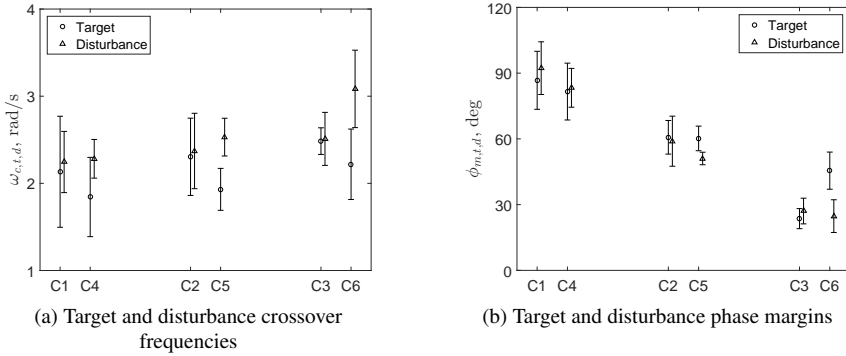
Figure 2.6: Target, disturbance crossover frequencies and phase margins for each condition averaged over six subjects.
