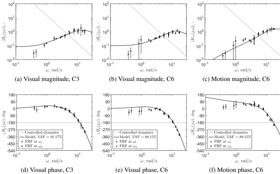
Figure 2.9: Example of human operator model fitting results for C3 and C6 (Subject 4).
