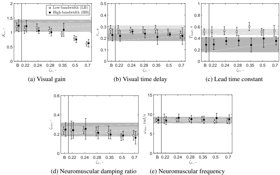
Figure 3.8: Estimated human operator model parameters.
