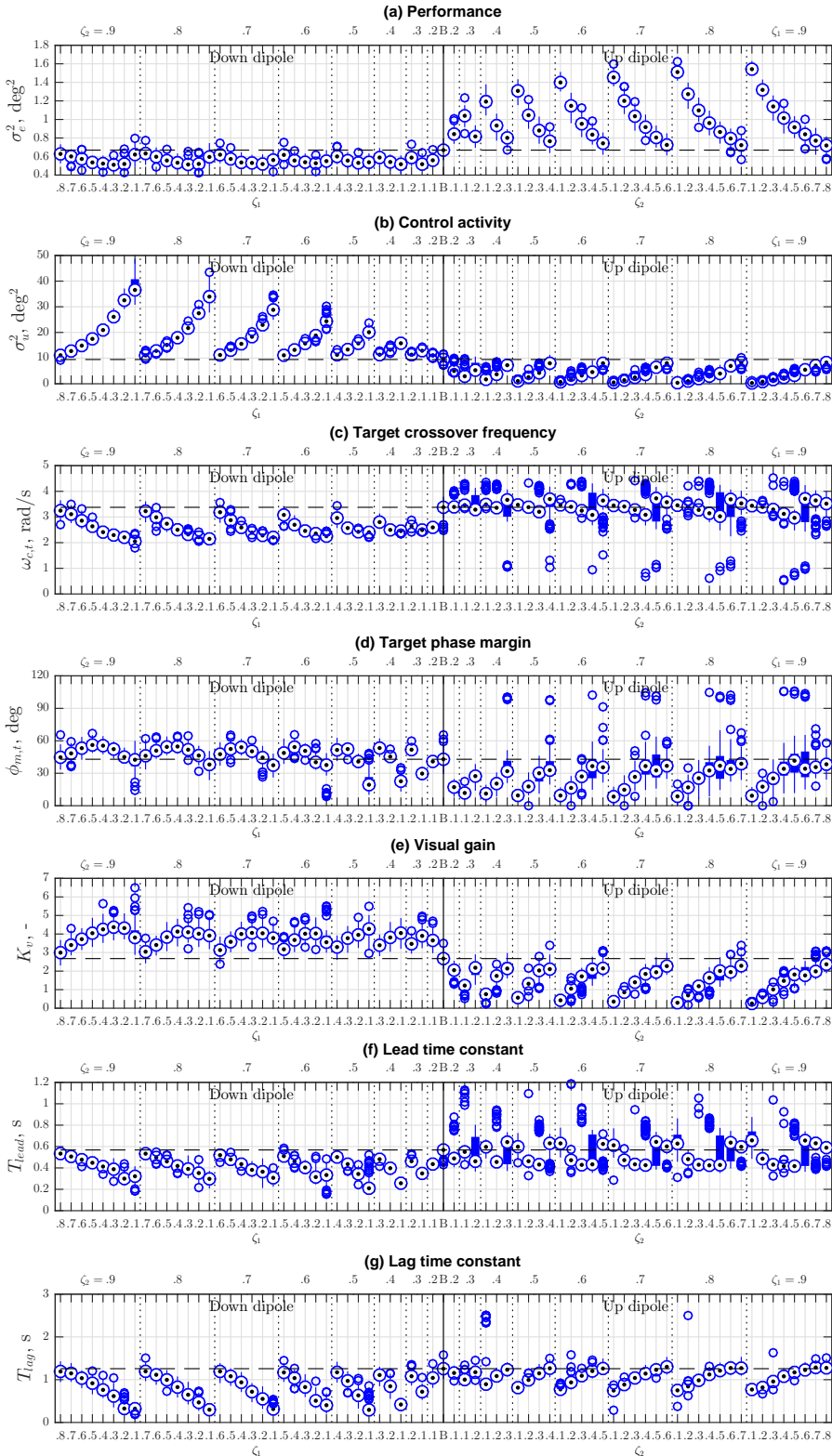
Figure 5.10: All simulation results at \omega_{dp} = 3 rad/s.
