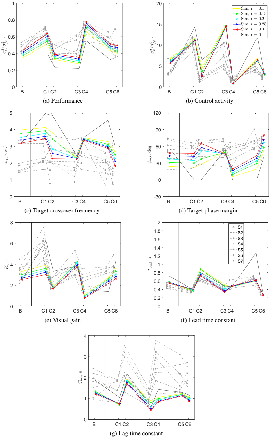
Figure 4.15: Comparison between experiment and simulation results with different remnant ratios.
