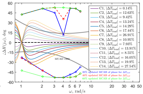
(h) Phase, \Delta T_{lag}
