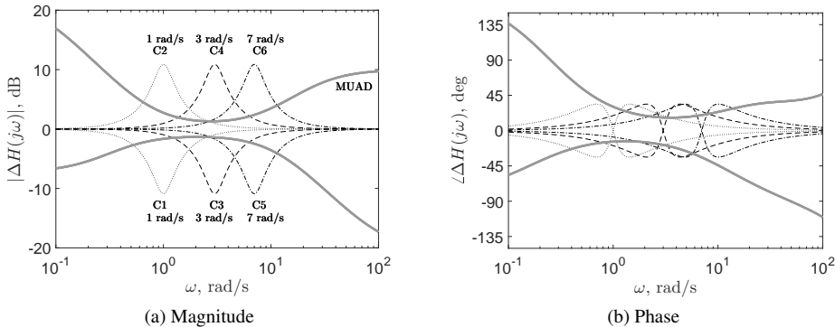
Figure 4.3: MUAD and all added dynamics.
