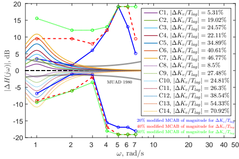
(e) Magnitude, \Delta K_v/T_{lag}
