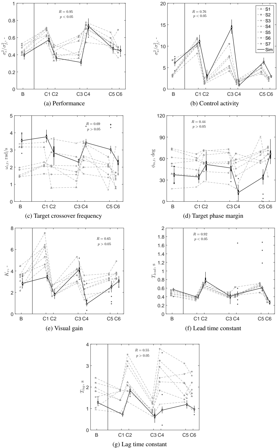
Figure A.3: Comparison between experiment and simulation results (in simulation \sigma_n^2 / \sigma_u^2 = 0.2 ).
