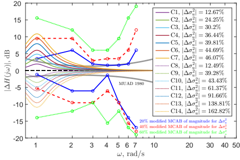
(c) Magnitude, \Delta\sigma_u^2
