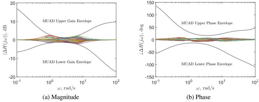
Figure 5.6: MUAD [1] with the tested added dipole dynamics within the envelopes.
