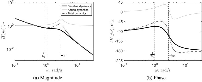
Figure 4.2: Bode plot of the baseline aircraft dynamics, the added dynamics, and the total controlled dynamics.
