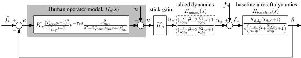
Figure 5.1: A schematic representation of the aircraft pitch attitude tracking task for simulation.
