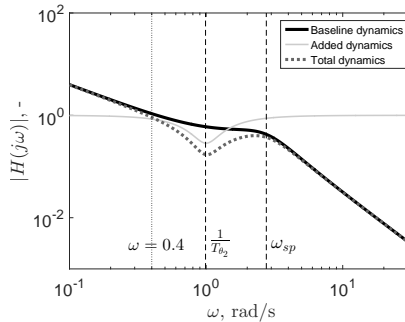
Figure 4.5: An indication of the lowest frequency for human operator to generate lead.
