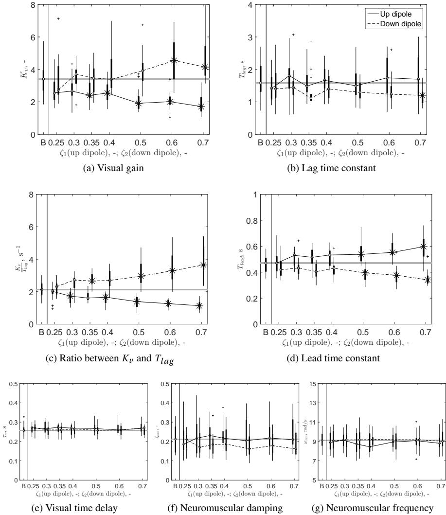
Figure 6.8: Human operator model parameters. The asterisk mark the conditions significantly different from the baseline (B) based on a Wilcoxon signed-rank test ( p < 0.0036 ).
