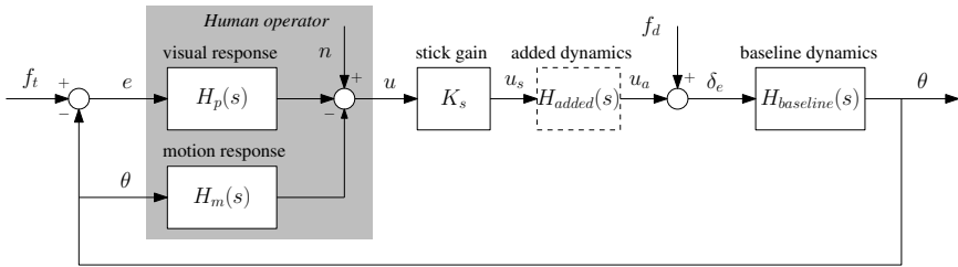
Figure D.1: A schematic representation of the aircraft pitch attitude tracking task with motion feedback.
