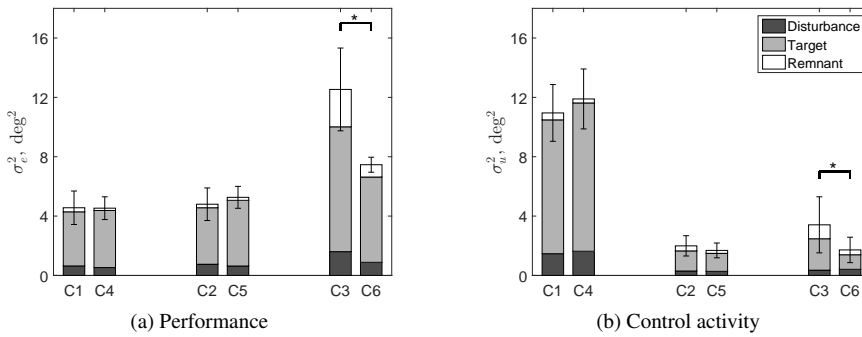
Figure 2.5: Variance decompositions of the error signal e and control signal u for each condition averaged over six subjects.
