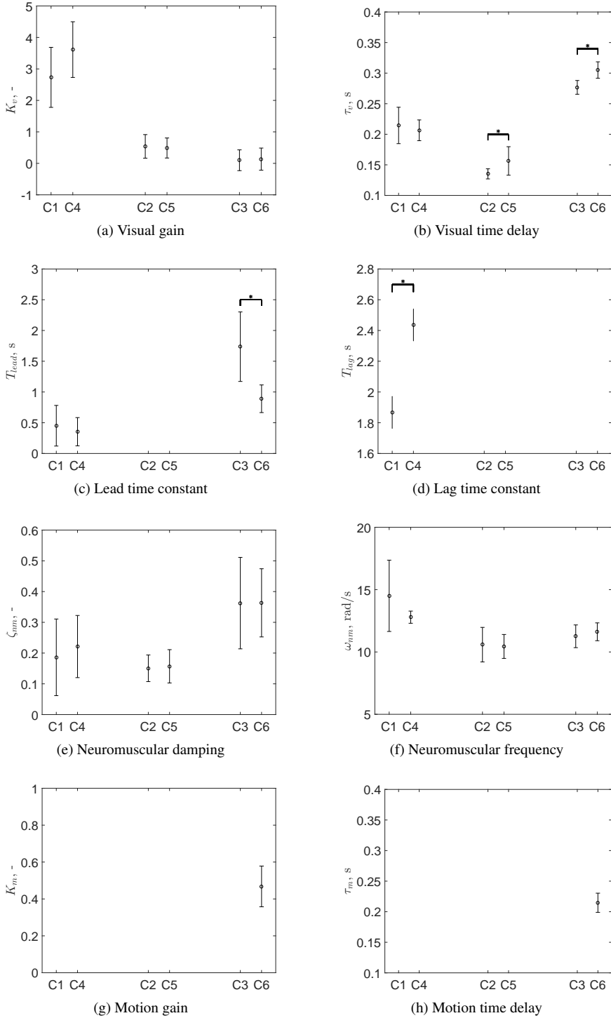
Figure 2.10: Estimated human operator model parameters.
