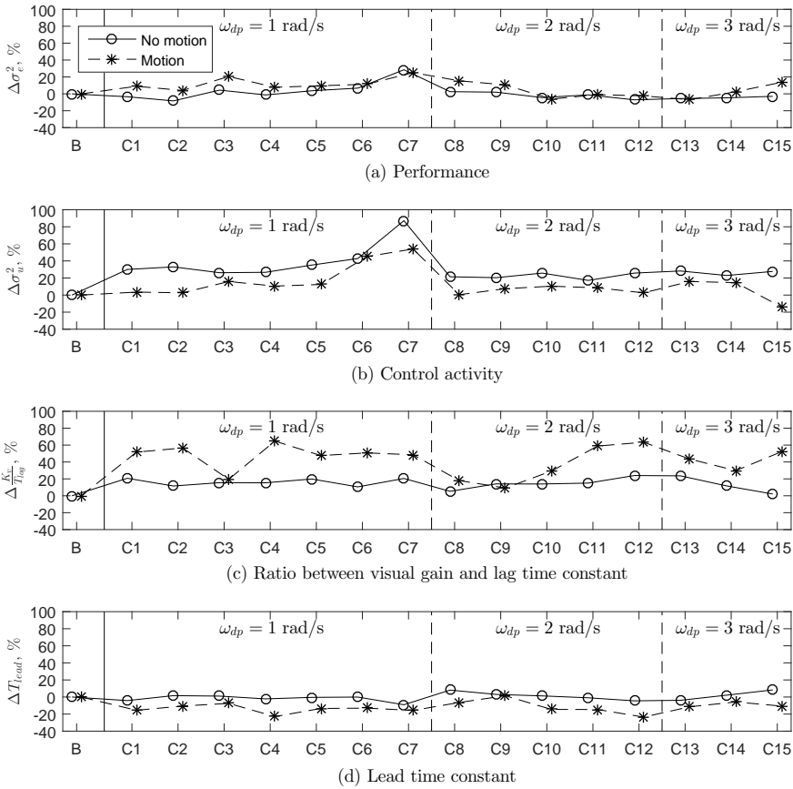
Figure D.7: Comparison of the dependent measures quantifying the MCAB between no-motion and motion cases.
