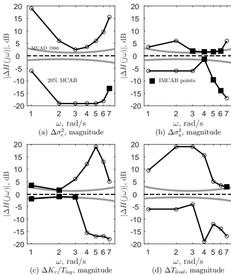
Figure 5.3: An example of the Manual Control Adaptation Boundaries (MCAB) of magnitude of 20%. The solid points closest to the 0 dB line form Figure 5.4.
