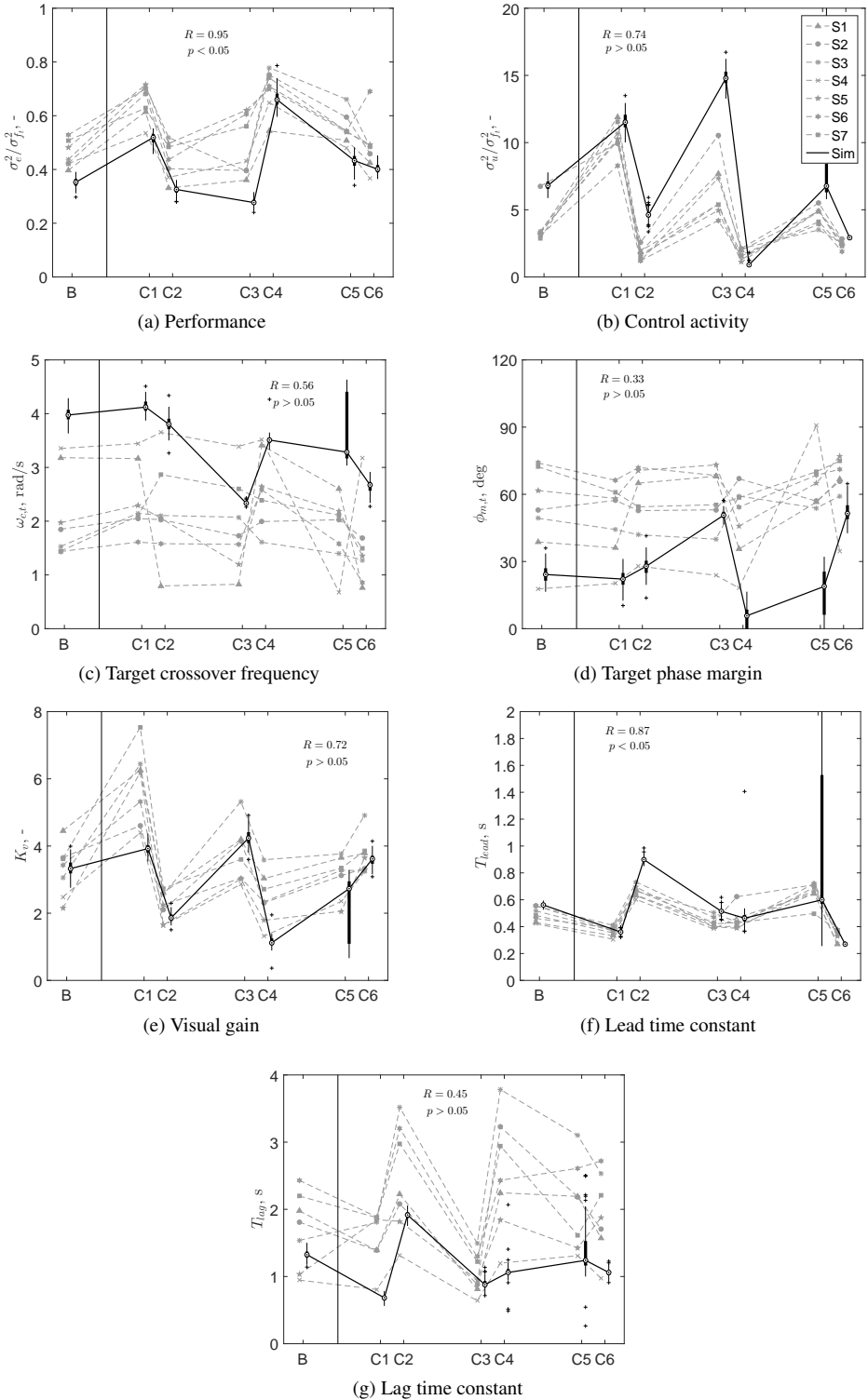
Figure A.1: Comparison between experiment and simulation results (in simulation \sigma_n^2 / \sigma_u^2 = 0.1 ).
