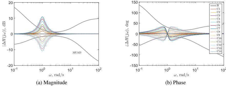
Figure 6.2: MUAD and all added dynamics.
