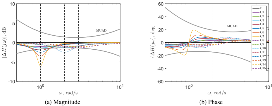
Figure D.2: The MUAD envelopes [4] and all added dynamics. The vertical dashed lines indicate the natural frequencies of the added dynamics (see Table D.1).
