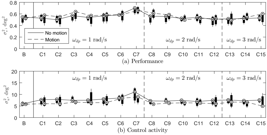
Figure D.4: Comparison of the performance and control activity between no-motion and motion cases.
