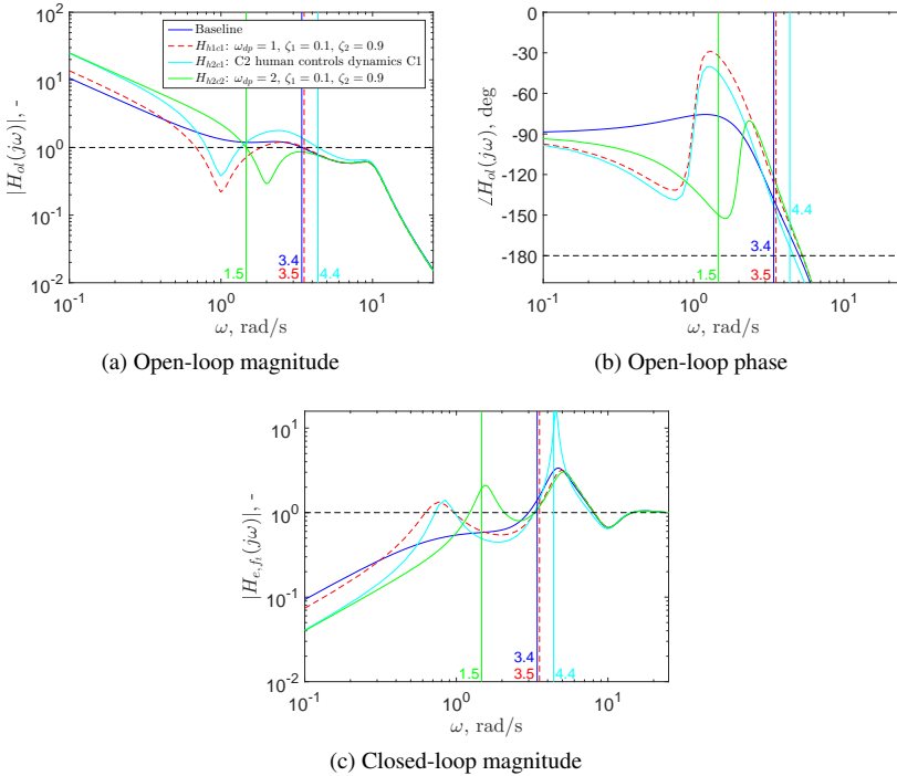
Figure 5.7: Open-loop and closed-loop analysis on baseline, down dipole ( \omega_{dp} = 1 rad/s, \zeta_1 = 0.1, \zeta_2 = 0.9 ), and down dipole ( \omega_{dp} = 2 rad/s, \zeta_1 = 0.1, \zeta_2 = 0.9 ) conditions.
