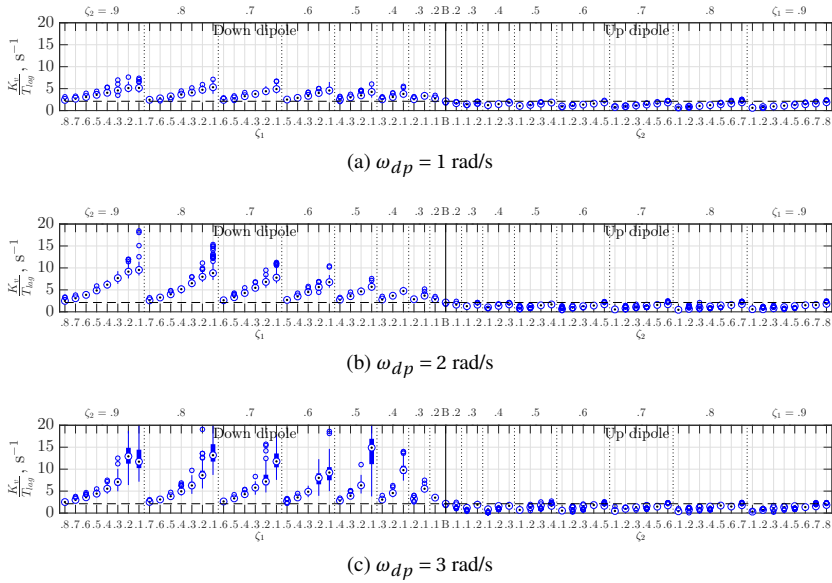
Figure 5.11: Ratio between visual gain and lag time constant at different \omega_{dp} .
