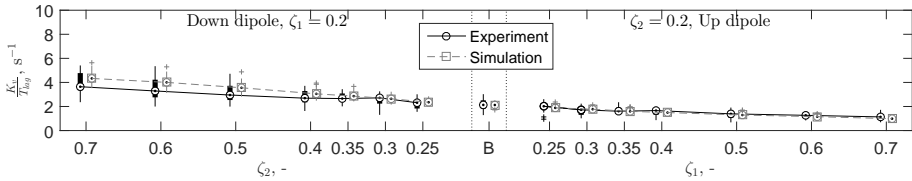
Figure 6.10: Comparison between experiment and simulation K_v/T_{lag} .
