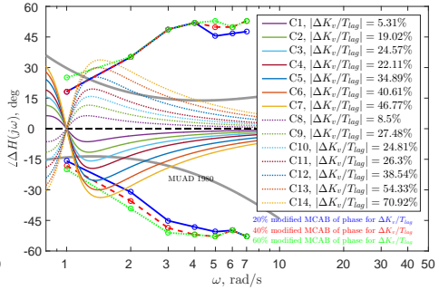
(f) Phase, \Delta K_v/T_{lag}
