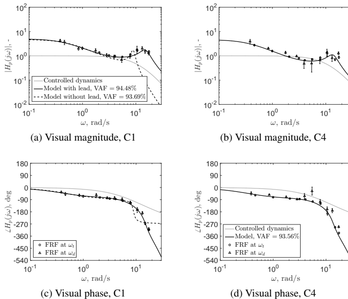
Figure 2.7: Example of human operator model fitting results for C1 and C4 (Subject 4).
