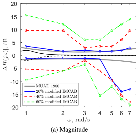
Figure 6.16: The modified IMCAB based on the intersection part of sub-figures in Figures 6.12a, 6.12d, 6.12e, 6.12h and Figure 6.15 for magnitude and phase, respectively. The added dipole dynamics of C1 and C8 (which are not significantly different from the baseline for the tracking performance, control activity, ratio of the visual gain and lag time constant and the lead time constant) are drawn for reference.
