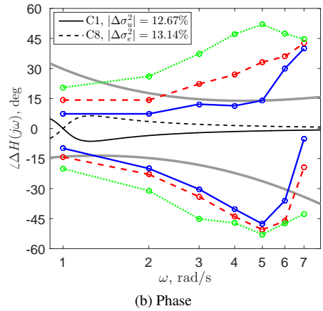
Figure 6.16: The modified IMCAB based on the intersection part of sub-figures in Figures 6.12a, 6.12d, 6.12e, 6.12h and Figure 6.15 for magnitude and phase, respectively. The added dipole dynamics of C1 and C8 (which are not significantly different from the baseline for the tracking performance, control activity, ratio of the visual gain and lag time constant and the lead time constant) are drawn for reference.
