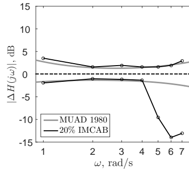
Figure 5.4: An example of the Integrated Manual Control Adaptation Boundary (IMCAB) of magnitude of 20%, based on all the solid points in Figure 5.3.
