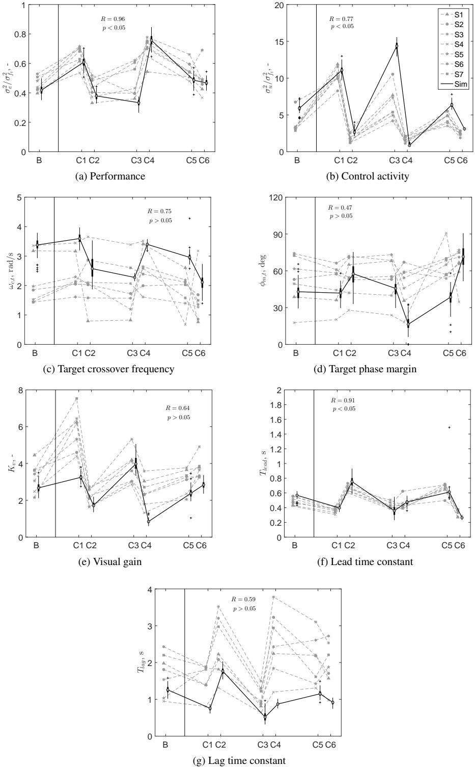
Figure 4.16: Comparison between experiment and simulation results (in simulation \sigma_n^2 / \sigma_u^2 = 0.25 ).
