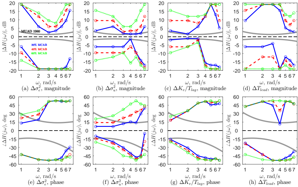
Figure 5.12: The Manual Control Adaptation Boundaries (MCAB) with various amounts of relative changes on the performance, control activity, ratio of the visual gain and lag time constant and lead time constant (blue: |\Delta| \leq 20\% , red: |\Delta| \leq 40\% , green: |\Delta| \leq 60\% ) compared with the original MUAD envelopes [1] (grey).
