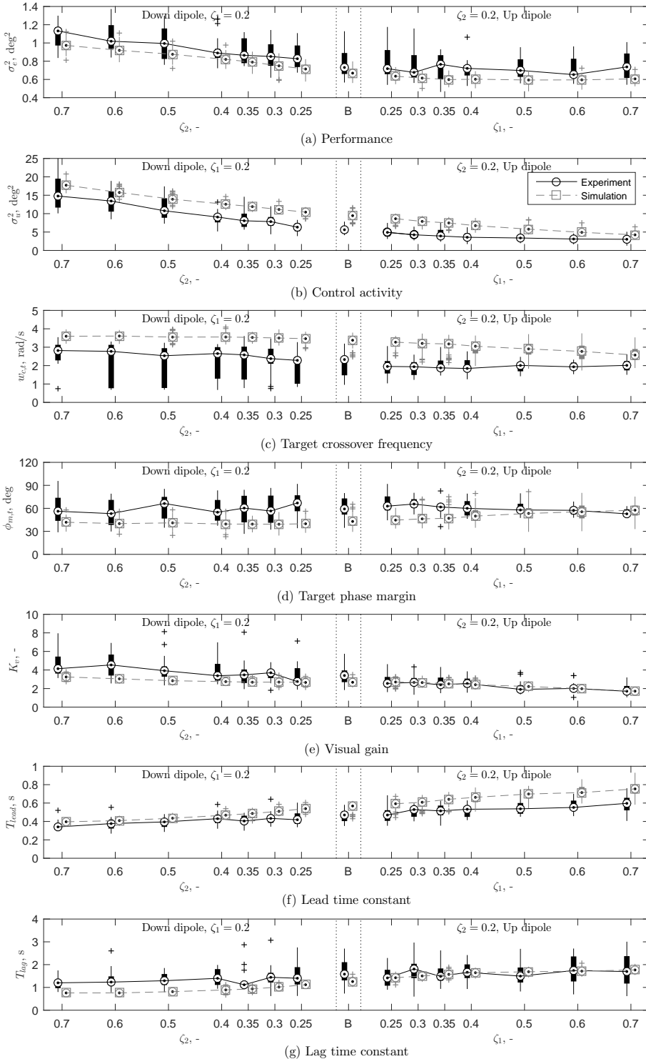
Figure 6.9: Comparison between experiment and simulation results.
