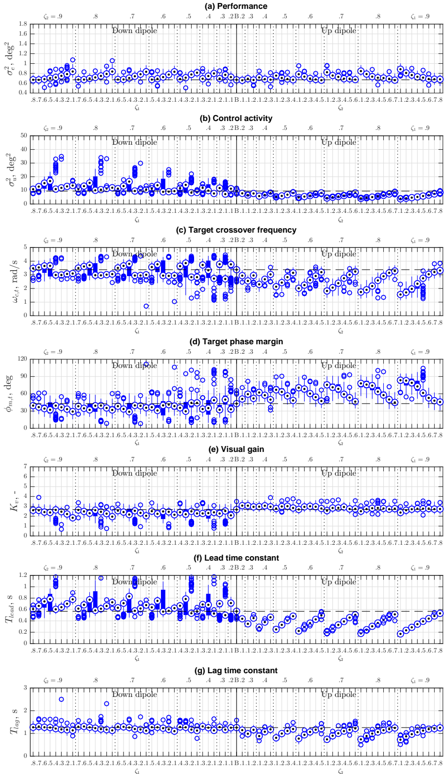
Figure C.4: All simulation results at \omega_{dp} = 7 \text{ rad/s} .
