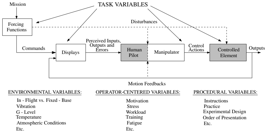
Figure 1.1: A schematic representation of a manual tracking task and the variables that affect a pilot-vehicle system. This figure is reproduced from [29], with adjustment to emphasize the relation between the human pilot and the controlled element, which is the main focus of this thesis.
