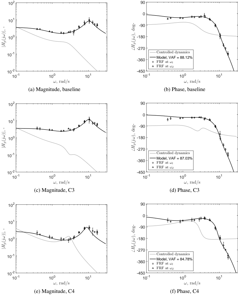
Figure 4.12: Subject 7 compensatory model fits and frequency response functions for conditions of baseline, C3 and C4.
