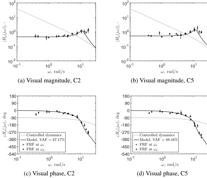
Figure 2.8: Example of human operator model fitting results for C2 and C5 (Subject 4).
