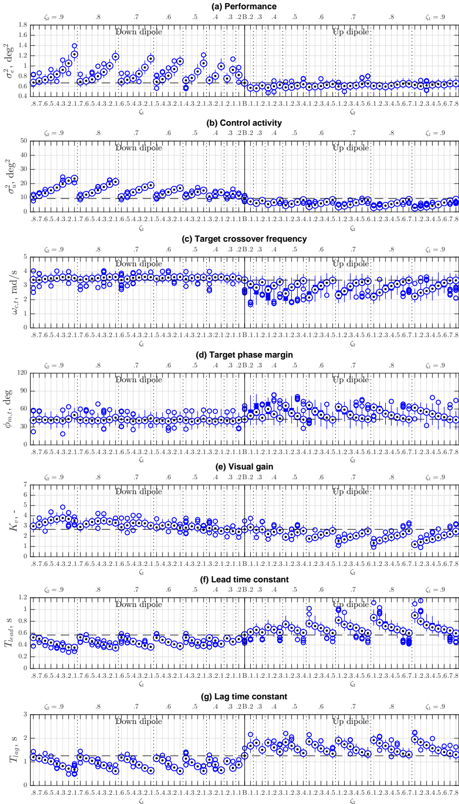
Figure 5.8: All simulation results at \omega_{dp} = 1 \text{ rad/s} .
