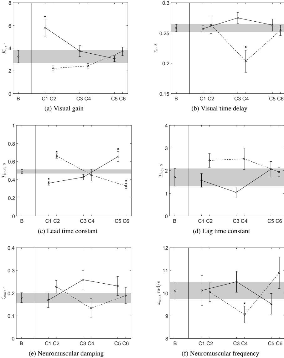
Figure 4.14: Human operator model parameters. The grey area marks the range of the baseline condition, and the asterisk marks the condition significantly different from the baseline condition.
