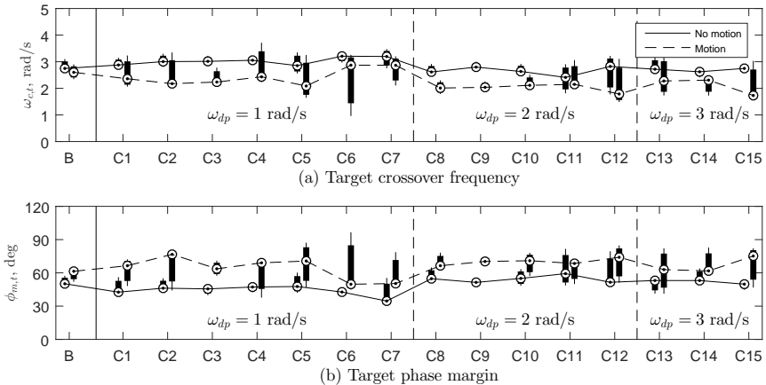
Figure D.5: Comparison of the target crossover frequencies and target phase margins between no-motion and motion cases.
