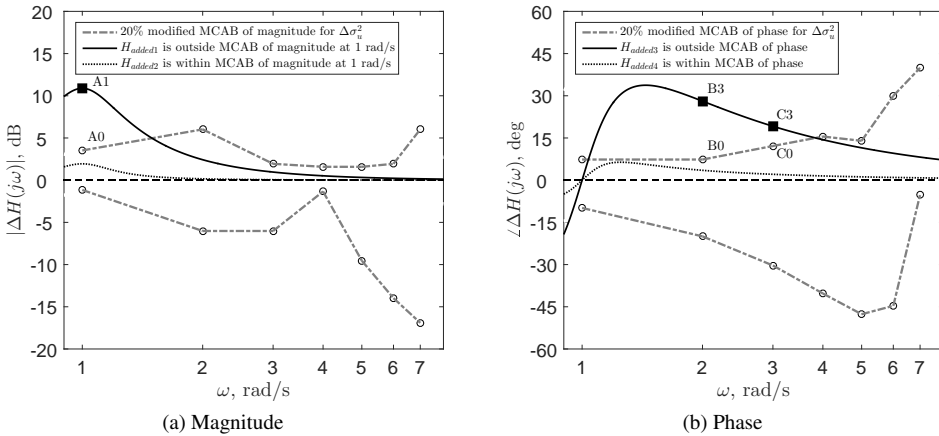
Figure 6.17: A demonstration showing the approach to verify the MCAB for \Delta\sigma_u^2 .
