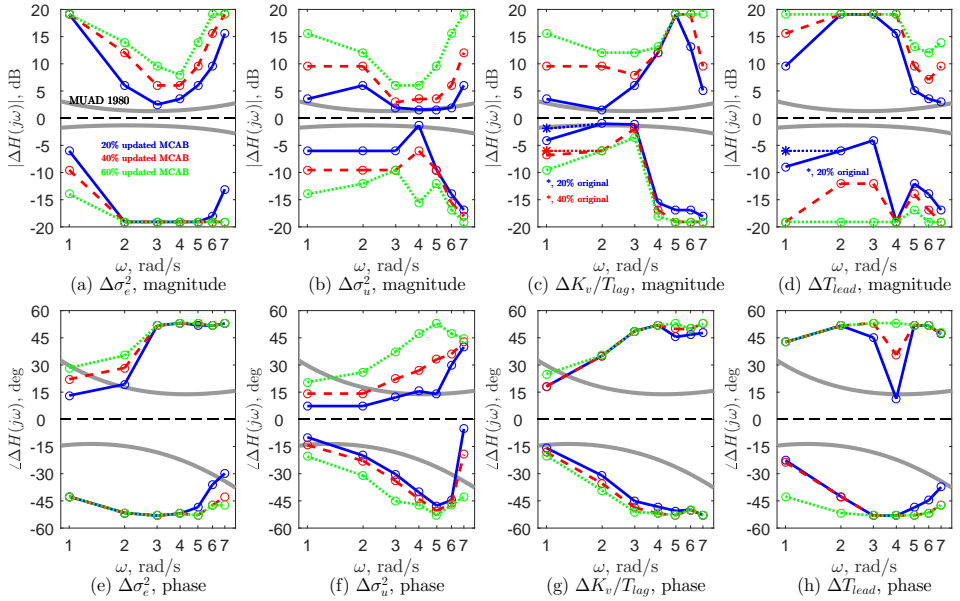
Figure 6.12: The updated simulation-based MCAB with various amounts of relative changes on the performance, control activity, ratio of the visual gain and lag time constant and lead time constant (blue: |\Delta| \leq 20\% , red: |\Delta| \leq 40\% , green: |\Delta| \leq 60\% ) compared with the original MUAD envelopes [2] (grey). Figure 6.12c and 6.12d also show the changes compared with the original simulation-based MCAB developed in Chapter 5.
