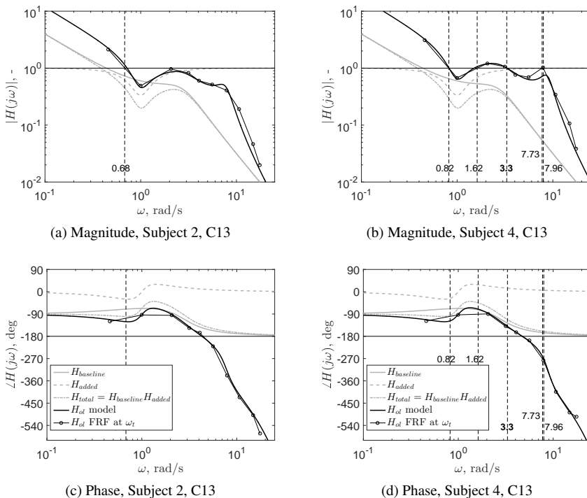
Figure E.1: Open-loop frequency responses of Subject 2 and Subject 4 in condition C13 (Chapter 6).
