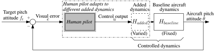
Figure 1.2: A schematic representation of the aircraft pitch attitude tracking tasks performed in Neal-Smith and Landing Approach High Order (LAHOS) System projects [69–71].
