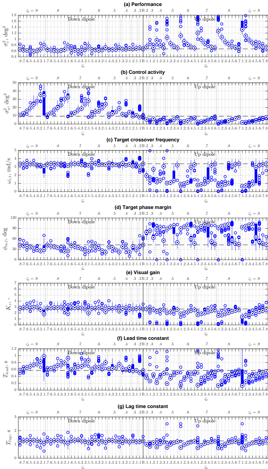
Figure C.2: All simulation results at \omega_{dp} = 5 \text{ rad/s} .
