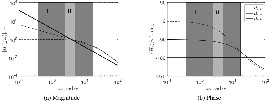
Figure 2.3: Bode of three different controlled elements. I: forcing function frequency range; II: crossover region for compensatory tracking.
