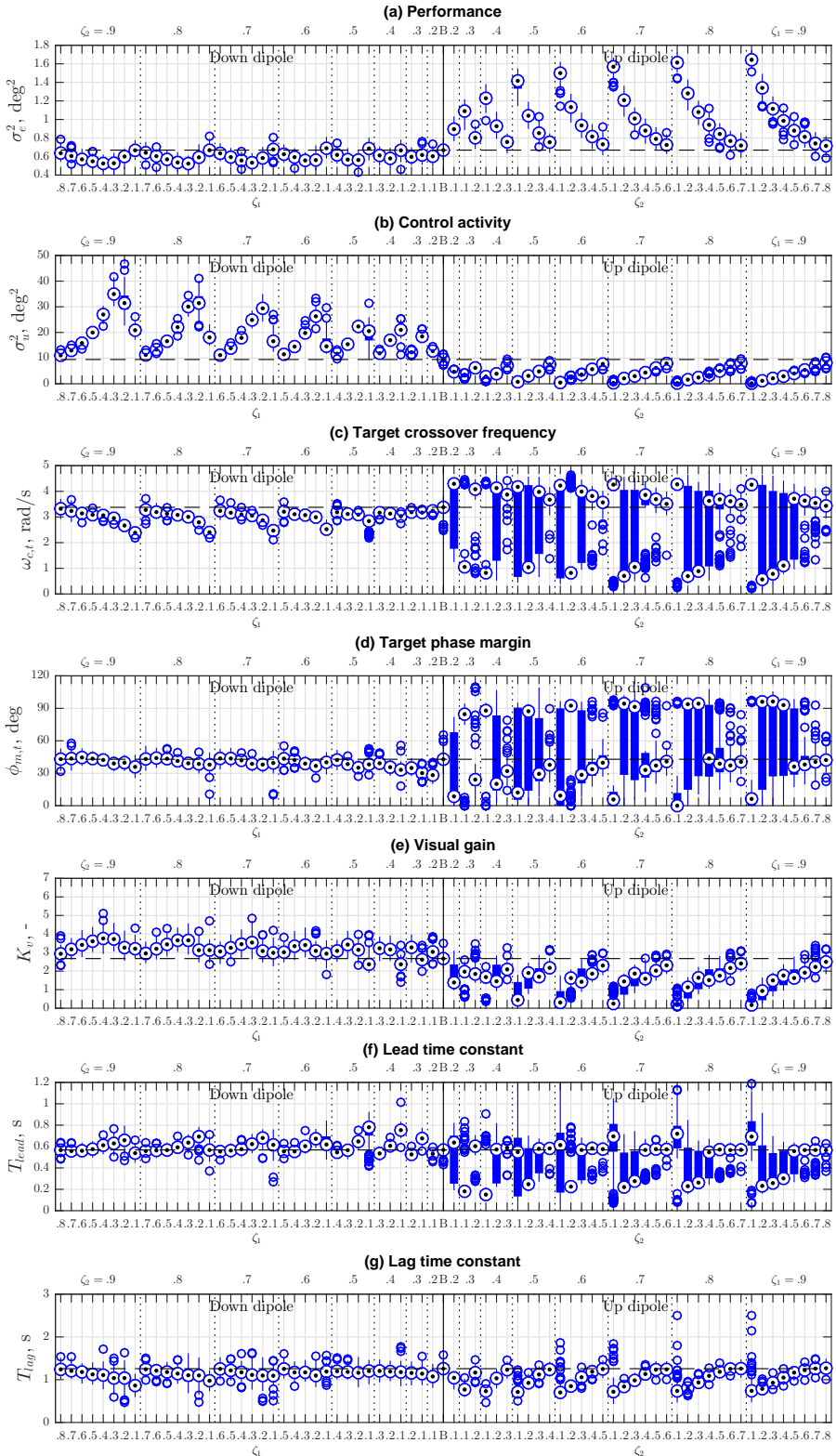
Figure C.1: All simulation results at \omega_{dp} = 4 \text{ rad/s} .
