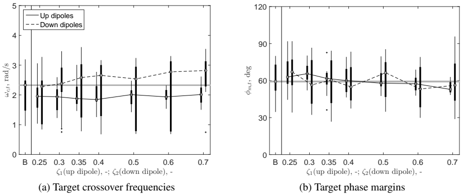
Figure 6.6: Target crossover frequencies and phase margins for each condition of fifteen subjects. Based on a Wilcoxon signed-rank test ( p < 0.0036 ), none of the condition is significantly different from the baseline for target crossover frequency or target phase margin, respectively.
