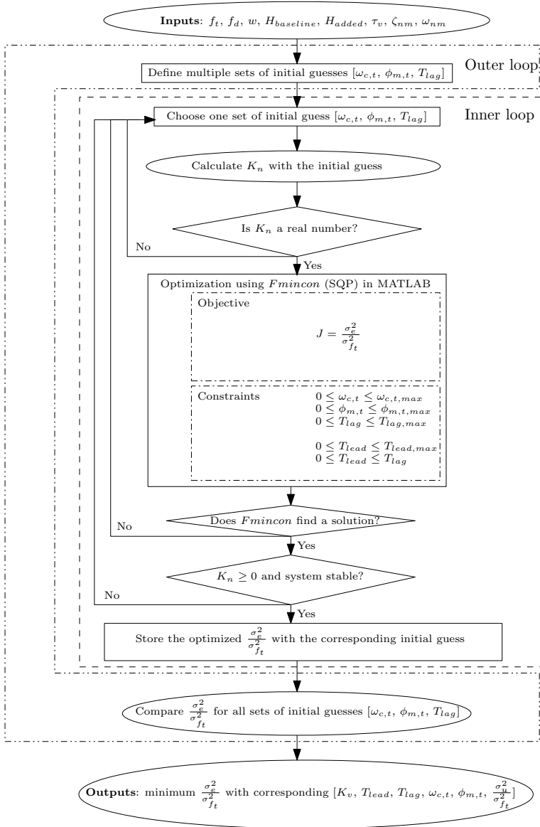
Figure 4.6: A representation of the simulation routine.
