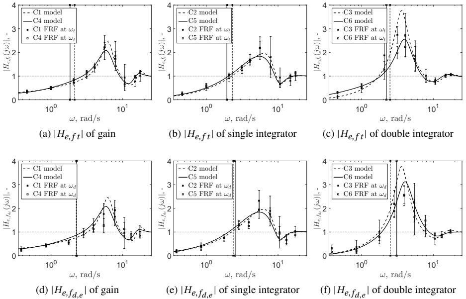
Figure 2.11: Frequency responses of target-to-error and disturbance-to-error dynamics.
