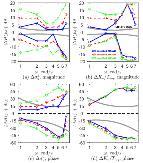
Figure 6.15: The modified MCAB for \Delta\sigma_u^2 and \Delta K_v/T_{lag} with experiment data corrections.
