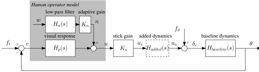
Figure 4.4: A schematic representation of the simulation remnant.
