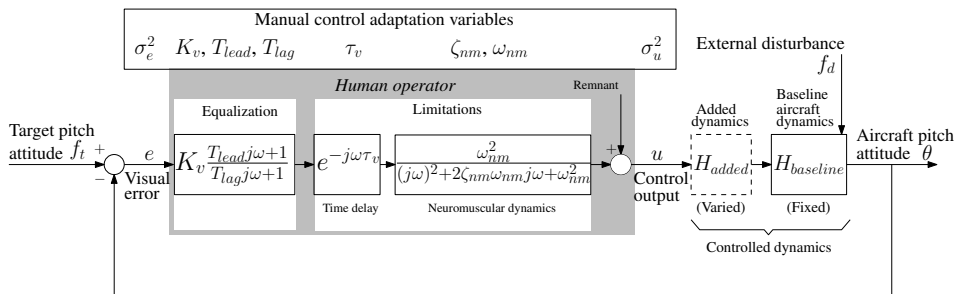
Figure 1.4: An example of the human operator model quantifying manual control behavior in a compensatory tracking task.
