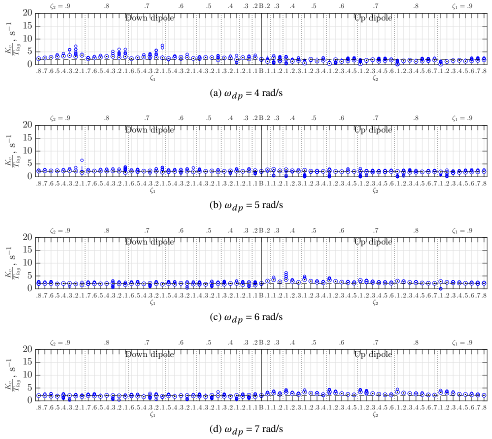
Figure C.5: Ratio between visual gain and lag time constant at different \omega_{dp} .
