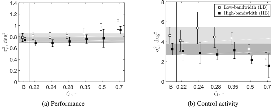
Figure 3.5: Variance of the error signal e and control signal u for each condition averaged over seven subjects.
