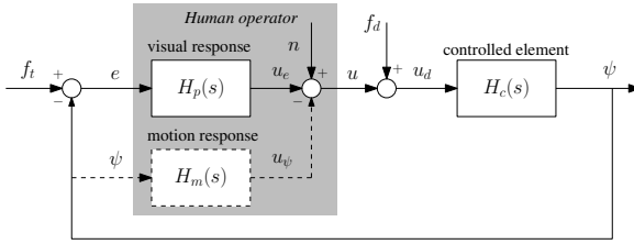
Figure 2.1: The closed-loop yaw attitude tracking task.
