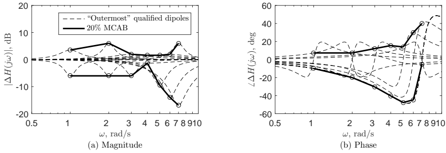
Figure 5.2: An example of formulating the Manual Control Adaptation Boundaries (MCAB) for control activity based on the “outermost” qualified dipole dynamics, of which -20\% \leq \Delta\sigma_u^2 \leq 20\% .
