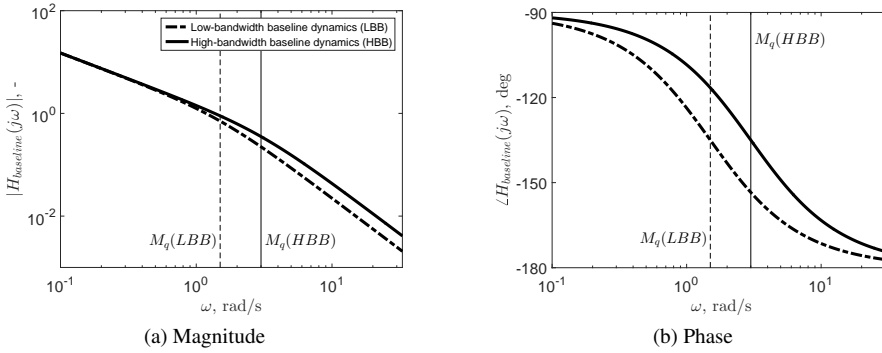
Figure 3.2: Frequency responses of low and high-bandwidth baseline dynamics.
