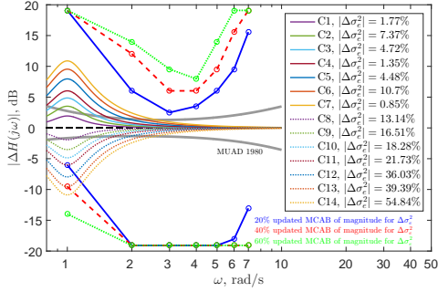
(a) Magnitude, \Delta\sigma_e^2
