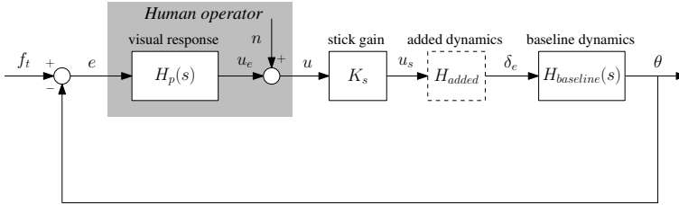
Figure 3.1: A schematic representation of the pitch attitude tracking task.
