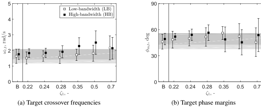
Figure 3.6: Target crossover frequencies and phase margins for each condition averaged over seven subjects.
