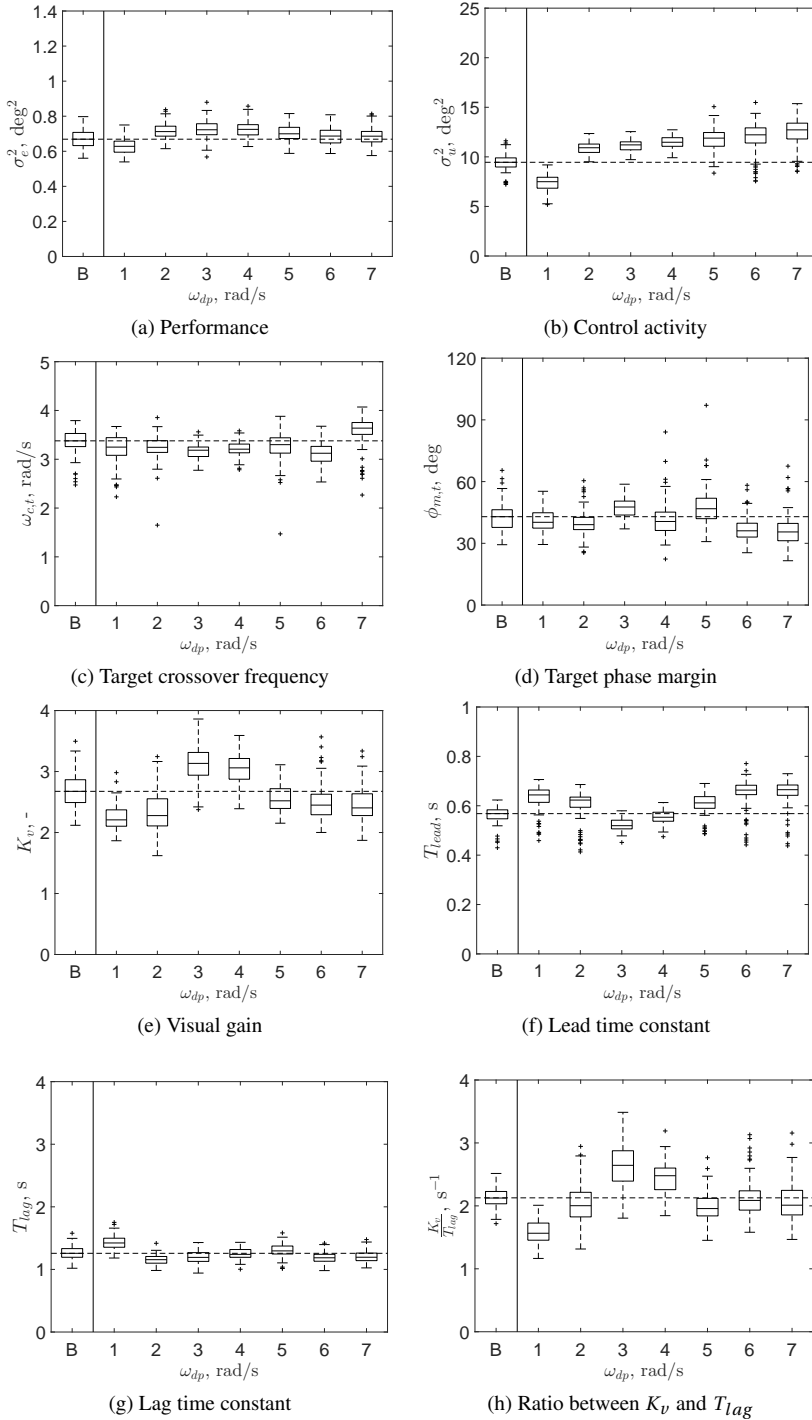
Figure 5.14: Human operator parameters of maximum deviations from baseline. All added dipole dynamics are within the MUAD envelopes (Figure 5.6).
