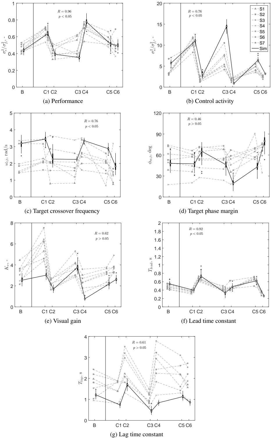
Figure A.5: Comparison between experiment and simulation results (in simulation \sigma_n^2 / \sigma_u^2 = 0.3 ).
