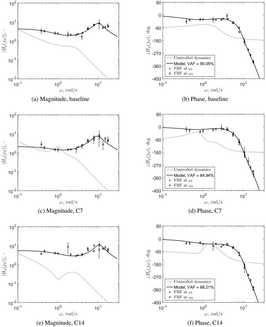
Figure 6.7: Subject 3 compensatory model fits and frequency response functions for conditions of baseline, C7 and C14.
