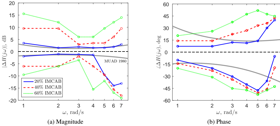
Figure 5.13: Integrated Manual Control Adaptation Boundaries (IMCAB) with different levels of relative changes on performance, control activity or control behavior. (blue: |\Delta| \leq 20\% , red: |\Delta| \leq 40\% , green: |\Delta| \leq 60\% ) compared with the original MUAD envelopes [1] (grey).
