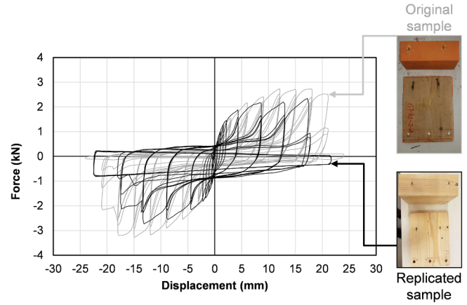
Fig. 8. Comparison between the hysteretic cycles of original and replicated plank-joist connections.
