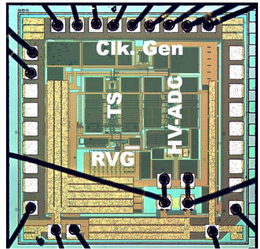
Fig. 7. Chip photograph.
