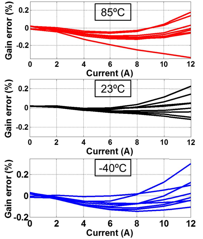
Fig. 11. Current sensing gain error with hybrid TCS.
