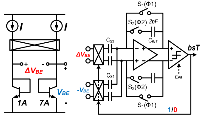
Fig. 6. Schematic of the RVG (left) and the TS (right).
