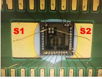
Fig. 3. Bonding diagram of the chip.
