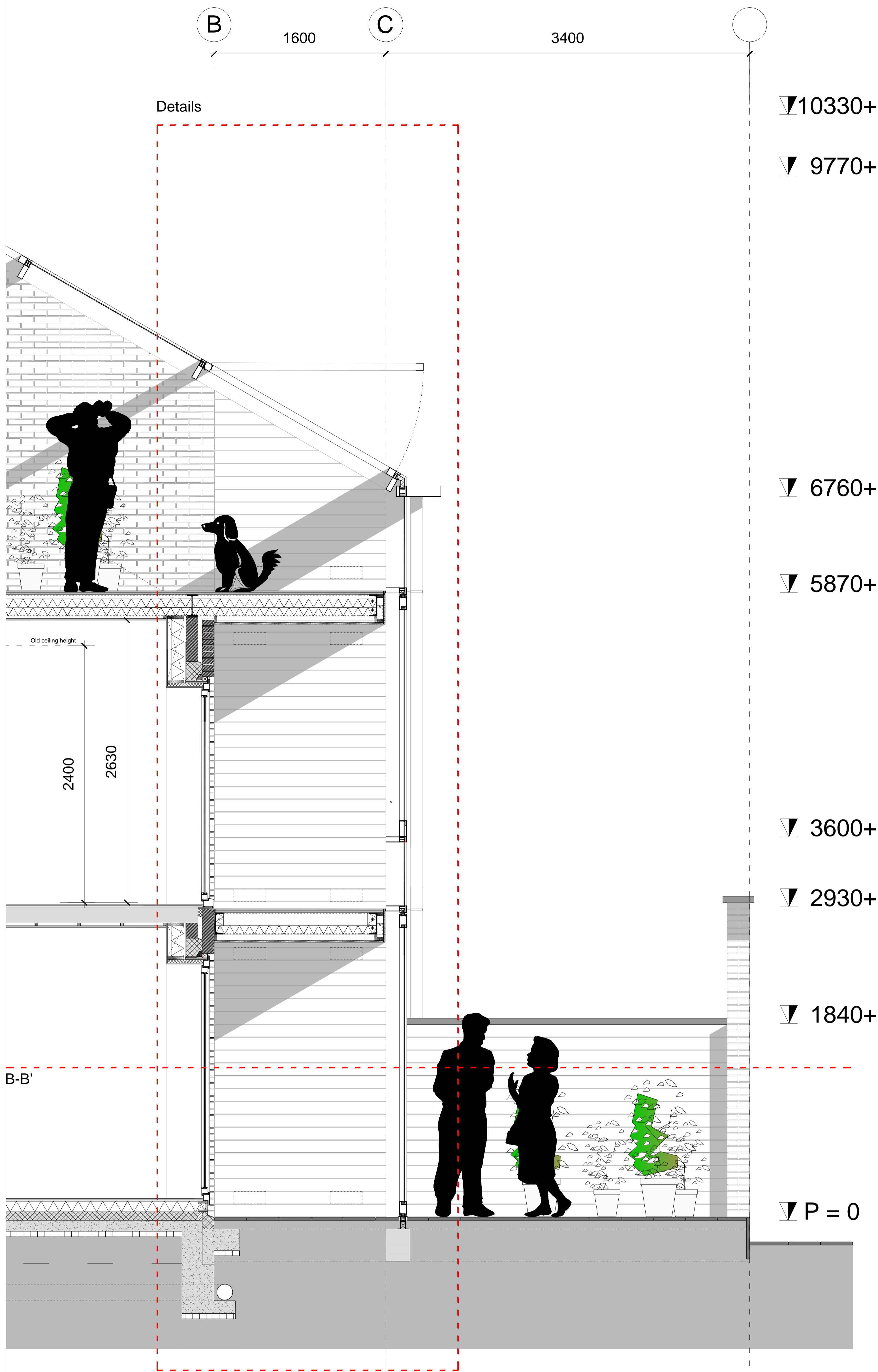
Section fragment A-A'
