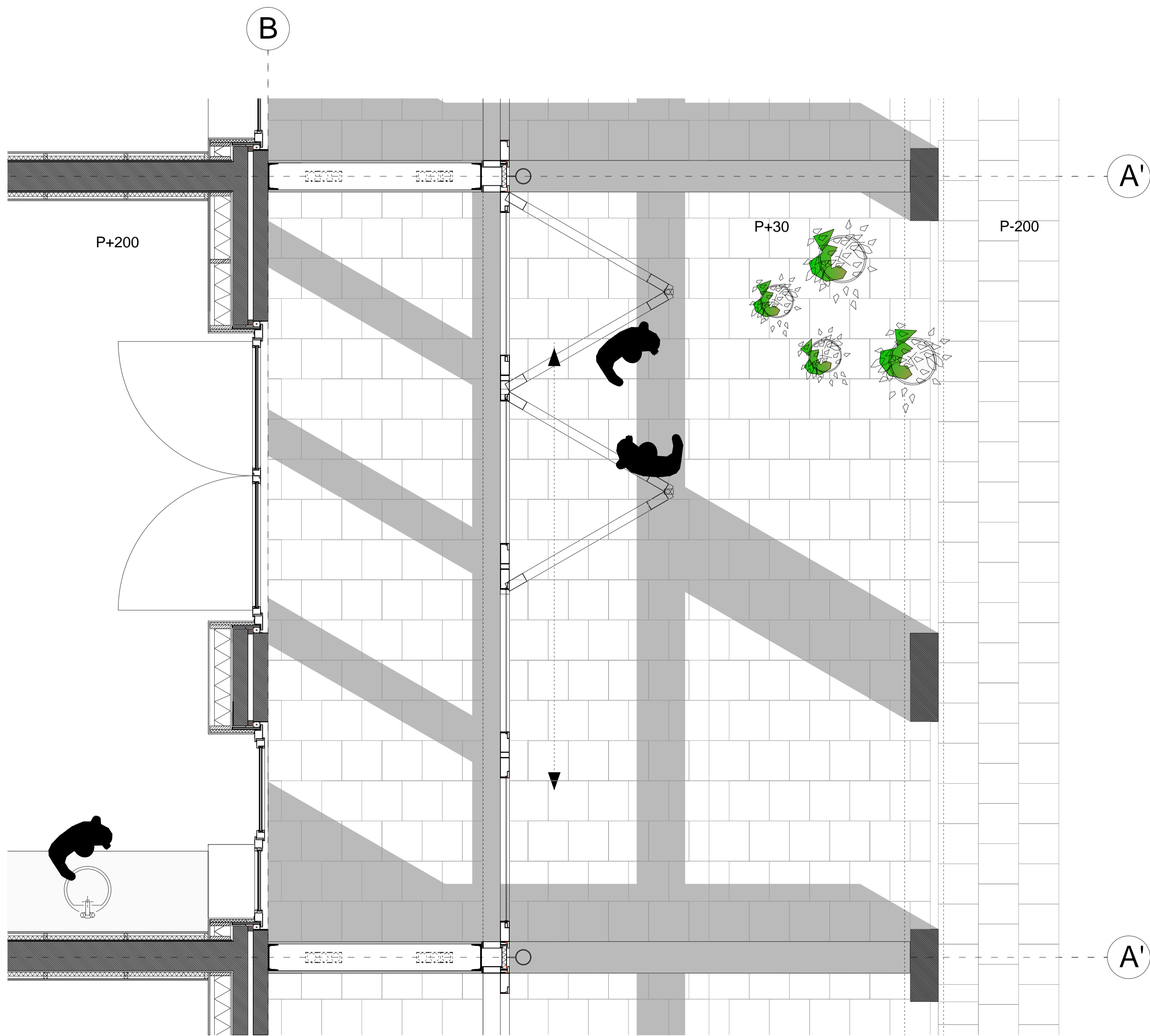
Groundfloor fragment B-B'
