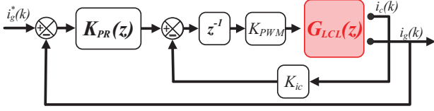
Fig. 6: Block diagram of the control structure in Figure 1
