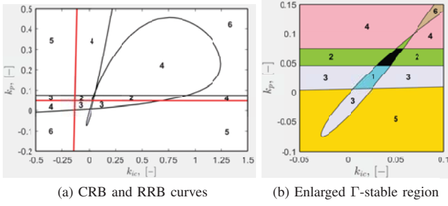
Fig. 3: Root invariant regions for L_g = 0 , R_g = 0
