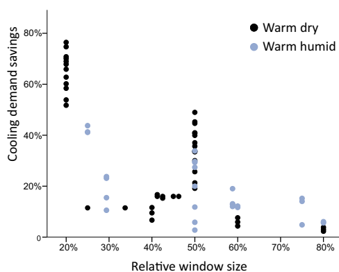
FIGURE 6.7 Cooling demand savings compared to relative window size
