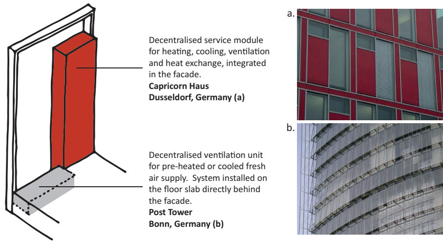
FIGURE 4.1 Integrated façades: Capricorn Haus, Düsseldorf (a) and Post Tower, Bonn (b). Pictures from the author
