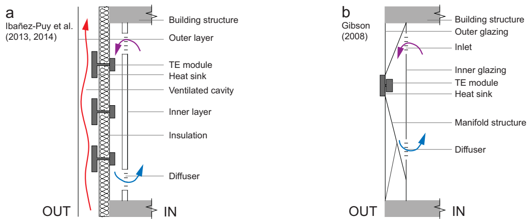
FIGURE 3.9 Air-based thermoelectric facades. Schemes based on Ibanez-Puy et al. (2013, 2014) and Gibson (2008).
