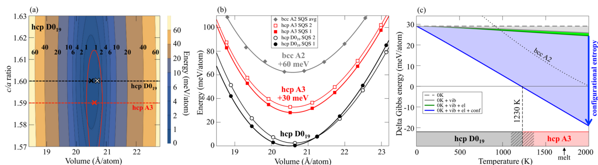
Figure 4. Ab initio energetics of the hcp based phases D0 19 and A3, and of the bcc based A2 phase for the Al 15 Hf 25 Sc 10 Ti 25 Zr 25 at.% HEA. (a) Energy contour plot at T = 0 K for the D0 19 phase as a function of volume and c/a ratio. The bold black numbers give the value of the contours in meV/atom. The black dashed line indicates the equilibrium c/a ratio (of SQS 1) and the black and white crosses mark the equilibrium volumes of the two employed supercells (SQS 1 and 2). The red solid line shows the 1 meV/atom contour of the hcp A3 energy surface. The red dashed line indicates the equilibrium c/a ratio for hcp A3 and the red cross the corresponding equilibrium volume. (b) T = 0 K energy-volume curves for D0 19 and A3 (with two SQS' for each phase) at the equilibrium c/a ratios as indicated by the dashed lines in (a). The energy-volume curve of bcc A2 which has been obtained by an average over the two studied SQS supercells (see the Methods section on the ab initio energetics) is also shown. (c) Difference in the Gibbs energies of D0 19 and A3 as a function of temperature (D0 19 corresponding to the zero line). The Gibbs energy difference is decomposed into the T = 0 K energy (0 K), the vibrational (vib), electronic (el), and configurational (conf) contribution. The final curve corresponds to the blue solid line, resulting in a transition temperature of 1230 K as indicated by the vertical dashed line. The dotted line shows the difference between the Gibbs energy of D0 19 and bcc A2 containing all contributions. The onset of melting as obtained from our experimental results is indicated by the black arrow.
