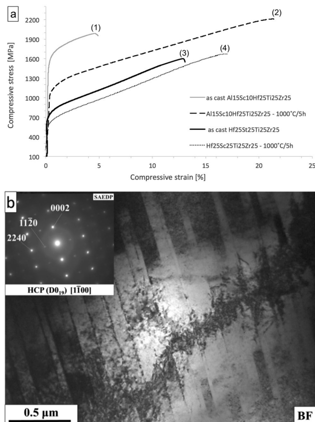
Figure 9. (a) Compression curves of the Al 15 Hf 25 Sc 10 Ti 25 Zr 25 at.% alloy in the as cast state (curve 1) and annealed state at 1000 °C for 5 h (curve 2), and of Hf 25 Sc 25 Ti 25 Zr 25 at.% in the as cast (curve 3) and annealed (curve 4) state. (b) TEM bright field image with SAED pattern of the annealed Al 15 Hf 25 Sc 10 Ti 25 Zr 25 at.% HEA after compression to 22% strain.
