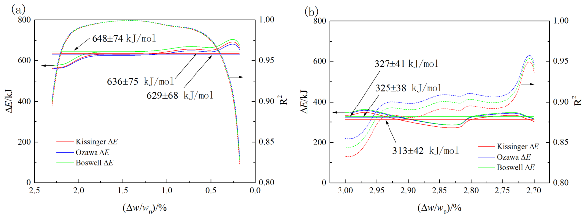
Fig. 8. Activation energy of thermal decomposition reaction: (a) 1st stage; (b) 2nd stage, which are before and after 1320^\circ\text{C} . (Online version in color.)
