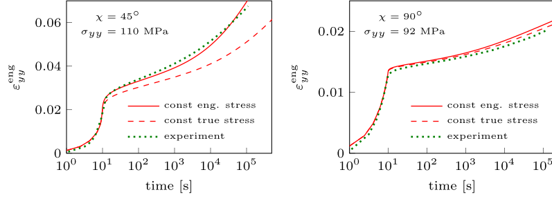
Fig. 13. Comparison of experimental results with simulations assuming constant engineering stress and constant true stress on the material, for two off-axis angles and T = 25 °C.
