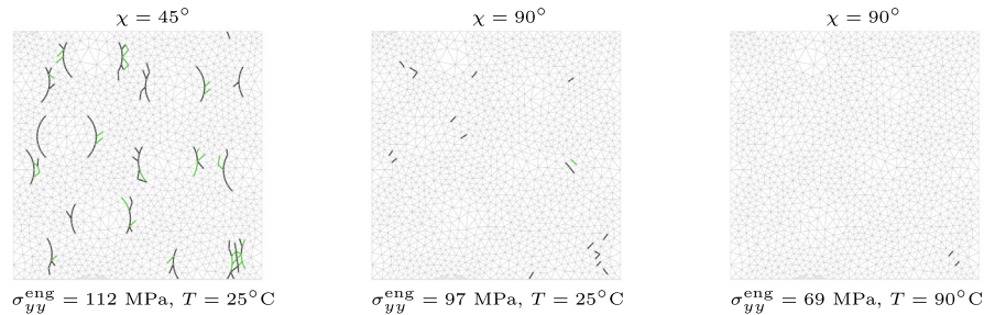
Fig. 19. Black lines representing degrading cohesive elements at the moment of minimum creep strain-rate in the RVE, which coincides with defined rupture time; green lines indicate unloading cohesive segments, whereas gray lines represent finite element mesh.
