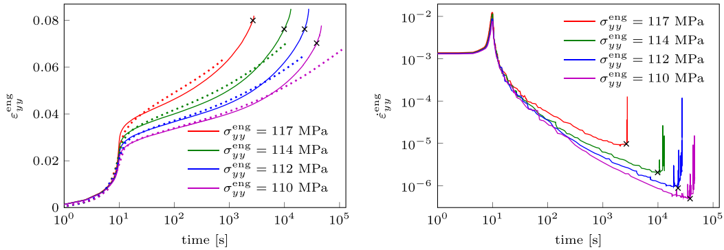
Fig. 15. Evolution of homogenized strain for \chi = 45^\circ and T = 25 °C (left); change in homogenized strain-rate with time (right); solid lines: model response, markers: model creep rupture points, dotted lines: experiment.
