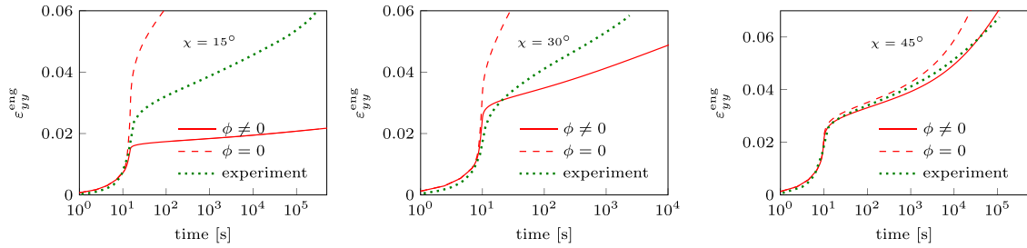
Fig. 21. Creep response of rotating RVE ( \phi \neq 0 ) and non-rotating RVE ( \phi = 0 ) compared with experiments for T = 25^\circ\text{C} and three off-axis angles: 15^\circ (290 MPa), 30^\circ (154 MPa) and 45^\circ (110 MPa); creep stress for \chi = 15^\circ reached at t = 15 s.
