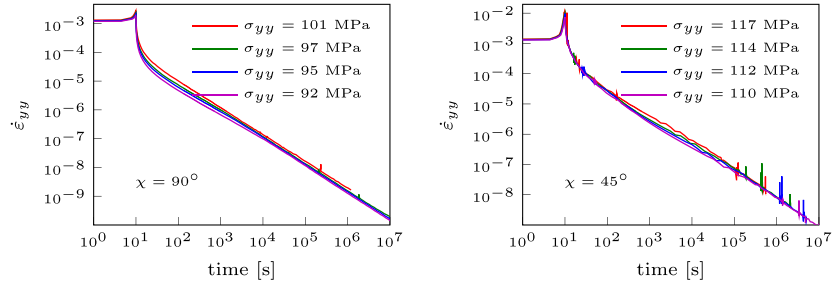
Fig. 12. Homogenized strain-rate versus time for T = 25 °C, different off-axis angles and stress levels, with time-independent cohesive law governing decohesion process.
