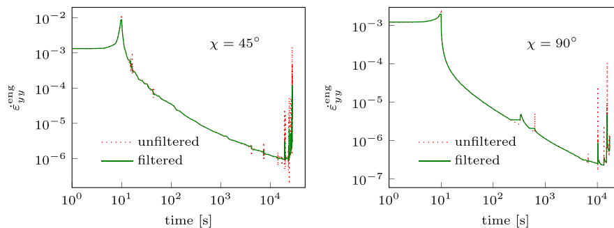
Fig. B.24. Unfiltered versus (median) filtered homogenized strain-rate curves for \chi = 45^\circ and \sigma_{yy}^{eng} = 112 MPa (left), and \chi = 90^\circ and \sigma_{yy}^{eng} = 95 MPa (right).
