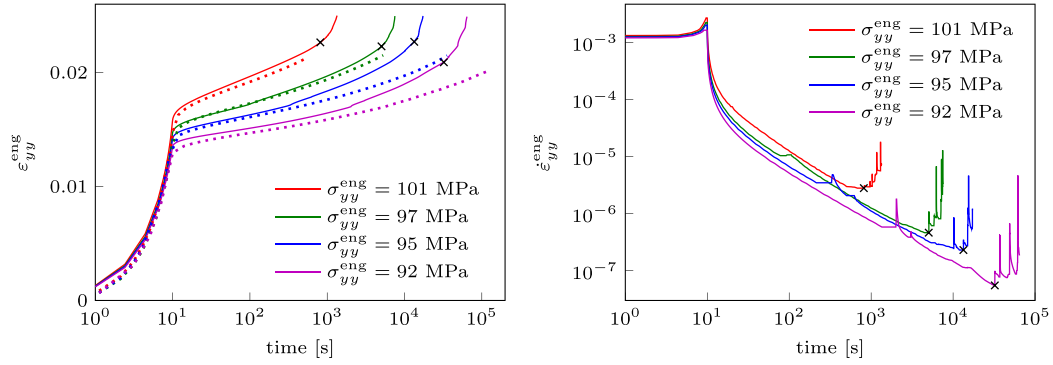
Fig. 14. Evolution of homogenized strain for \chi = 90^\circ and T = 25 °C (left); evolution of homogenized strain-rate (right); solid lines: model response, markers: model creep rupture points, dotted lines: experiment.
