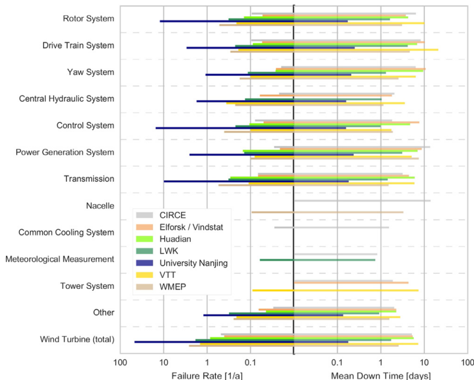
Fig. 3 Failure rates (failure per WT per year) and mean downtimes (weighted according to their occurrences) per failure of onshore WTs according to seven (7) publicly available databases (Pfaffel et al., 2017). From Pfaffel S, Faulstich S, and Rohrig K (2017) Performance and reliability of wind turbines: A review. Energies 10(11): 1904.
