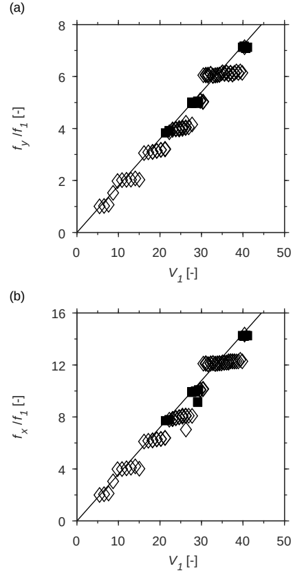
Fig. 8: Normalised (a) cross-flow and (b) in-line dominant frequencies ( f_{x,y}/f_1 ) versus V_1 . In (a), the straight line represents the frequency corresponding to a Struhall number 0.17; and in (b), the straight line represents the doubled frequency corresponding to a Struhall number 0.17.
