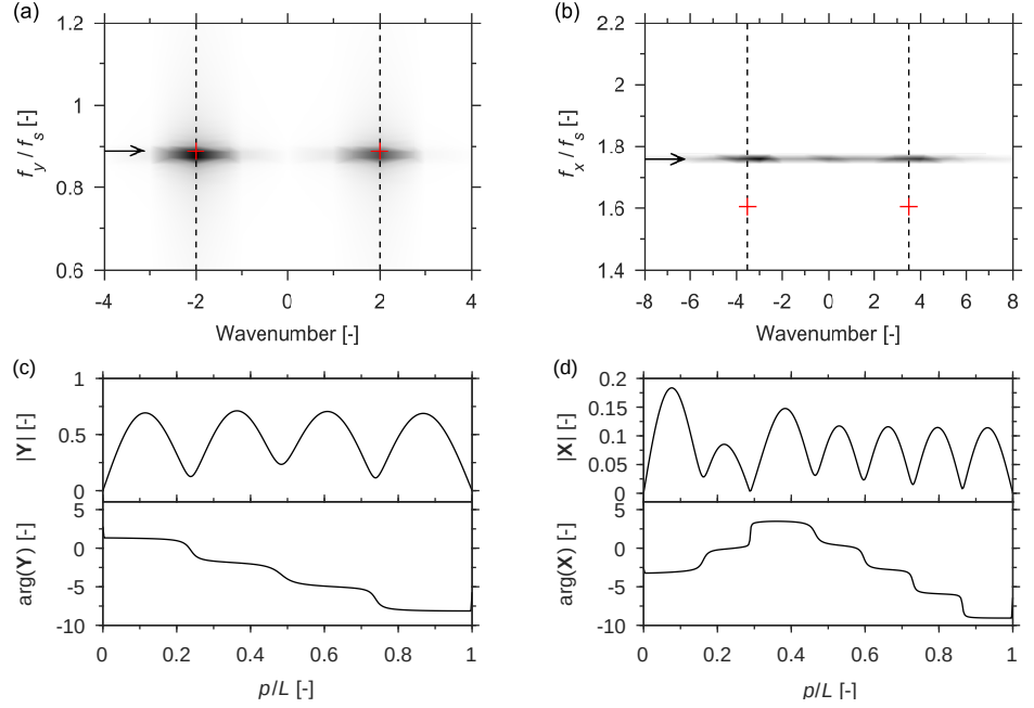
Fig. 11: Spatio-temporal spectra of (a) cross-flow and (b) in-line displacements at flow velocity V = 0.5 m/s with (c) cross-flow and (d) in-line complex modes extracted at dominant frequencies which are indicated by arrows. The wavenumbers and natural frequencies of selected free vibration modes are indicated by black vertical dashed lines and red crosses respectively.
