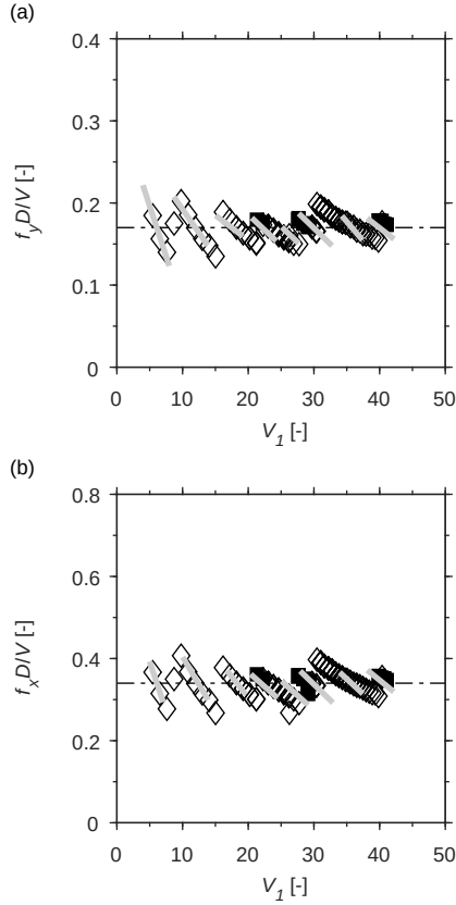
Fig. 7: Normalised (a) cross-flow and (b) in-line dominant frequencies ( f_{x,y}D/V ) versus V_1 . In (a), the straight line represents the frequency corresponding to a Struhall number 0.17; and in (b), the straight line represents the doubled frequency corresponding to a Struhall number 0.17. Linear approximation of the experimental results by [37] are represented by grey thick lines.
