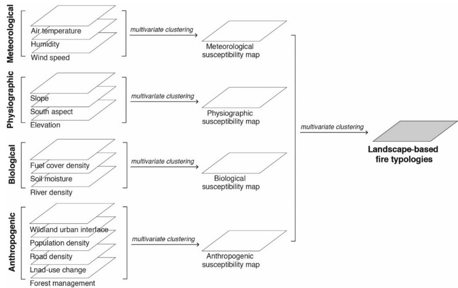
Fig. 2. GIS-base methodology
