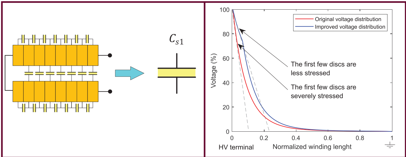
Figure 4. Equivalent capacitance model of a discs pair.
