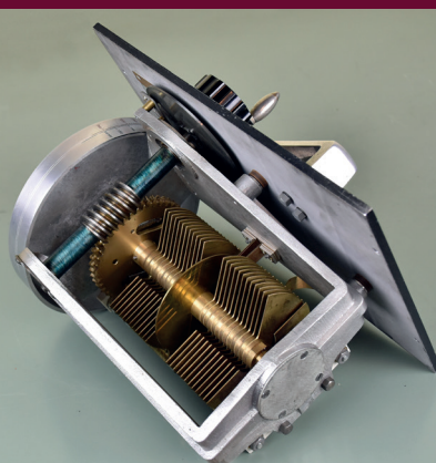
Figure 6. Variable precision capacitor (internal view)
