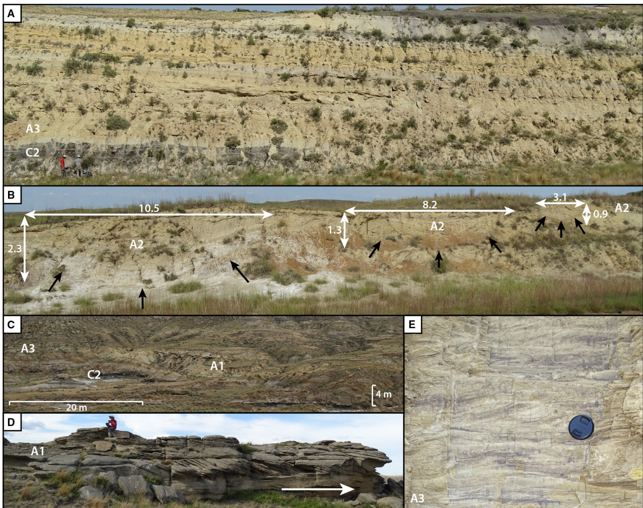
Fig. 4. Field photographs of Facies Association A – Channel-splay. (A) Facies A3. Greyish-yellow crevasse-splay sandstones and mudstones resting on top of a coal seam in the upper part of the RT-M section. Indurated elongated sandstone ribbons in the middle representing crevasse-splay channel fills. Laterally discontinuous whitish layer at top reflects weak soil leaching in between splays. Persons for scale are ca 1.8 m tall. (B) Facies A2. Low-angle diagonal stacking of concentric small-sized channel sandstone fills. Average width-depth ratios ca 4.8. West-side of Highway 24, ca 500 m south of the RT-M section. (C) Facies A1. Yellow, indurated channel sandstone belonging in the lower part of the RP-SW section. The sandstone is ca 7 m thick on the right and thins to the left and passes laterally into splay deposits of Facies A3. (D) Facies A1. Trough-cross-stratified channel sandstone in the top of the RP-SW section. Arrow indicates palaeo-flow to (E). (E) Facies A3. Ripple cross-laminations marked by black organic matter in sandy mudstone splays. Lens cap for scale is 5.7 cm in diameter.
